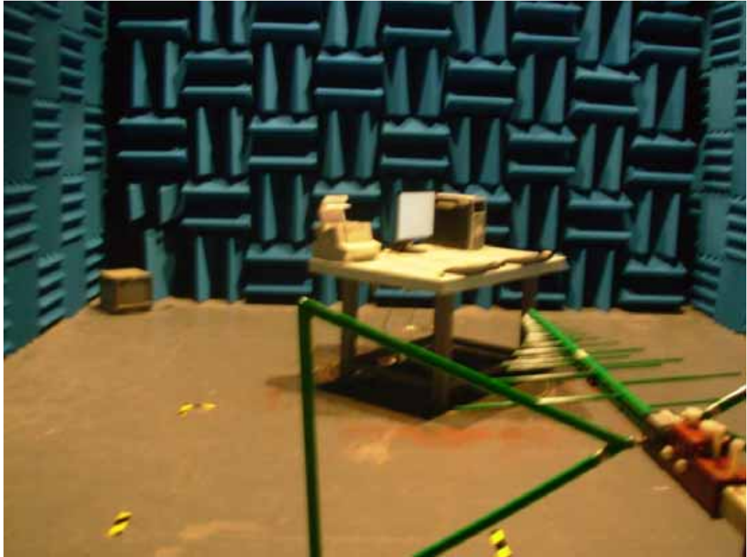
SETUP WITH MAXIMUM DETECTED EMISSION AT HORIZONTAL POLARIZATION (X-PORT 1440*900@60Hz)
