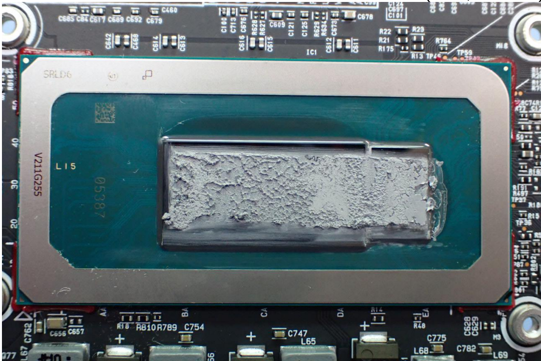
Figure 17 Internal View (CPU, i7-1260P)
