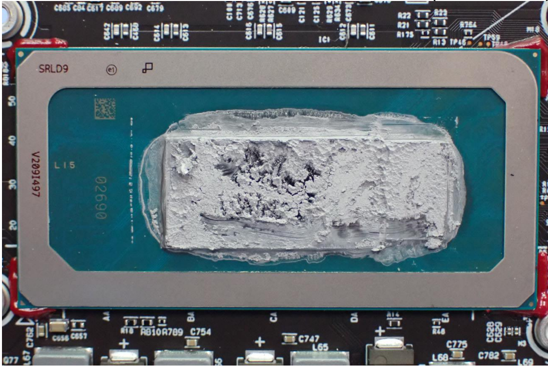
Figure 18 Internal View (CPU, i5-1240P)
