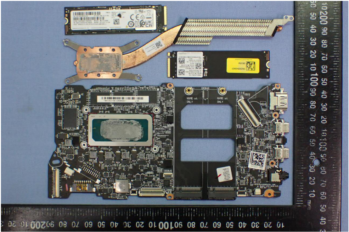
Figure 16 Internal View
