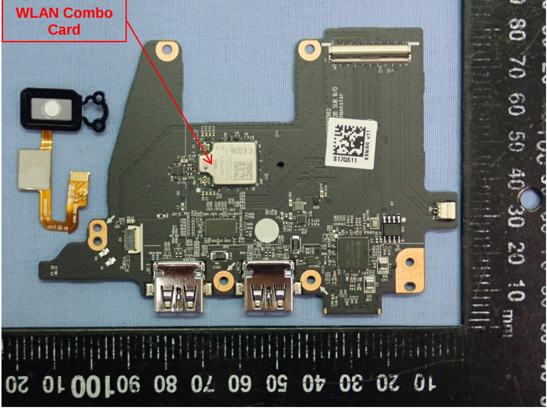
Figure 21 Internal View (WLAN SUB Bard, WLAN Combo CARD)
