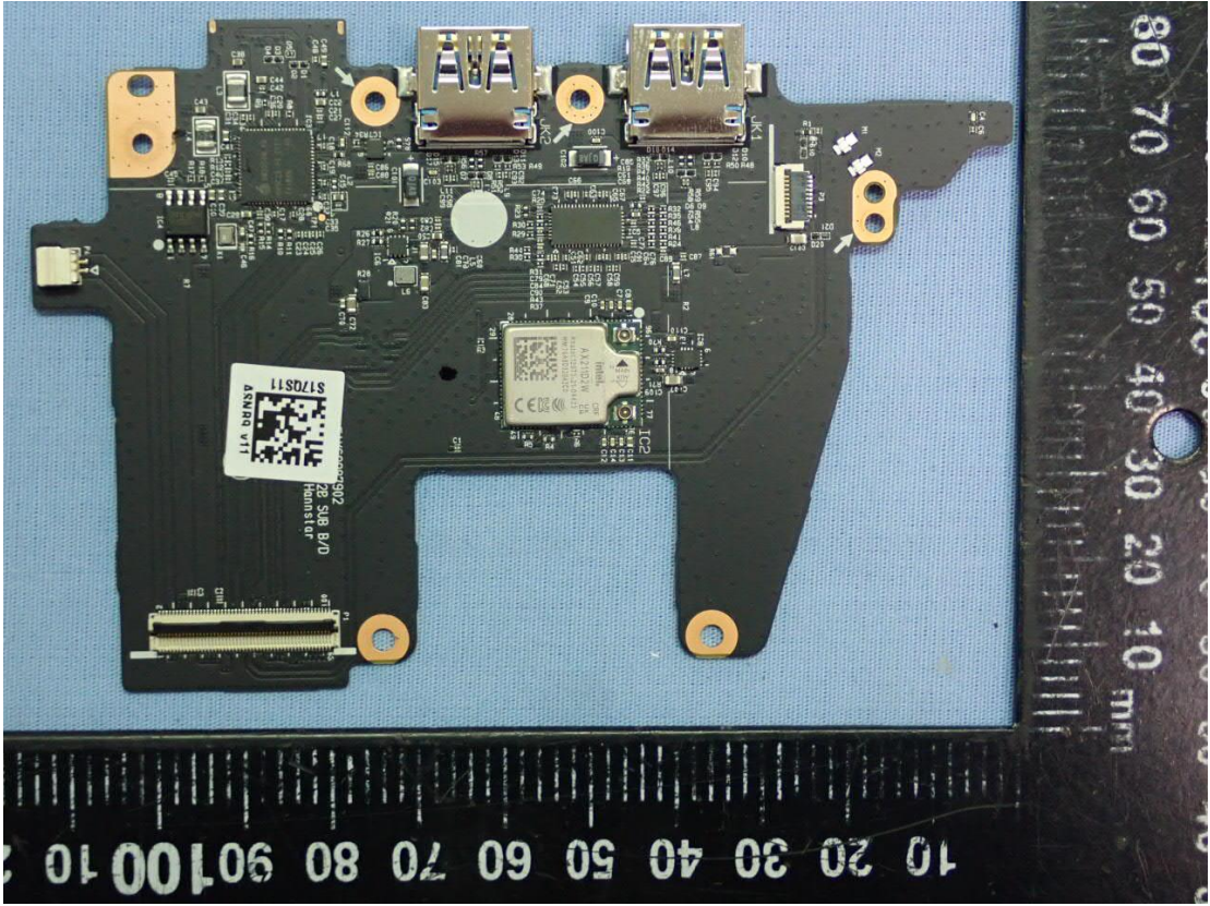
Figure 23 SUB Board, Front View
