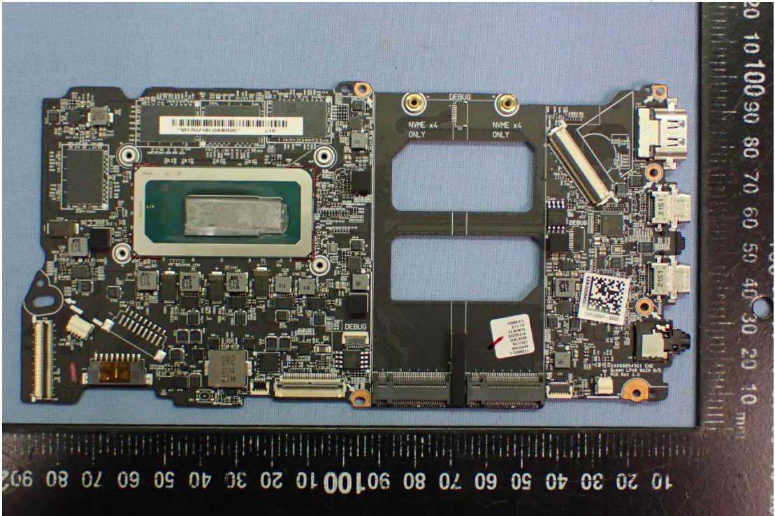
Figure 19 Main Board, Front View
