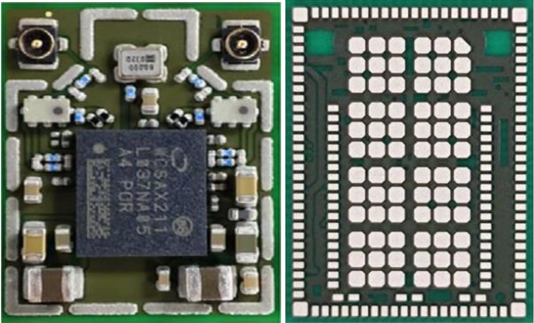
Figure 26 WLAN Combo Card, Without Shield and Back View
