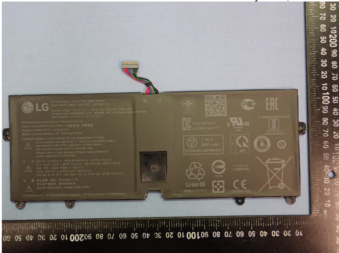
Figure 12 Battery Pack, Back View
