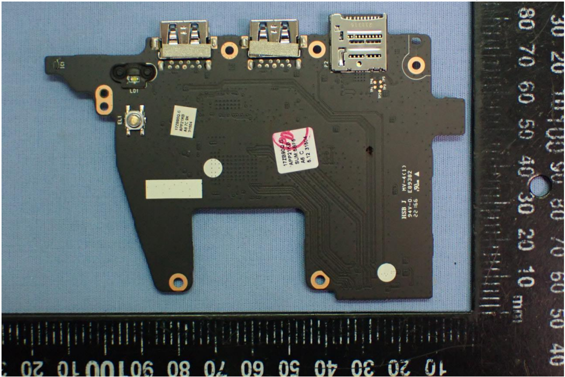
Figure 24 SUB Board, Back View
