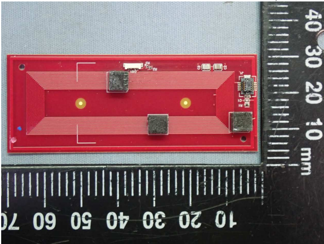
Figure 33 RFID Antenna, Front View
