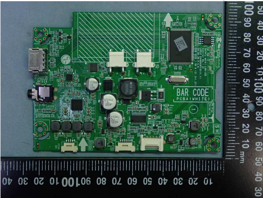
Figure 14 Control Board, Front View
