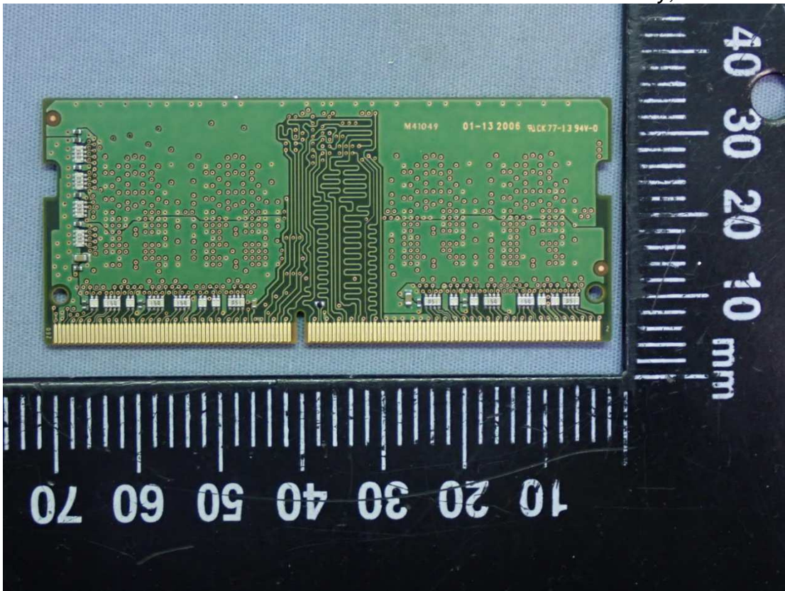
Figure 17 Memory, Back View
