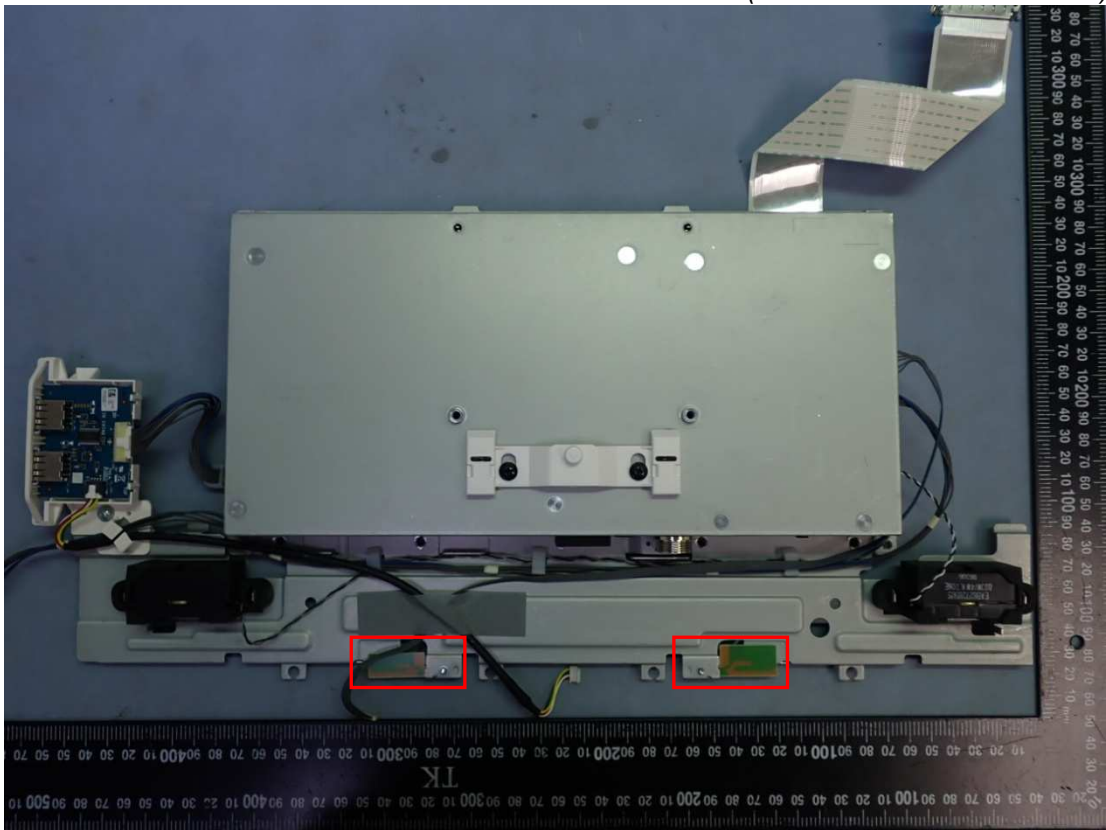
Figure 22 Internal View (WLAN Antenna Position)
