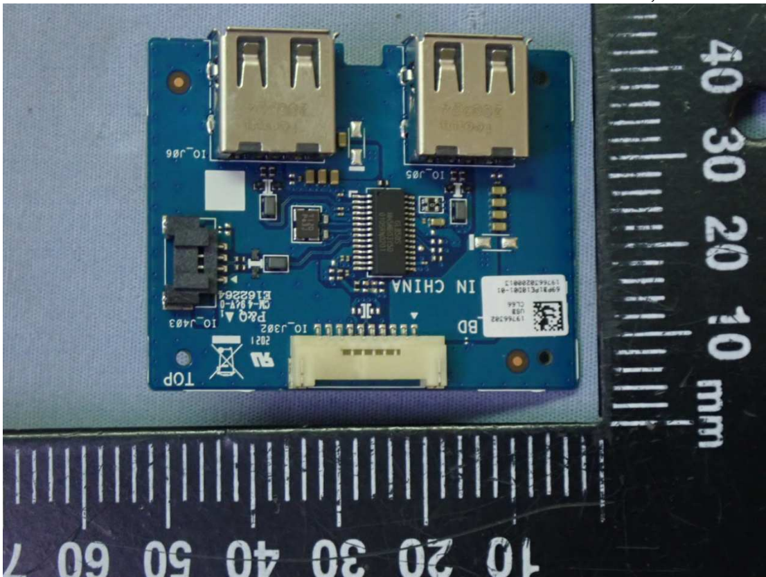
Figure 25 USB Control Board, Front View
