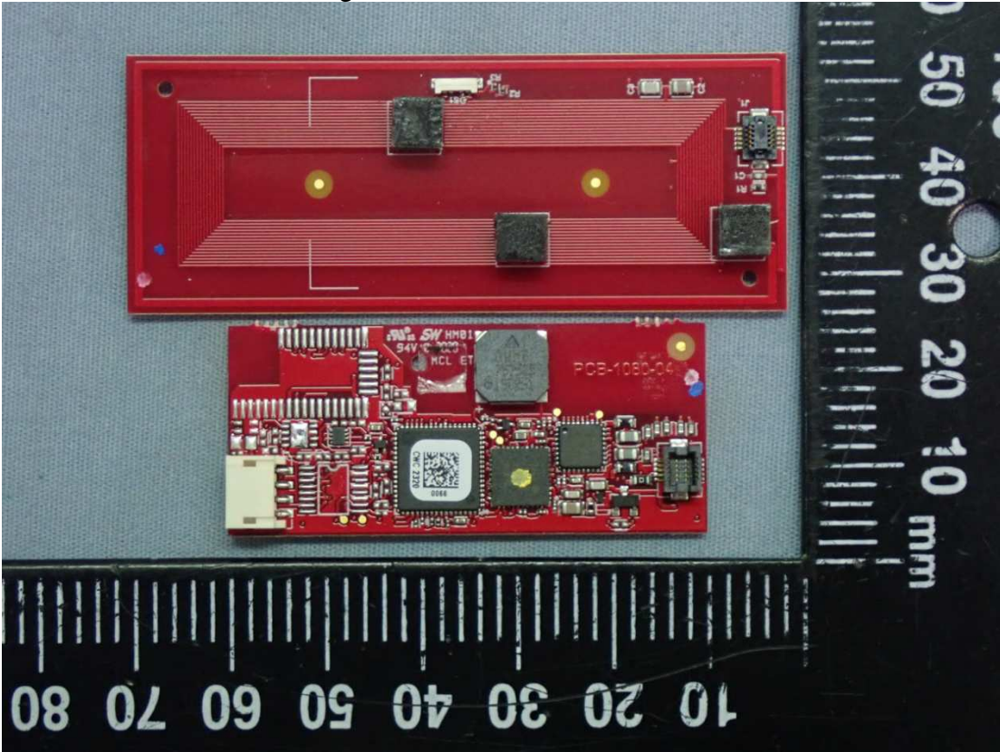
Figure 29 Integrated RFID Reader, Front View and RFID Antenna
