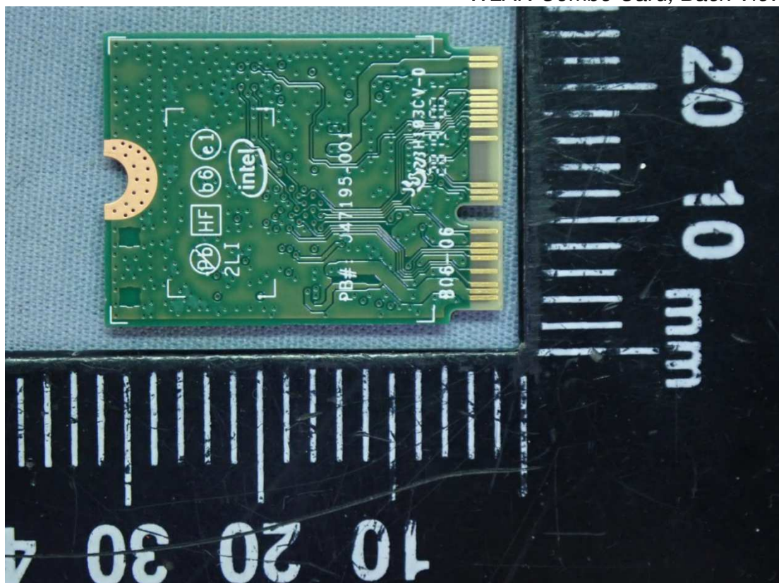
Figure 20 WLAN Combo Card, Back View
