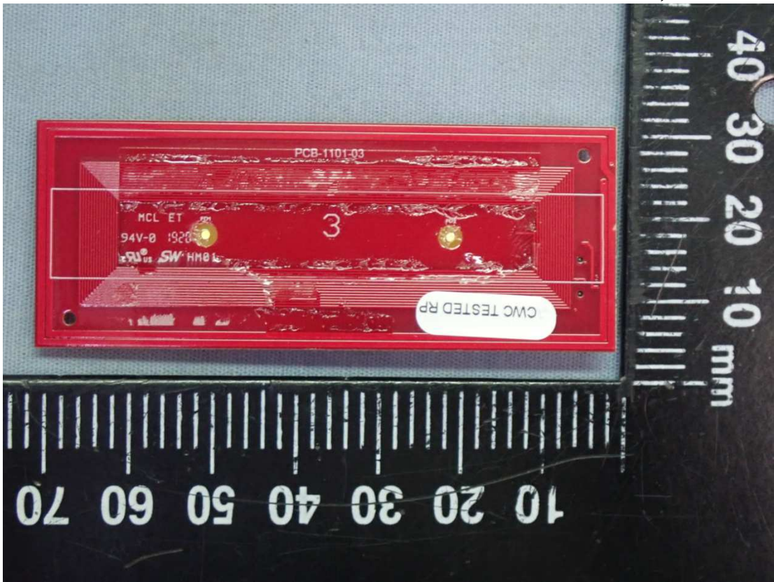
Figure 34 RFID Antenna, Back View
