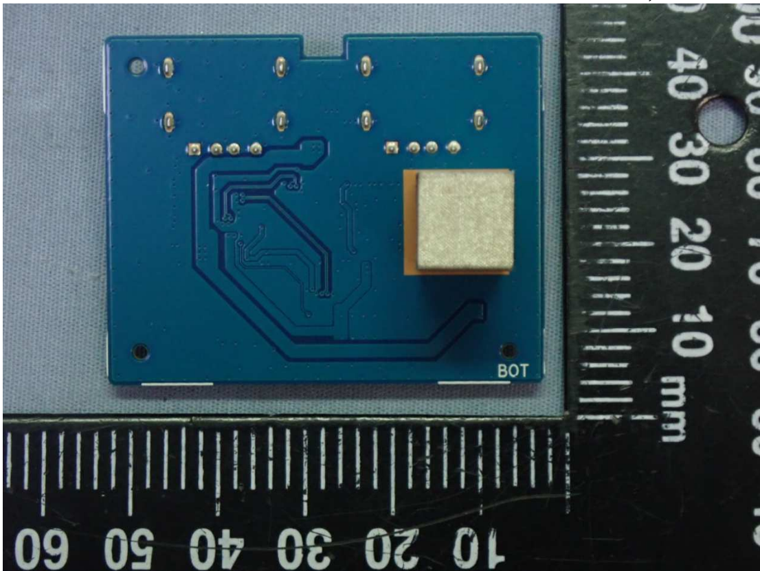
Figure 26 USB Control Board, Back View
