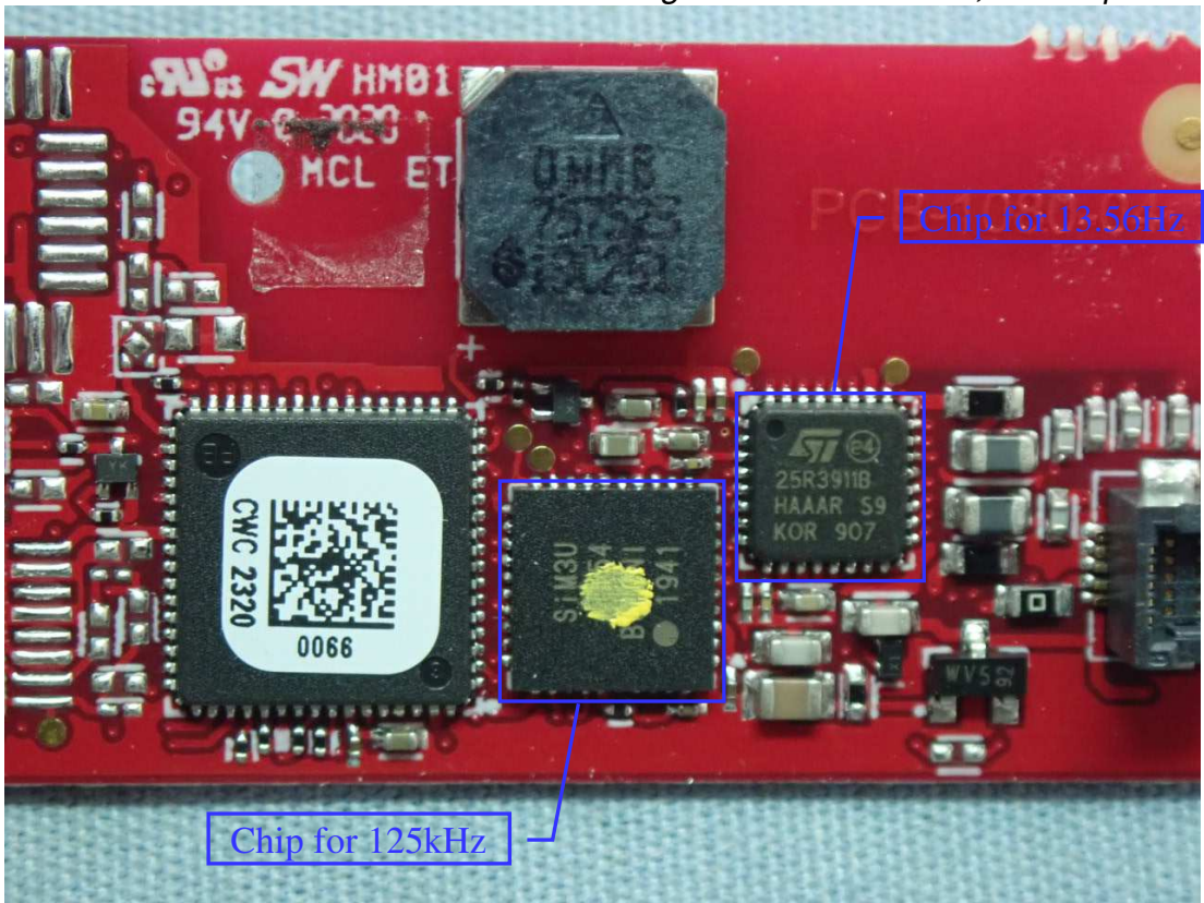
Figure 32 Integrated RFID Reader, RF Chip View
