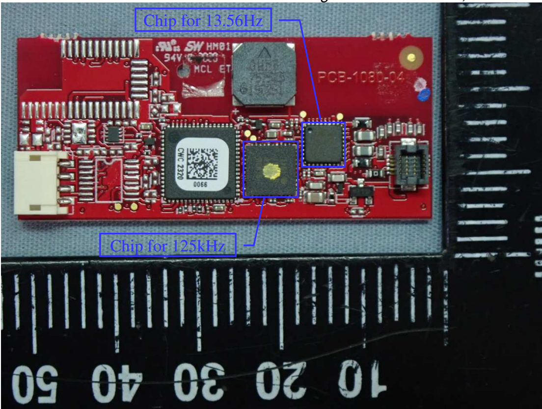
Figure 31 Integrated RFID Reader, Back View
