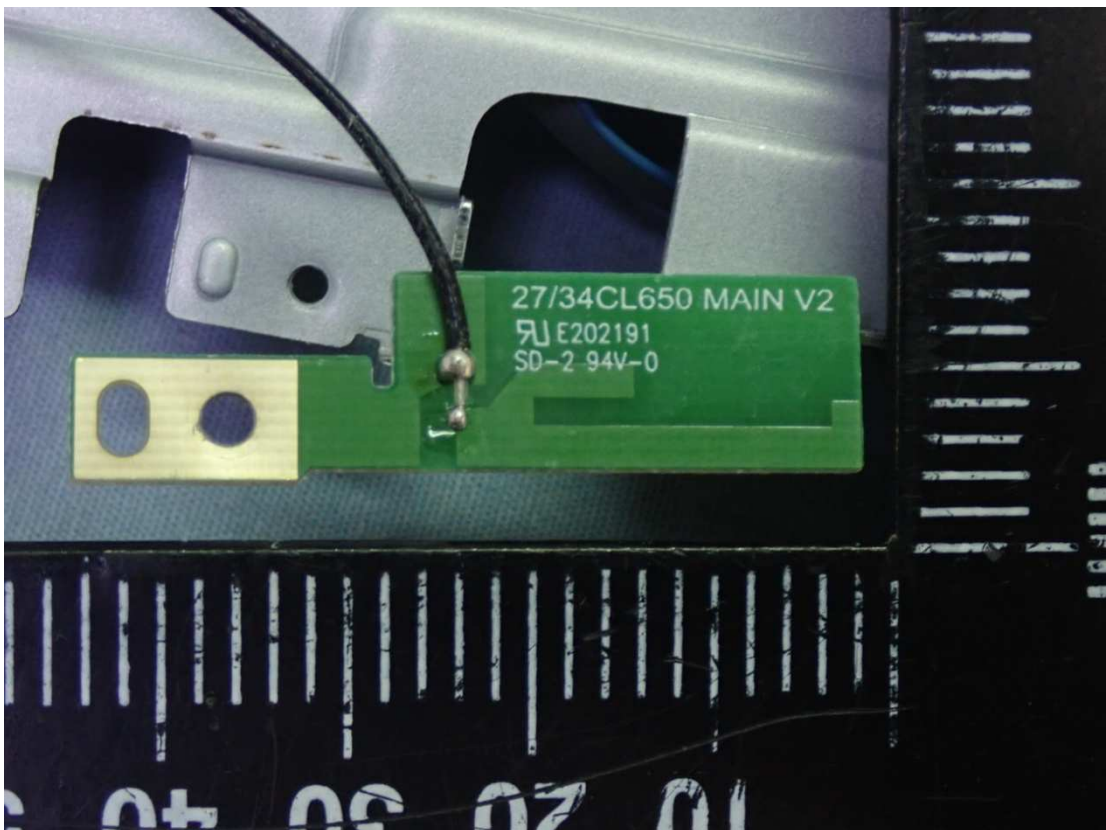
Figure 24 WLAN Combo Main Antenna
