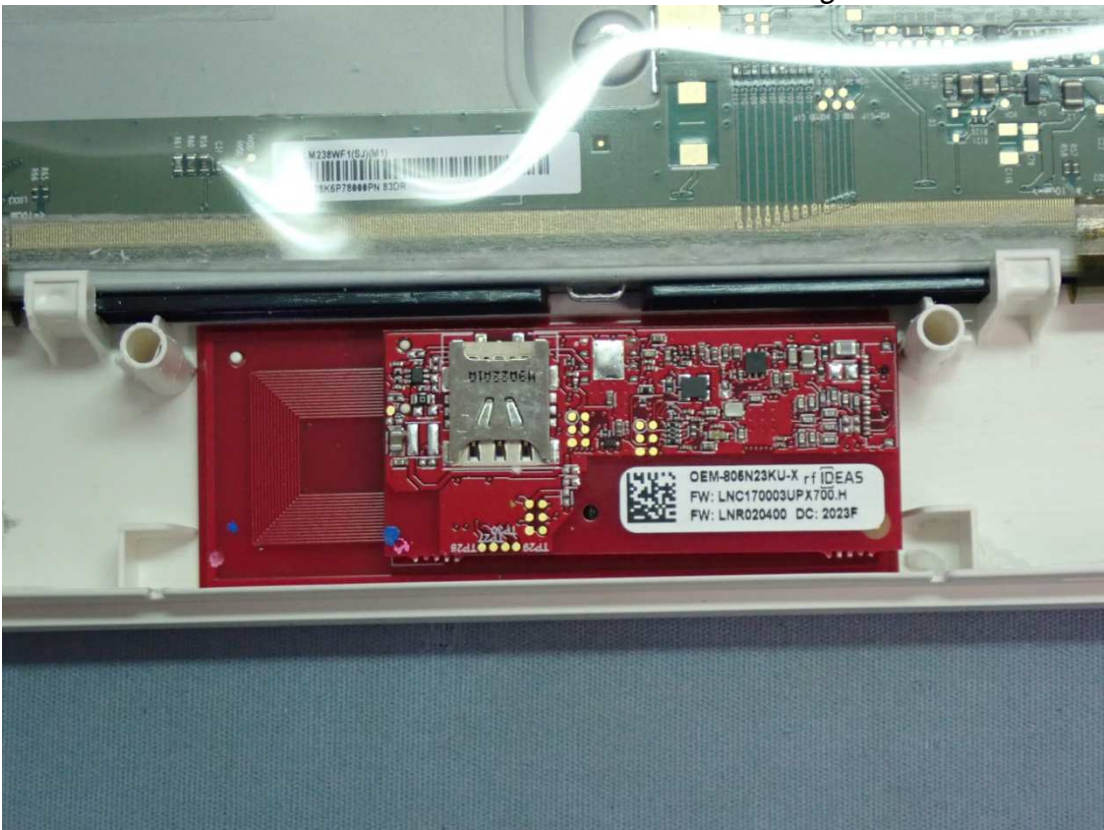
Figure 28 Integrated RFID Reader
