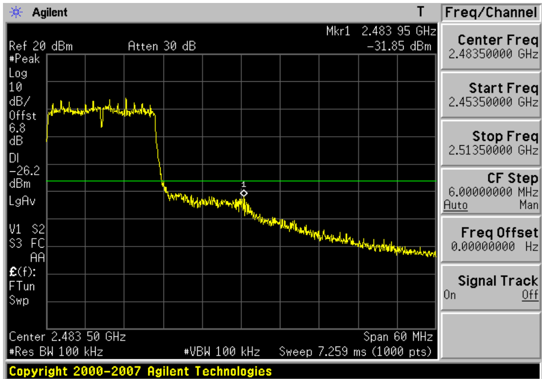
Plot 6-10. Band Edge Plot (802.11g - Ch. 11)
