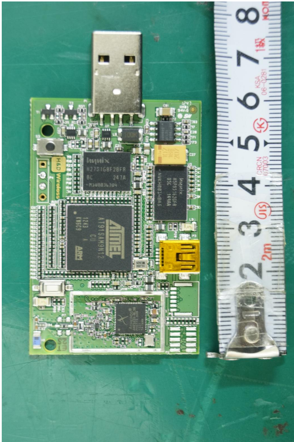
< Main board front (removed shield) >
