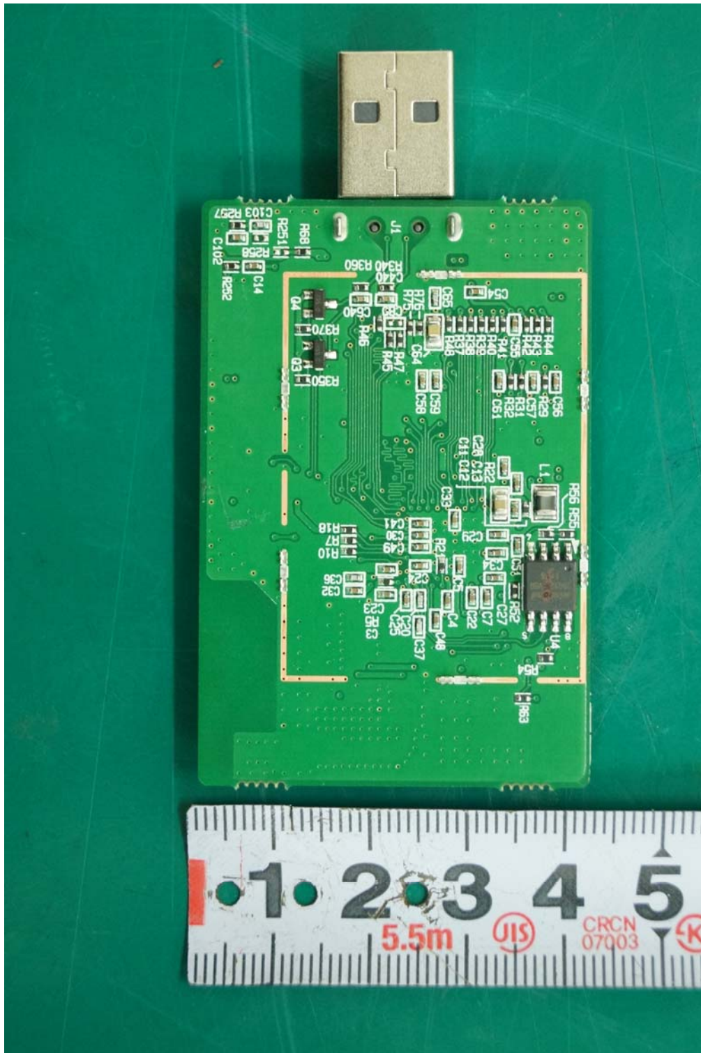
< Main board bottom view (removed shield) >
