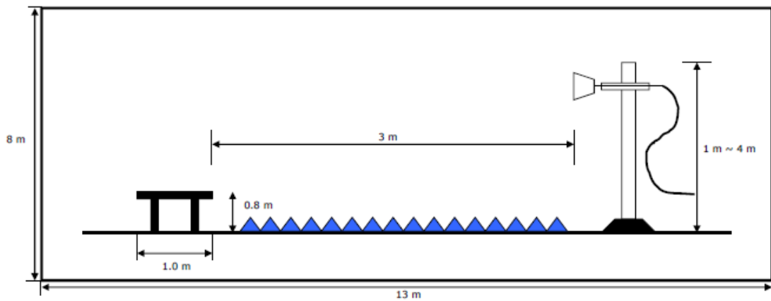
Fig 5. Dimensions of test site (Above 1GHz)
