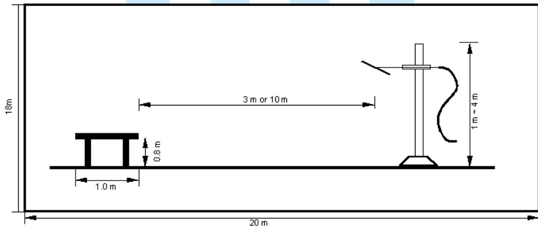
Fig 4. Dimensions of test site (Below 1GHz)
