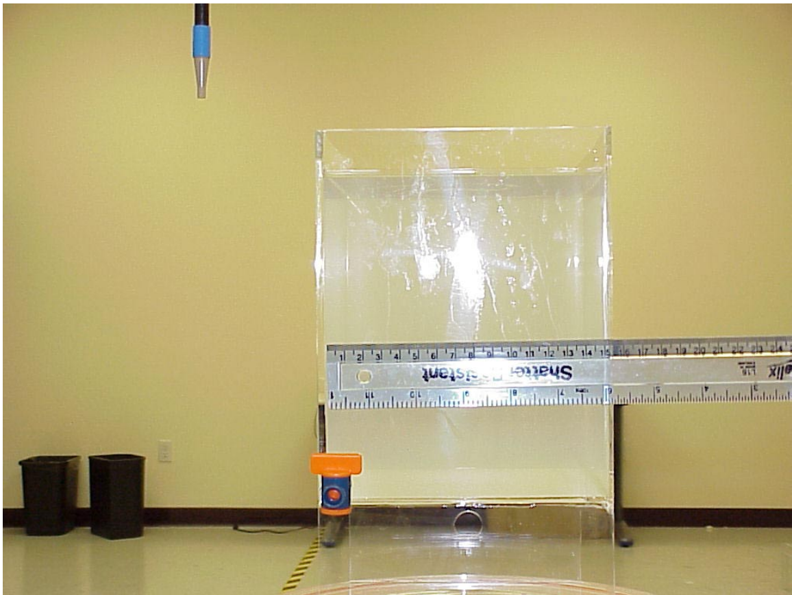
Photo 12. Photo to demonstrate 15 cm Z-axis flat phantom
