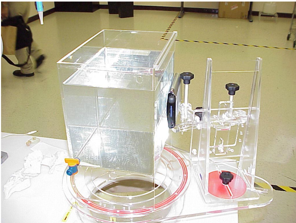
Photo 8. Screen to phantom
