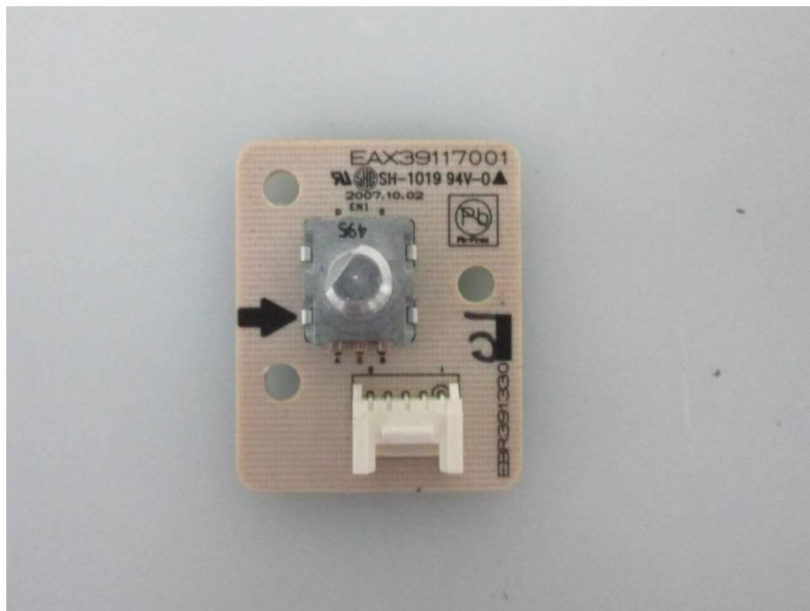
<PCB – Top of Control board (Dial)>
