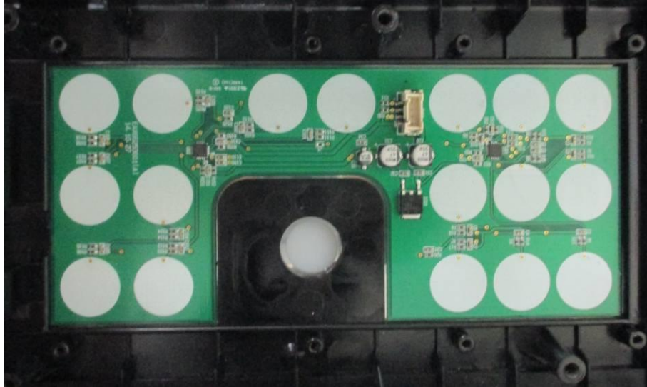
<PCB – Top of Control board>
