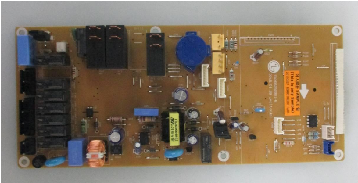
<PCB – Top of Main board>
