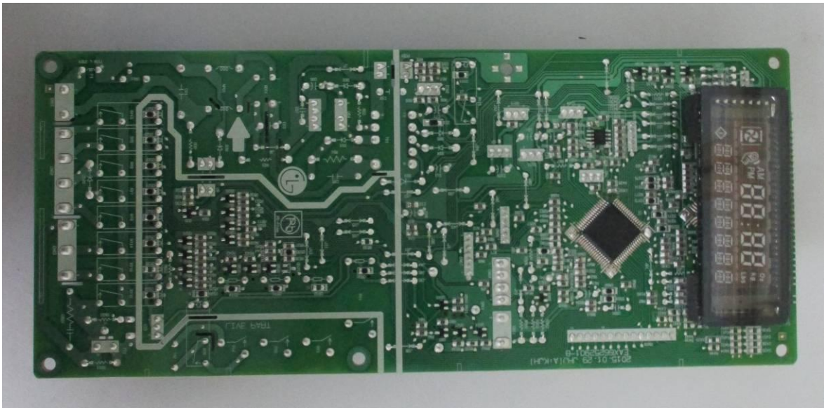
<PCB – Bottom of Main board>
