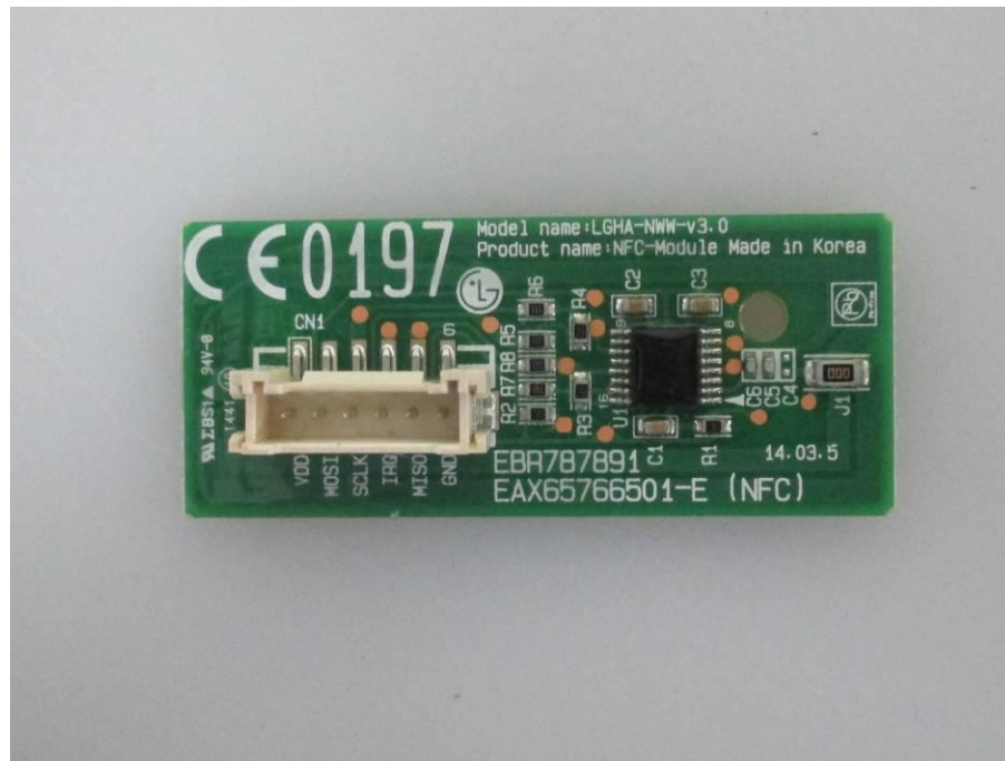
<PCB – Top of Passive type NFC Module>
