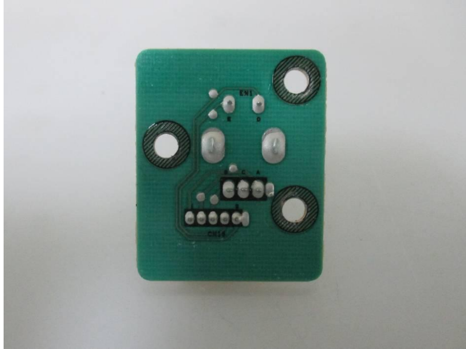
<PCB – Bottom of Control board (Dial)>
