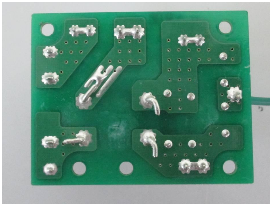
<Bottom of Noise filter>
