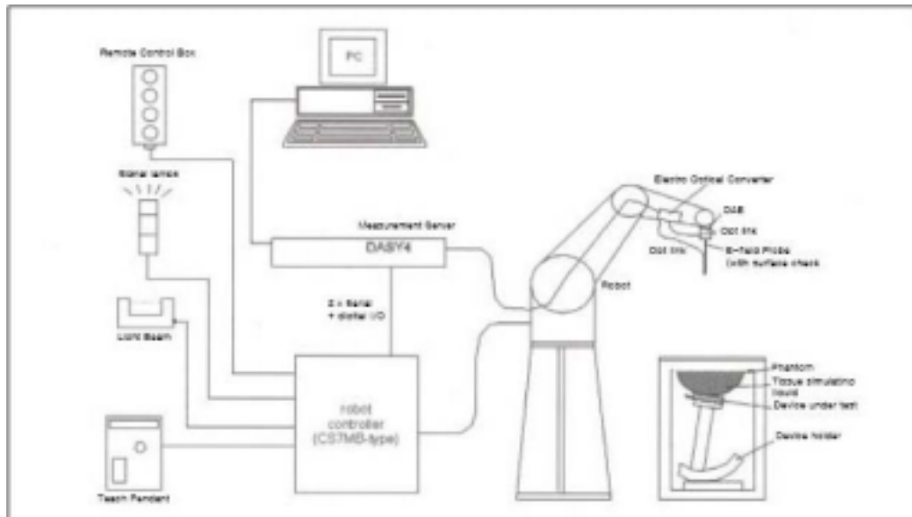
Fig. 5.1 SAR Measurement System Setup
