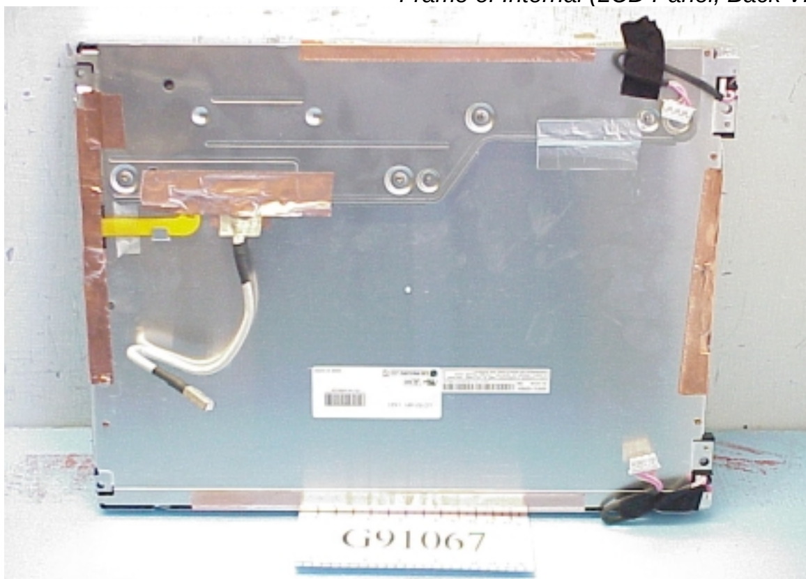
Figure 23 Frame of Internal (LCD Panel, Back View)
