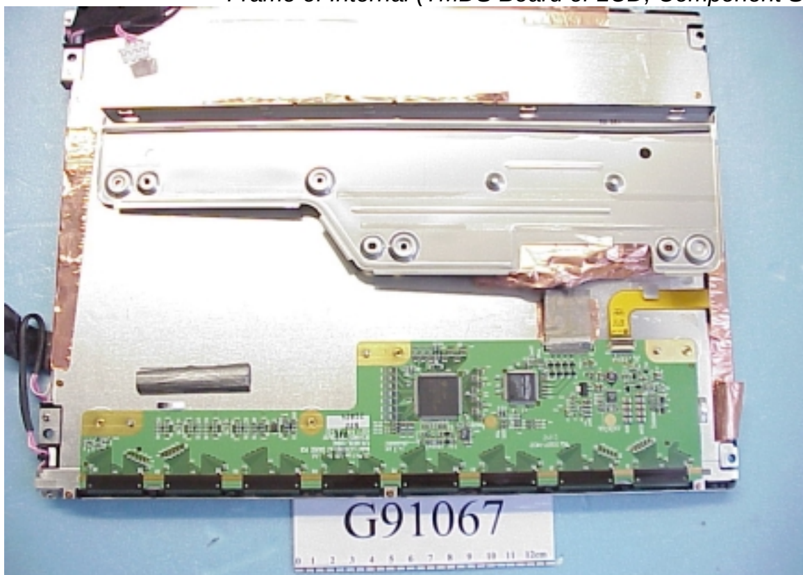
Figure 24 Frame of Internal (TMDS Board of LCD, Component Side)
