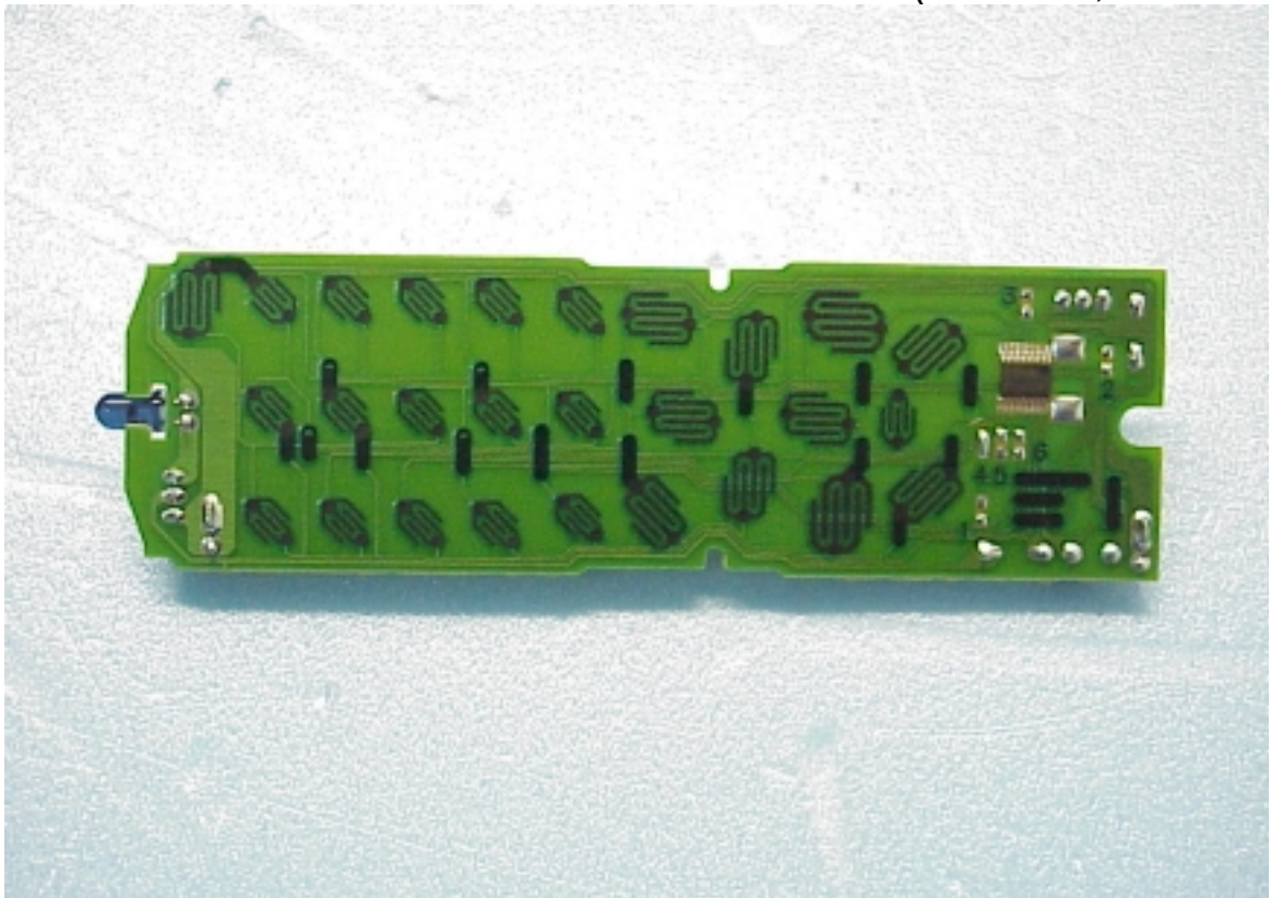
Figure 34 Remote Control (PCB View, Solder Side)
