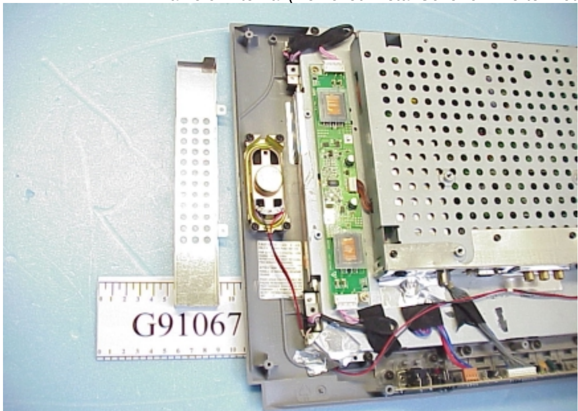
Figure 9 Frame of Internal (Removed Metal Cover of Inverter Board)
