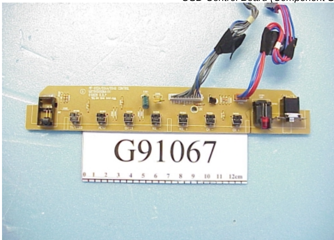
Figure 19 OSD Control Board (Component Side)
