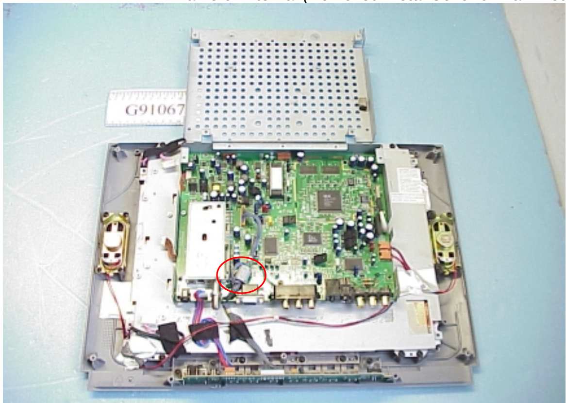
Figure 13 Frame of Internal (Removed Metal Cover of Main Board)
