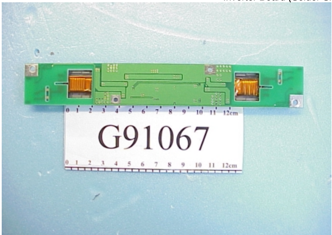
Figure 12 Inverter Board (Solder Side)
