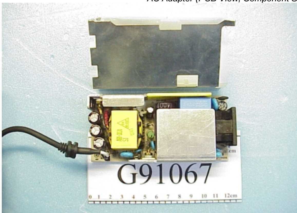
Figure 29 AC Adapter (PCB View, Component Side)
