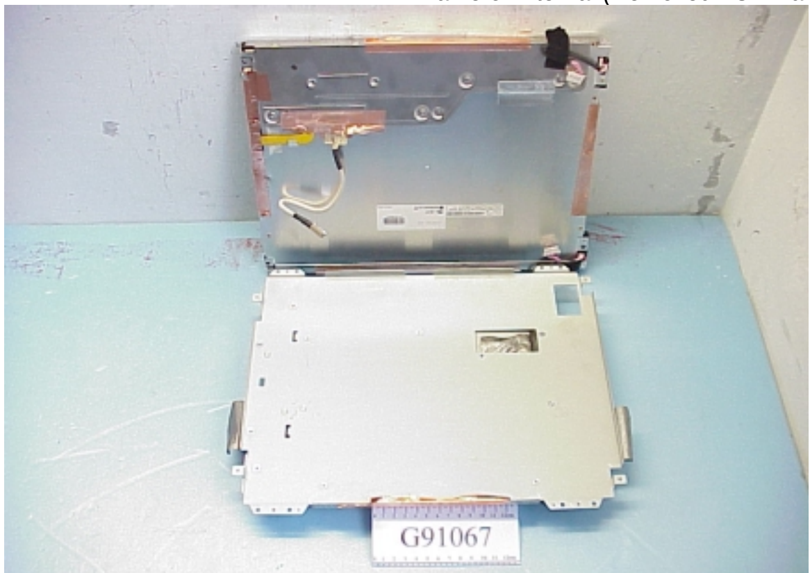
Figure 22 Frame of Internal (Removed LCD Panel)
