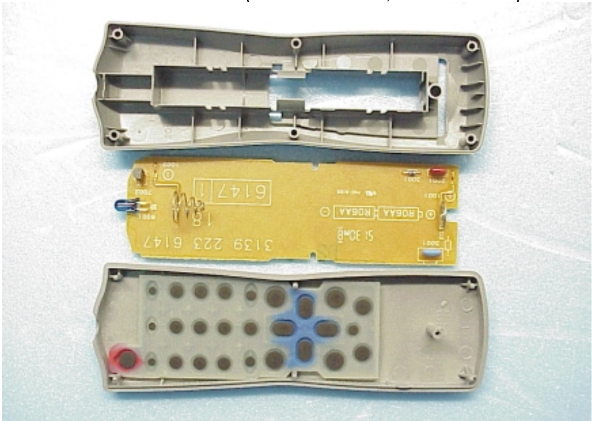
Figure 33 Remote Control (Removed Covers, PCB View/Component Side)
