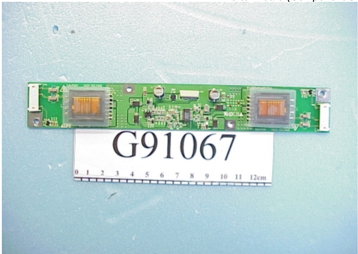
Figure 11 Inverter Board (Component Side)
