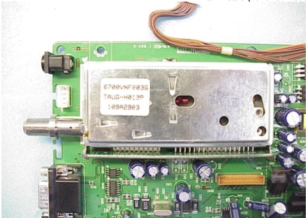
Figure 17 Main Board (w/Tuner Module)
