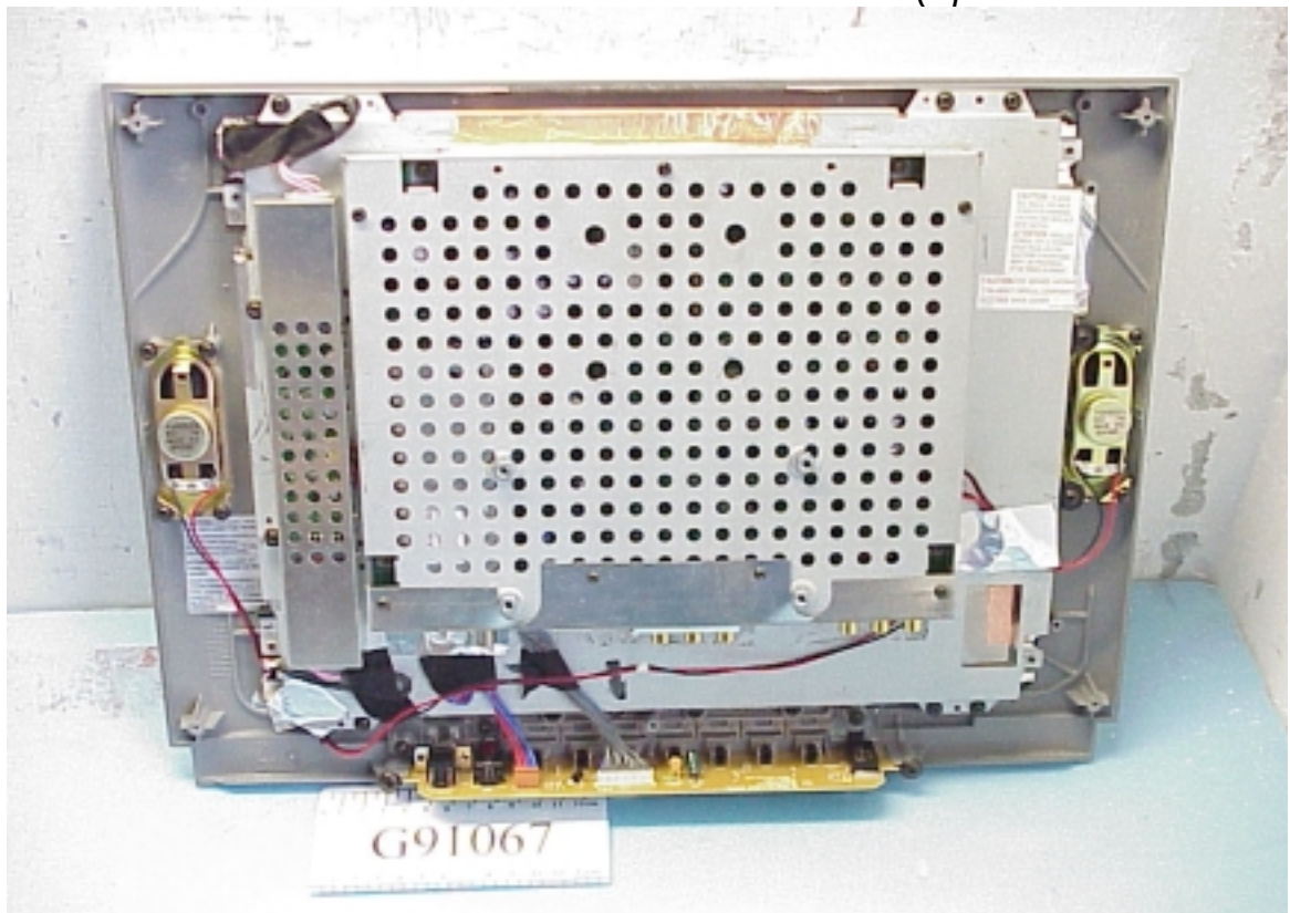
Figure 8 Frame of Internal (Speakers & Main Board)
