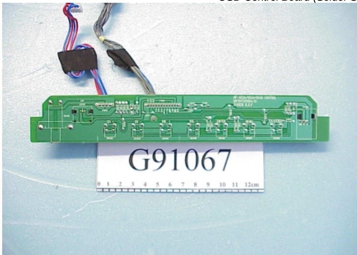
Figure 20 OSD Control Board (Solder Side)
