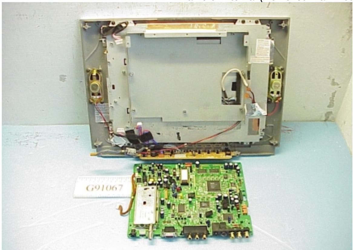
Figure 14 Frame of Internal (Removed Main Board)
