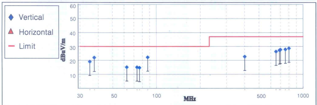
&lt; Fig 5. Radiated emission result _ Digital &gt;
