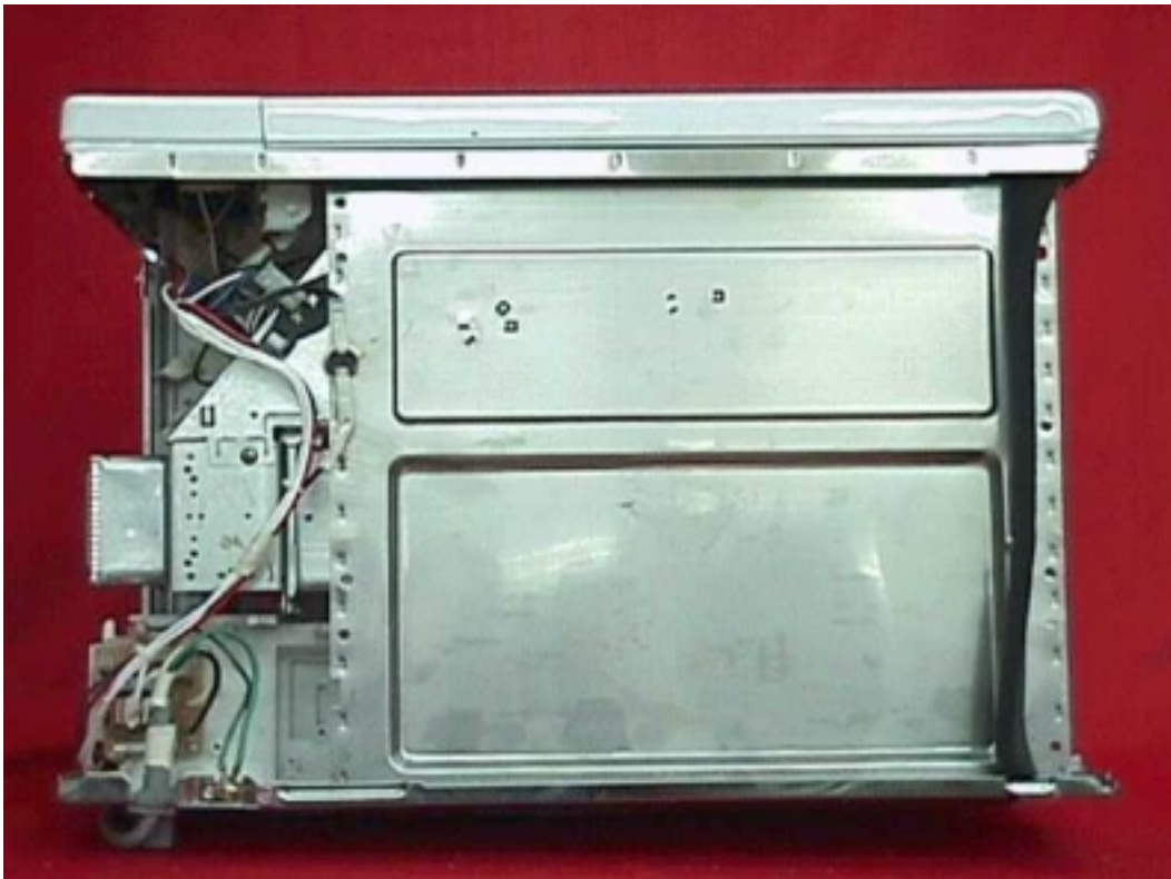
Upper Part View without enclosure
