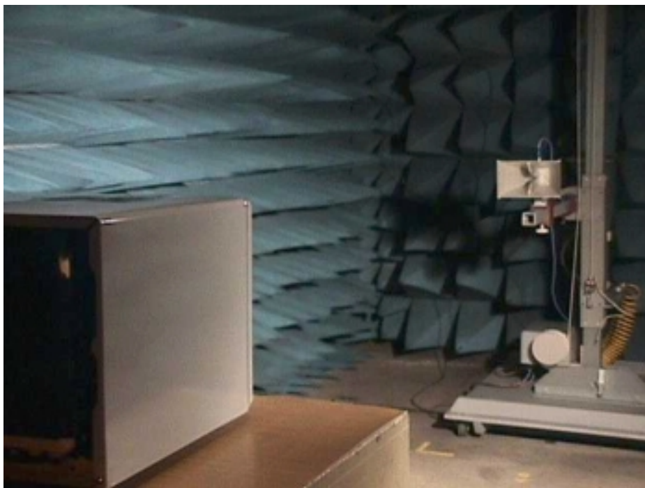
Test Set-Up Photo(1)
