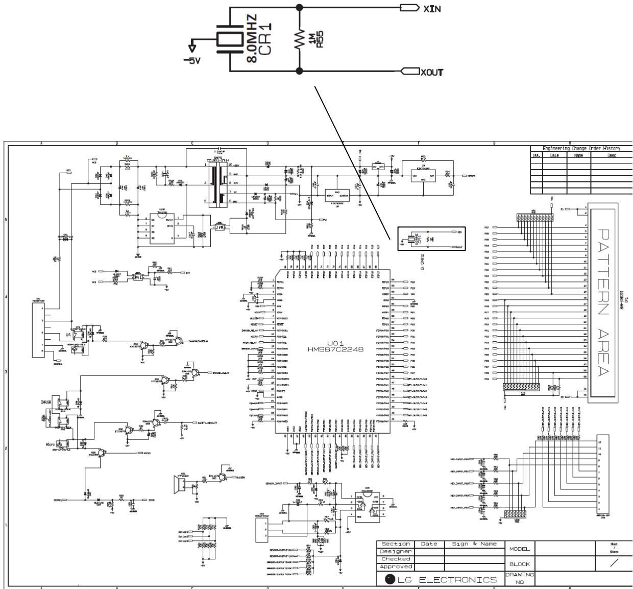
<Fig. 4. PCB Circuit Diagram>
