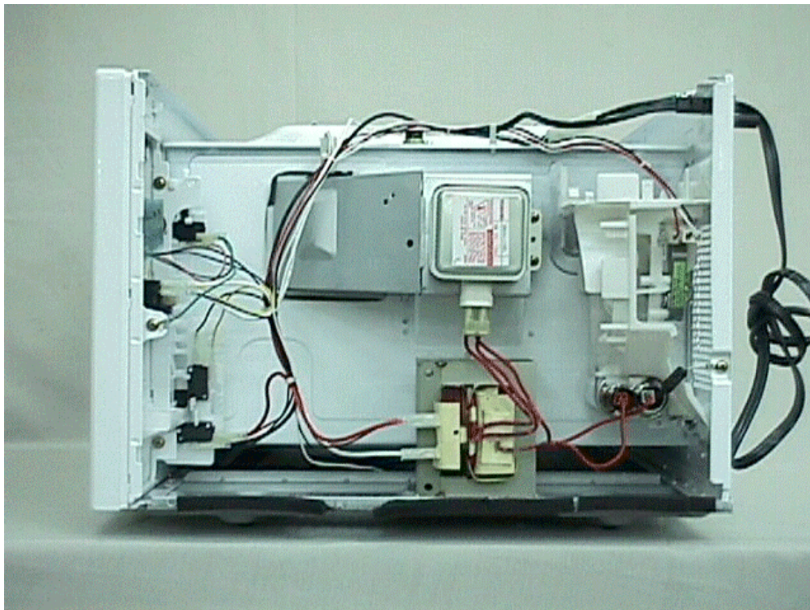
WAVE GUIDE VIEW
