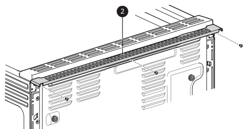
2 Rear filler
