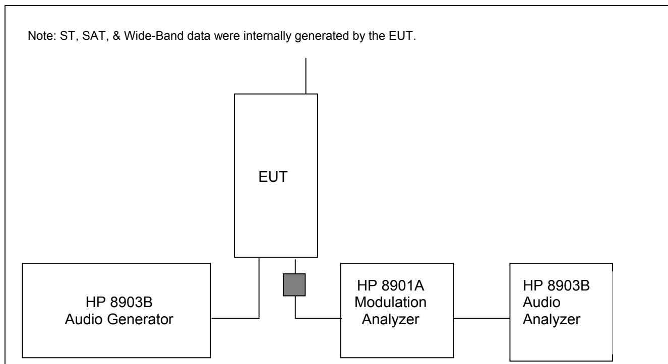
Fig. 3. Transmitter Audio Frequency & Tone Modulation Test Setup.
