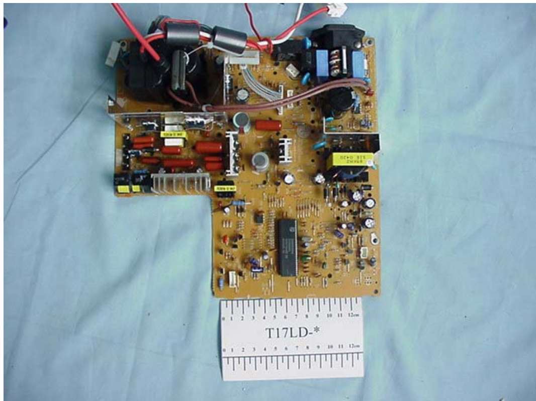
FIGURE 5 COLOR MONITOR (M/N: T17LD-*) MAIN BOARD (COMPONENT SIDE)
