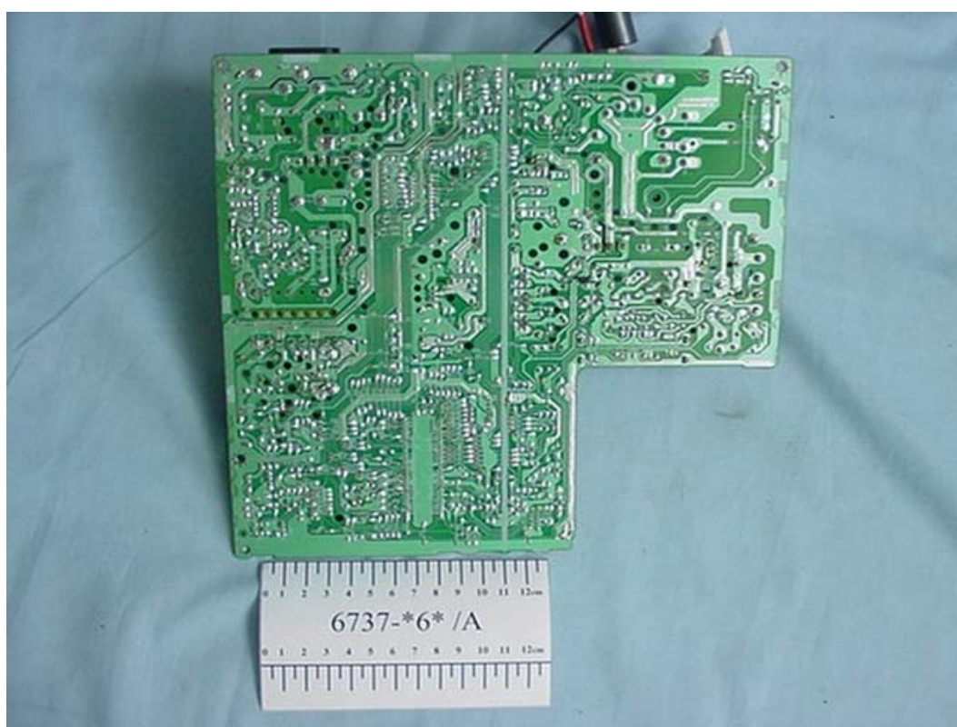
FIGURE 16 COLOR MONITOR (M/N: 6737-*6* /A) MAIN BOARD (SOLDERED SIDE)
