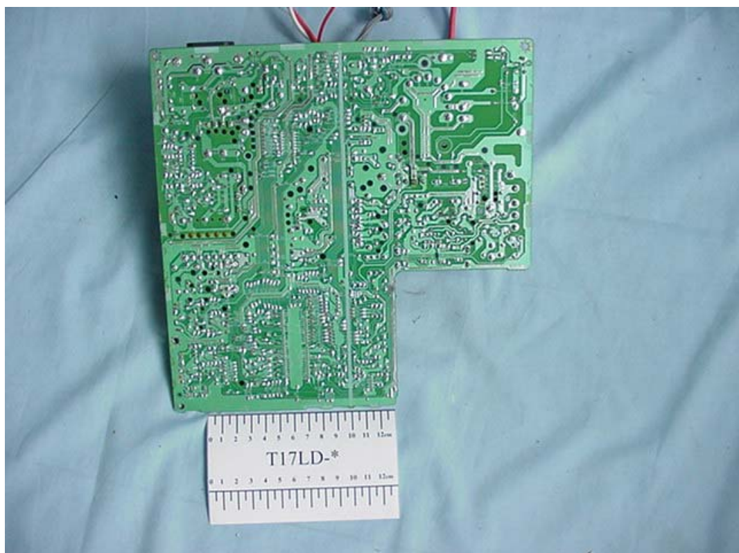
FIGURE 6 COLOR MONITOR (M/N: T17LD-*) MAIN BOARD (SOLDERED SIDE)
