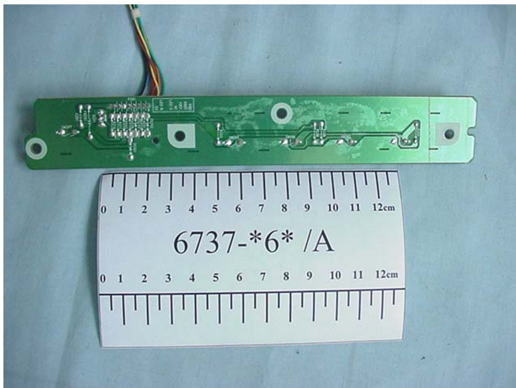
FIGURE 20 COLOR MONITOR (M/N: 6737-*6* /A) CONTROL BOARD (SOLDERED SIDE)
