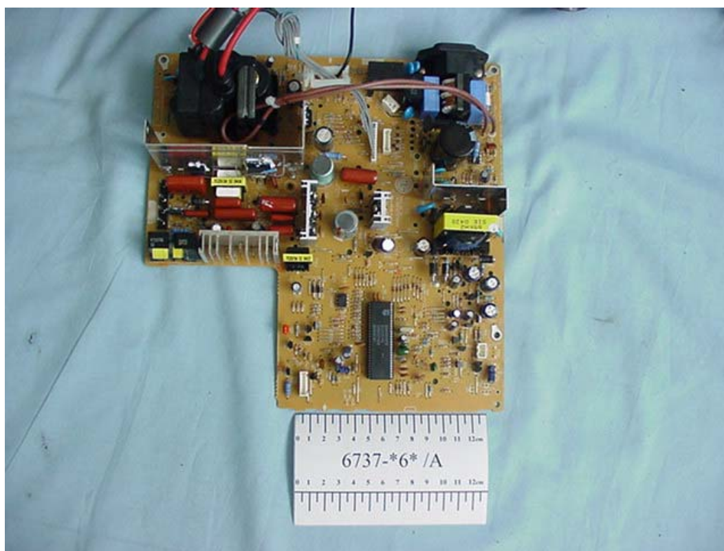
FIGURE 15 COLOR MONITOR (M/N: 6737-*6* /A) MAIN BOARD (COMPONENT SIDE)
