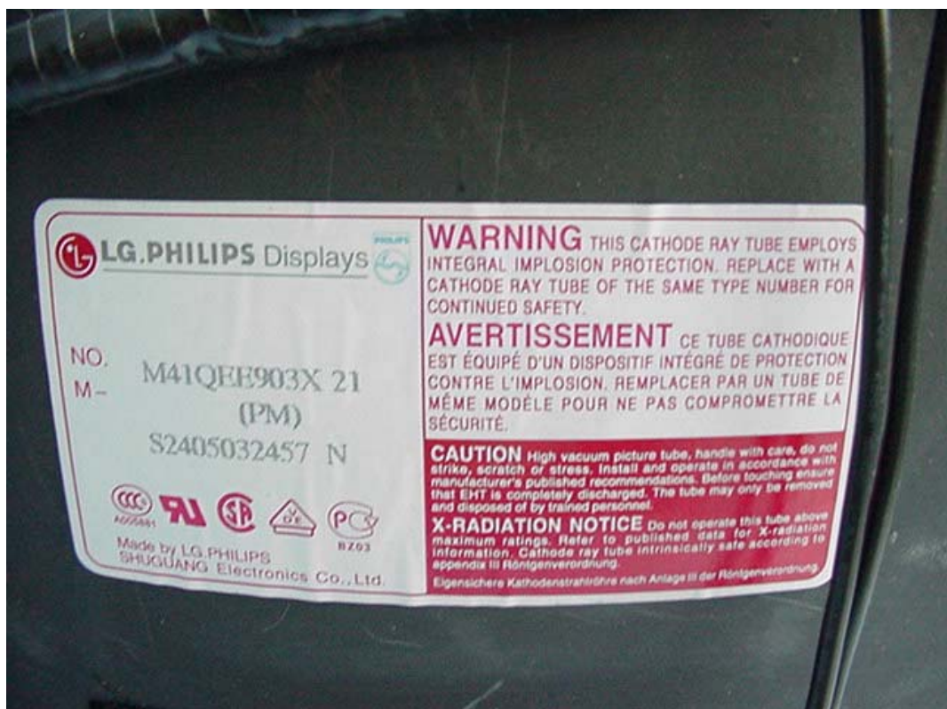
FIGURE 4 COLOR MONITOR (M/N: T17LD-*) CRT LABEL
