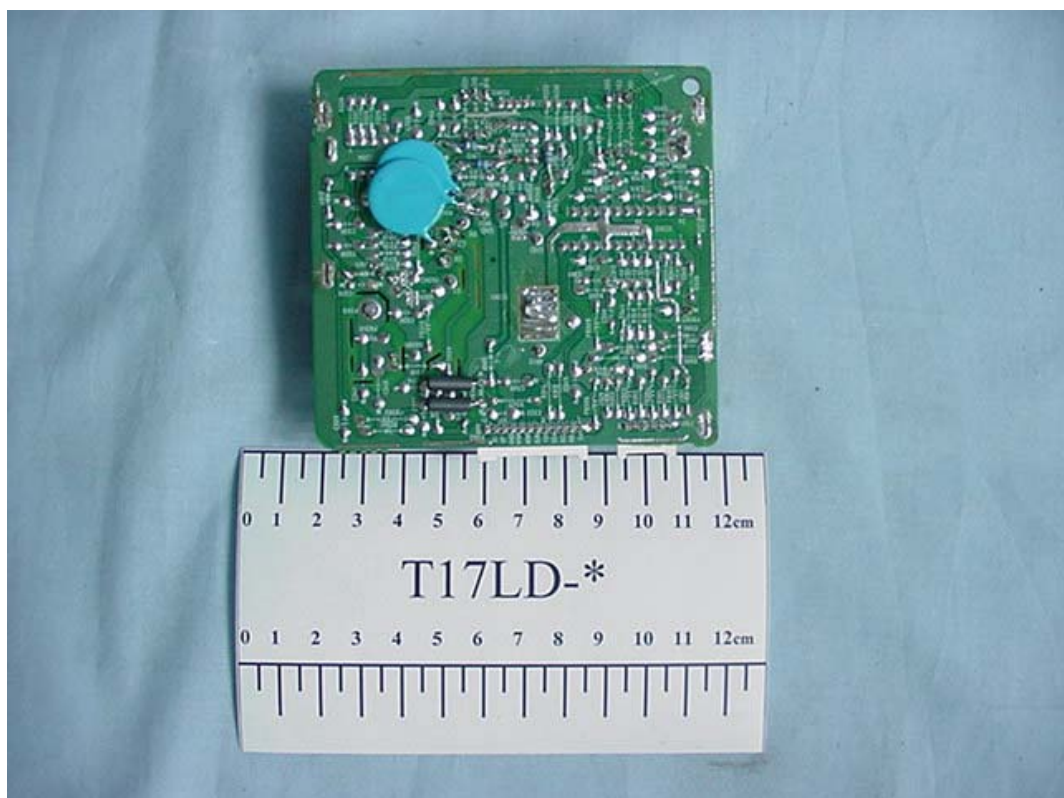
FIGURE 8 COLOR MONITOR (M/N: T17LD-*) VIDEO BOARD (SOLDERED SIDE)
