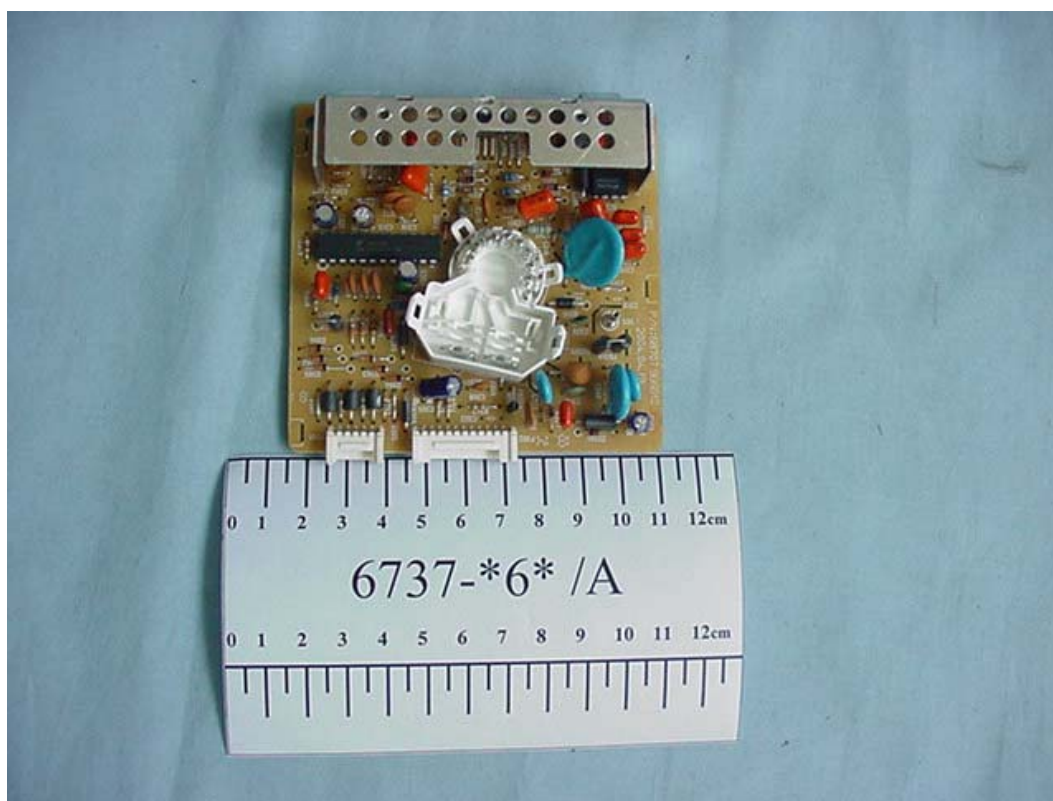
FIGURE 17 COLOR MONITOR (M/N: 6737-*6* /A) VIDEO BOARD (COMPONENT SIDE)
