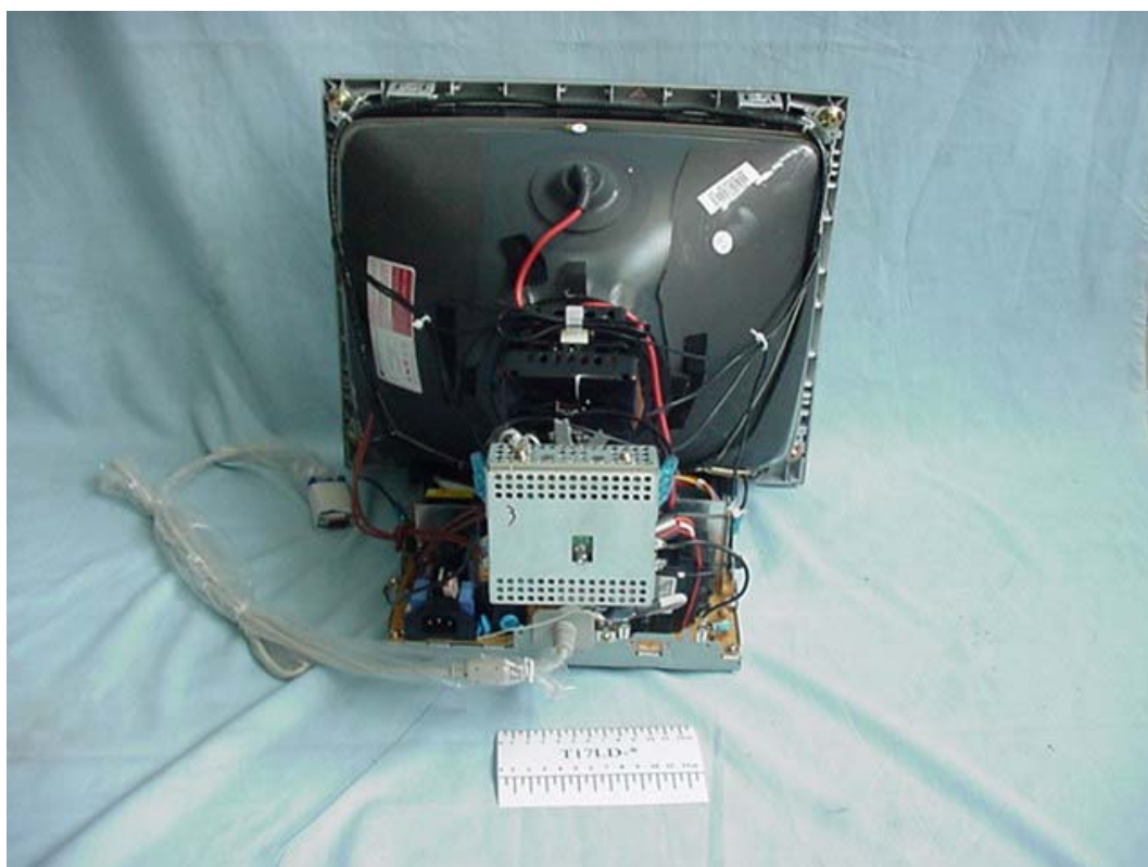
FIGURE 2 COLOR MONITOR (M/N: T17LD-*) COVER REMOVED 2
