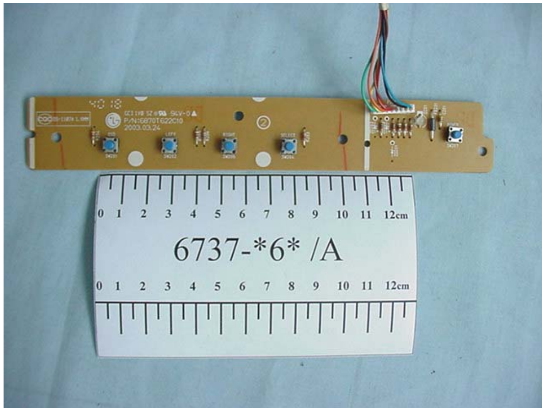
FIGURE 19 COLOR MONITOR (M/N: 6737-*6* /A) CONTROL BOARD (COMPONENT SIDE)
