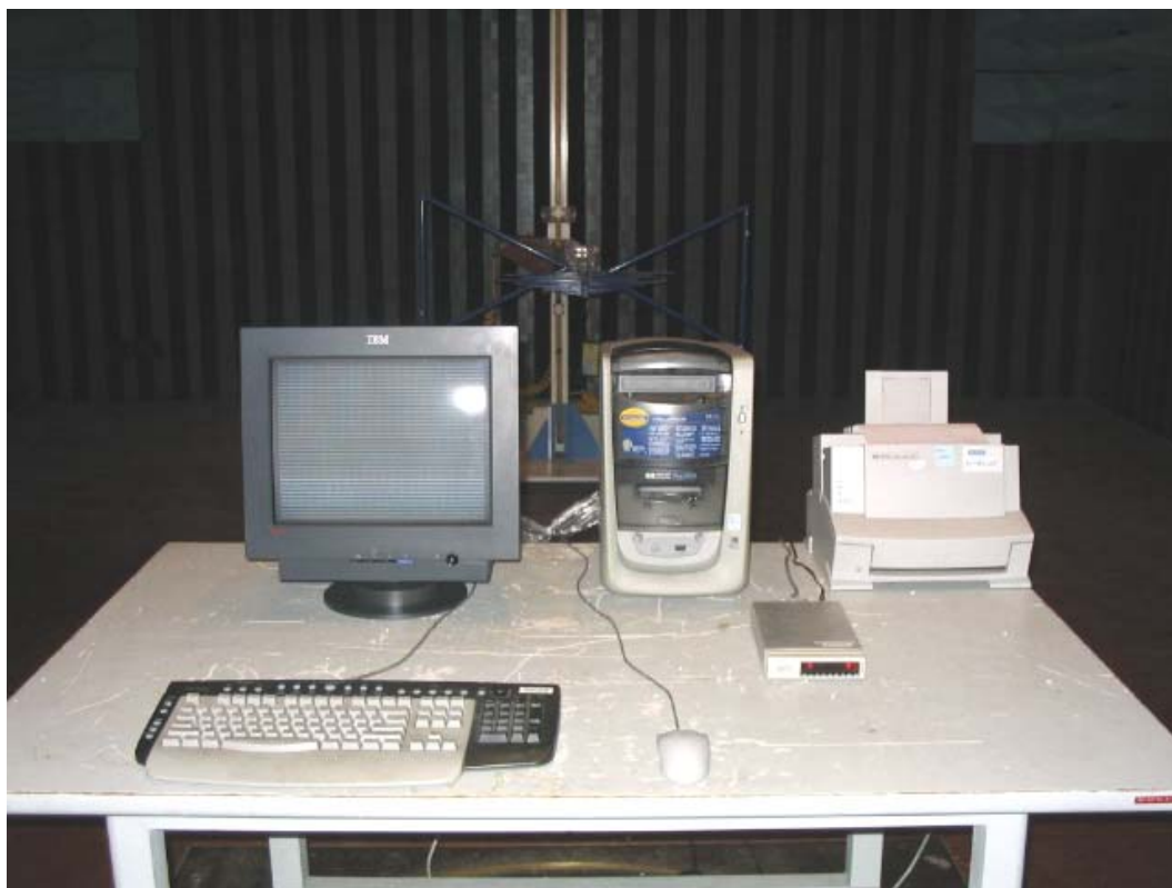
FRONT VIEW OF RADIATED EMISSION TEST (M/N: 6737-*6* /A)
