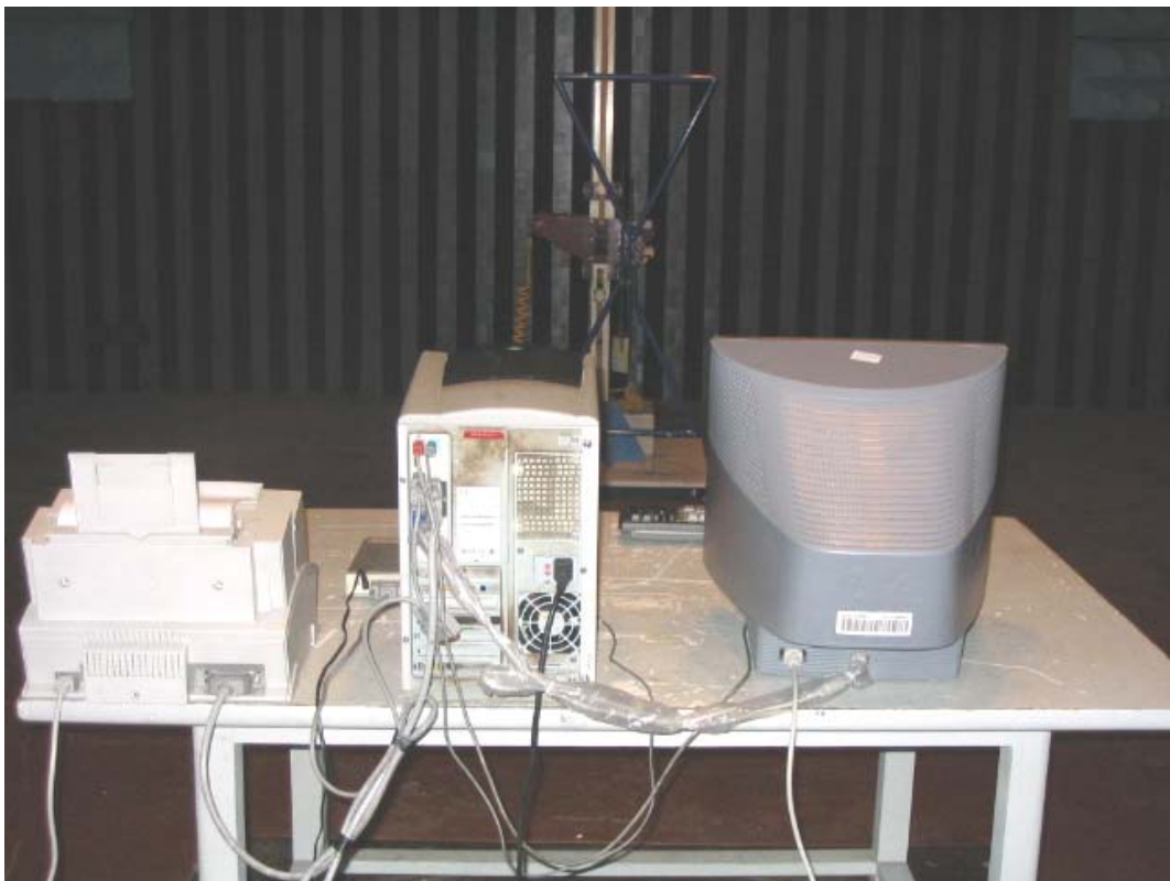
BACK VIEW OF RADIATED EMISSION TEST (M/N: T17LD-*)
