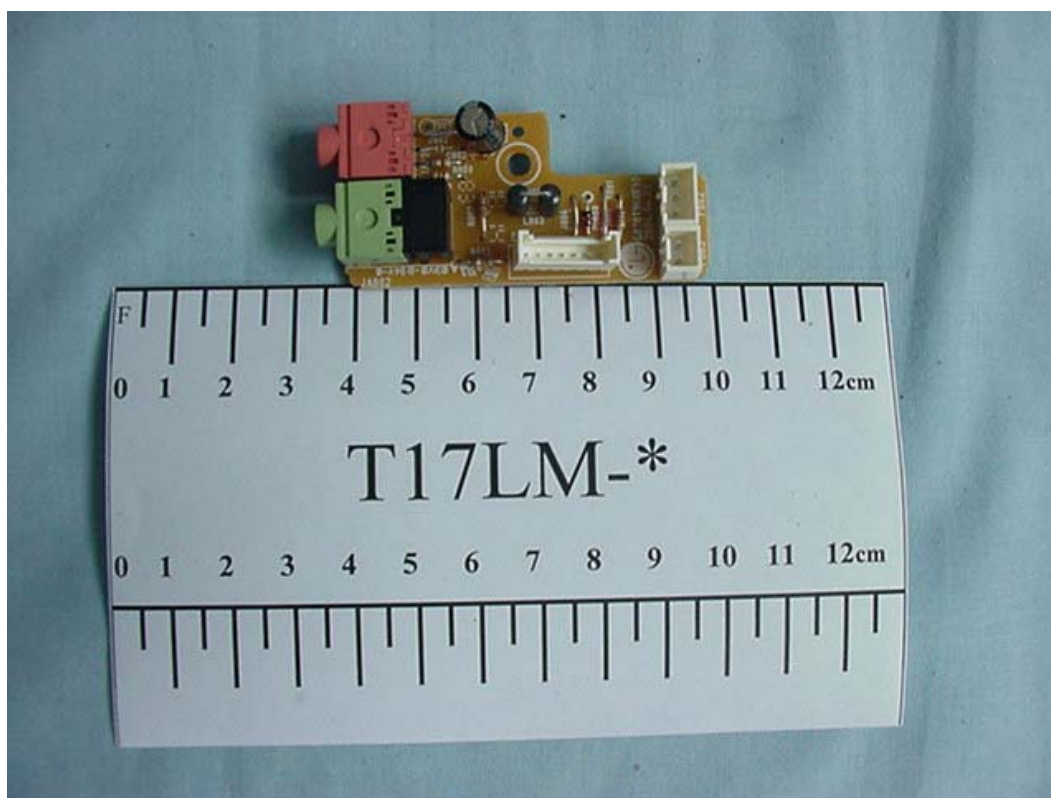
FIGURE 10 COLOR MONITOR (M/N:T17LM-*) AUDIO BOARD (COMPONENT SIDE)
