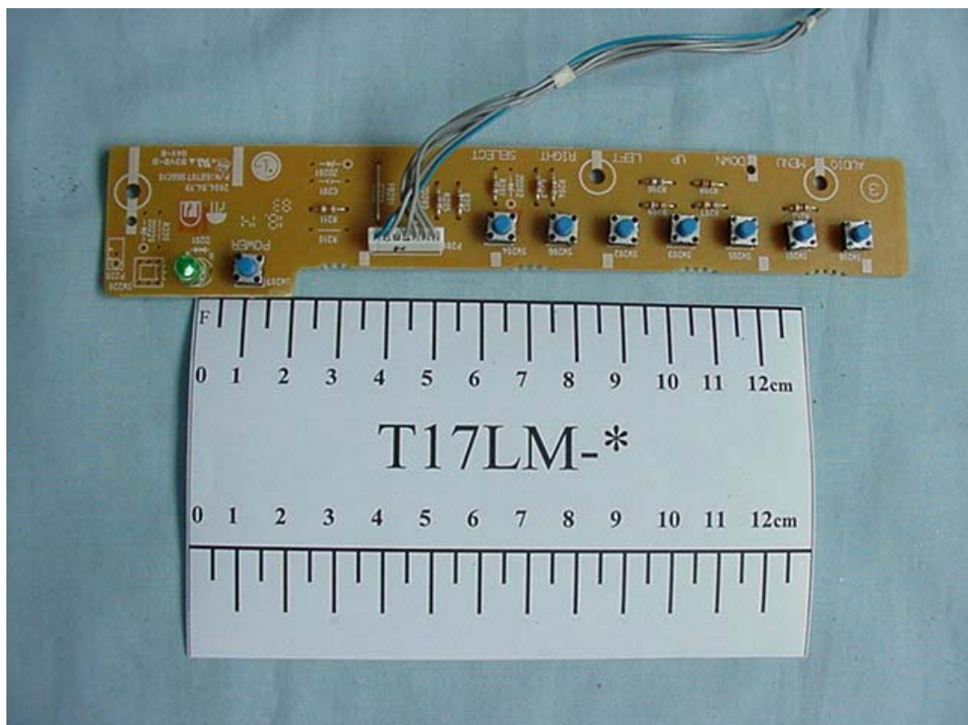
FIGURE 8 COLOR MONITOR (M/N:T17LM-*) CONTROL PANEL BOARD (COMPONENT SIDE)
