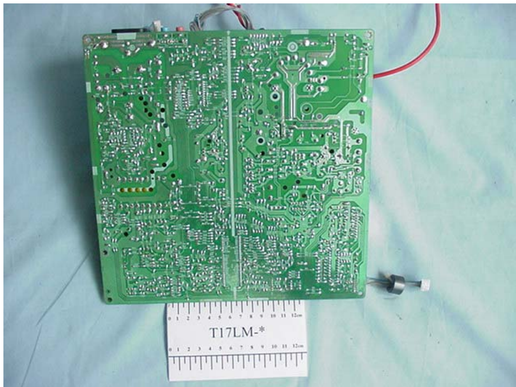
FIGURE 5 COLOR MONITOR (M/N:T17LM-*) MAIN BOARD (SOLDERED SIDE)
