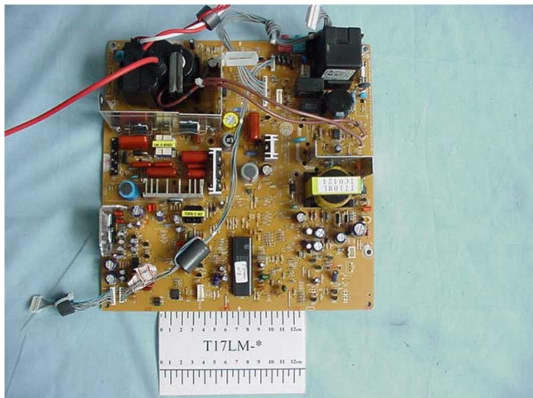
FIGURE 4 COLOR MONITOR (M/N:T17LM-*) MAIN BOARD (COMPONENT SIDE)
