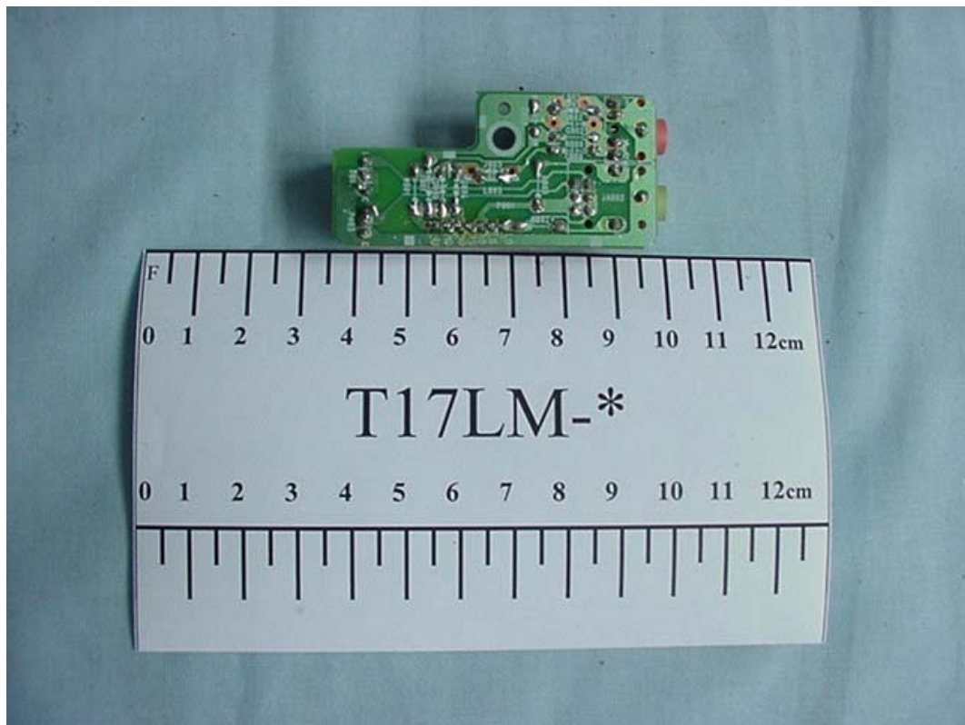
FIGURE 11 COLOR MONITOR (M/N:T17LM-*) AUDIO BOARD (SOLDERED SIDE)
