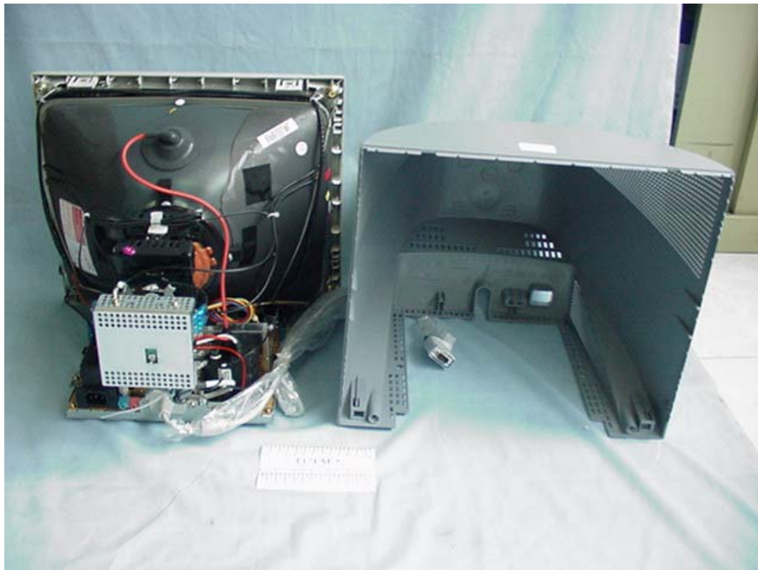
FIGURE 1 COLOR MONITOR (M/N:T17LM-*) COVER REMOVED
