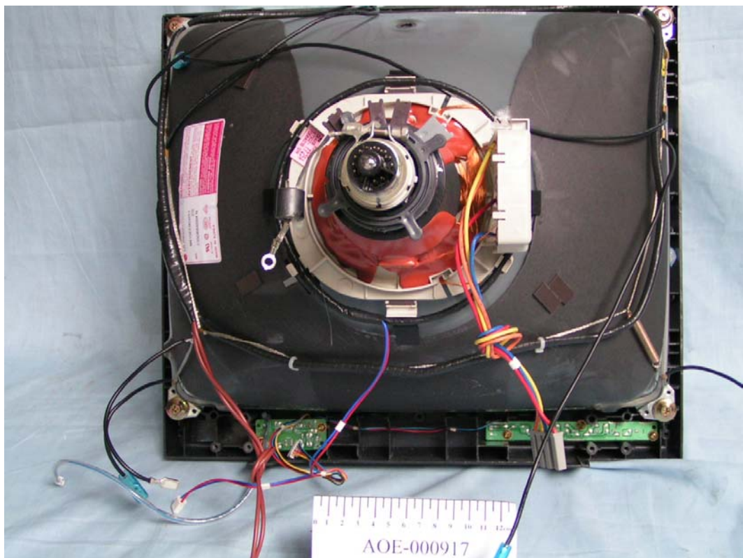
FIGURE 2 COLOR MONITOR (M/N: T17NC-*) COVER REMOVED 2
