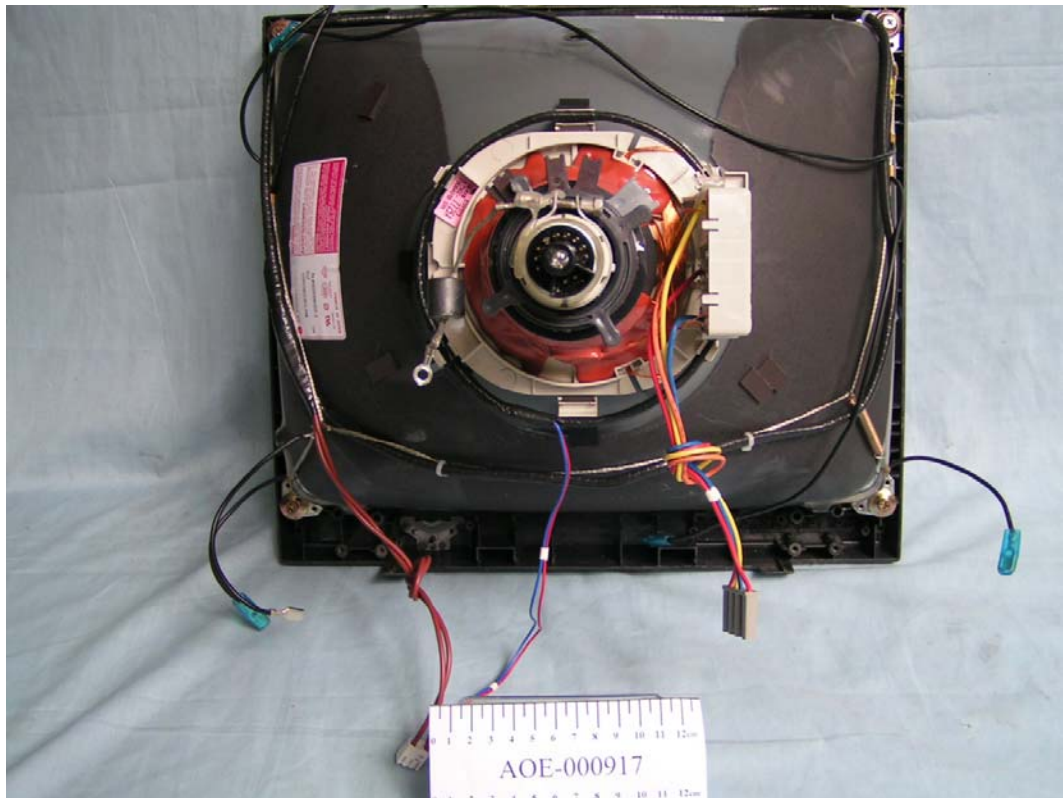
FIGURE 3 COLOR MONITOR (M/N: T17NC-*) CRT GENERAL APPEARANCE
