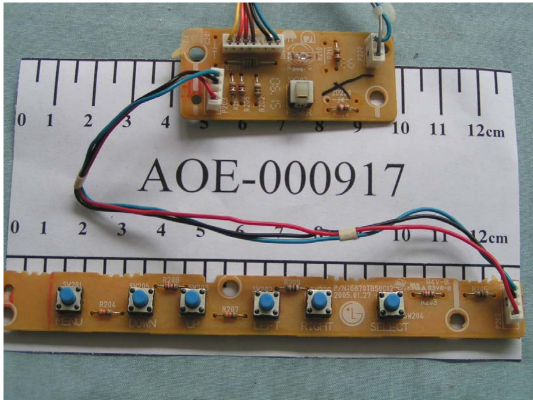
FIGURE 18 COLOR MONITOR (M/N: T17NC-*) BUTTON BOARD (COMPONENT SIDE)
