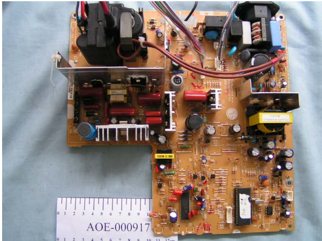
FIGURE 7 COLOR MONITOR (M/N: T17NC-*) MAIN BOARD (COMPONENT SIDE)
