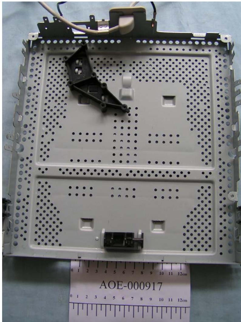
FIGURE 12 COLOR MONITOR (M/N: T17NC-*) MAIN BOARD HOLDER (FRONT VIEW)
