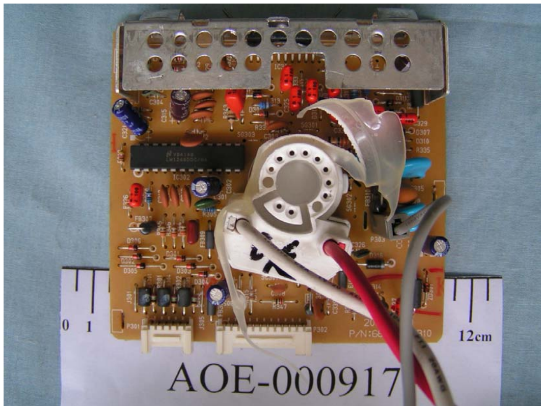
FIGURE 15 COLOR MONITOR (M/N: T17NC-*) CRT BOARD (COMPONENT SIDE)
