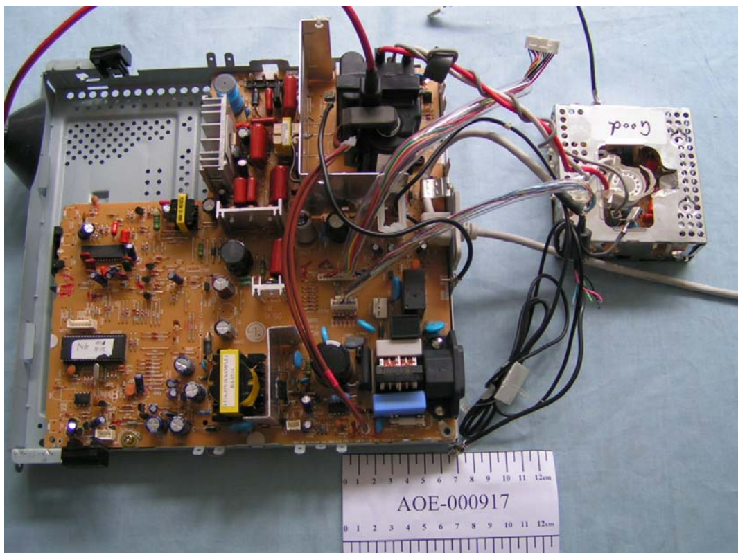
FIGURE 6 COLOR MONITOR (M/N: T17NC-*) MAIN BOARD & CRT BOARD
