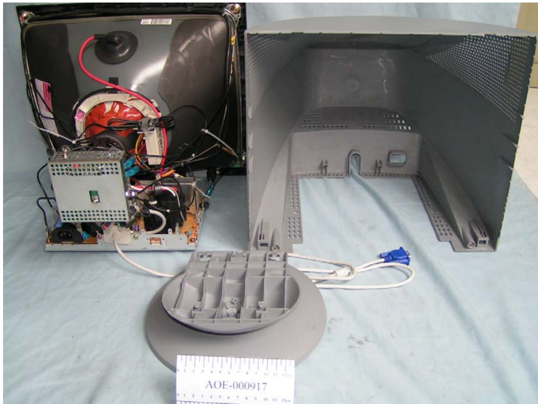
FIGURE 1 COLOR MONITOR (M/N: T17NC-*) COVER REMOVED 1
