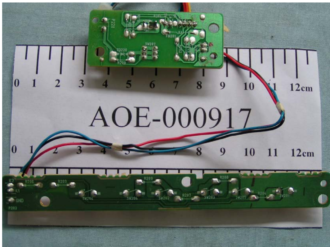
FIGURE 19 COLOR MONITOR (M/N: T17NC-*) BUTTON BOARD (SOLDERED SIDE)
