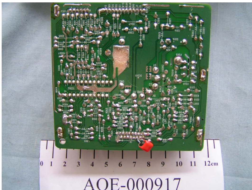
FIGURE 16 COLOR MONITOR (M/N: T17NC-*) CRT BOARD (SOLDERED SIDE)
