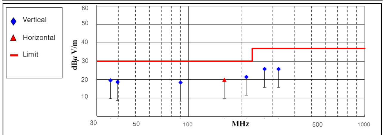
< Fig 10. Radiated emission result (30 MHz ~ 1 000 MHz)>
