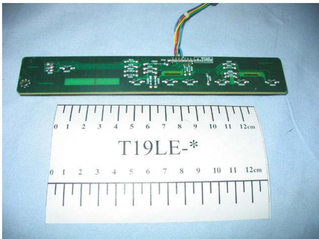
FIGURE 10 COLOR MONITOR (M/N:T19LE-*) CONTROL PANEL BOARD (SOLDERED SIDE)
