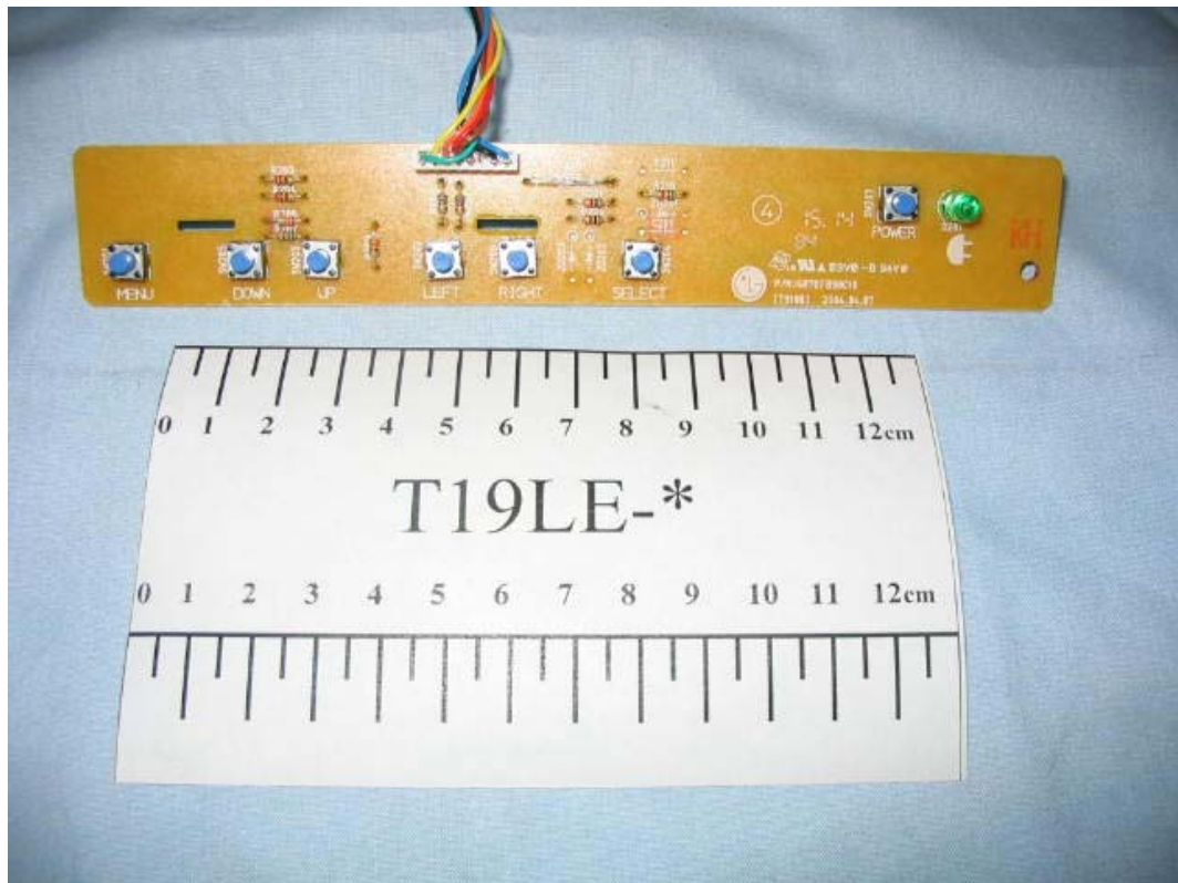
FIGURE 9 COLOR MONITOR (M/N:T19LE-*) CONTROL PANEL BOARD (COMPONENT SIDE)
