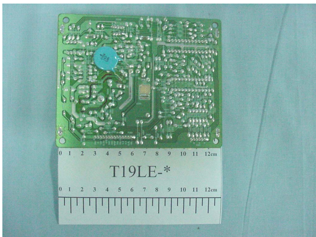
FIGURE 8 COLOR MONITOR (M/N:T19LE-*) CRT BOARD (SOLDERED SIDE)
