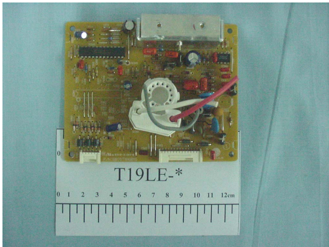
FIGURE 7 COLOR MONITOR (M/N:T19LE-*) CRT BOARD (COMPONENT SIDE)
