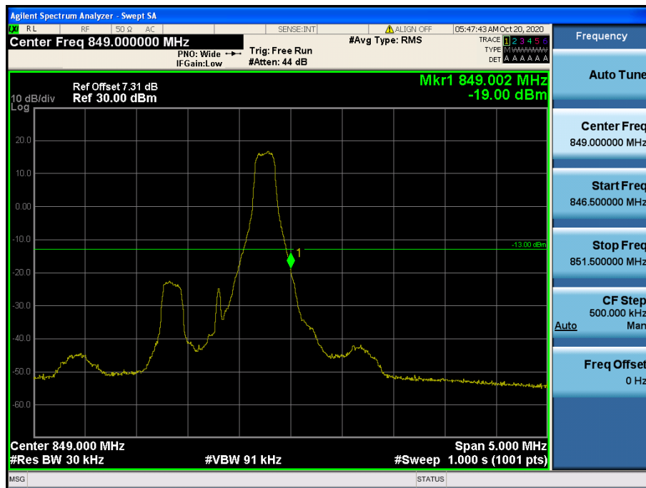
LTE Band 26 / 1.4 MHz / QPSK - RB Size/Offset (1/5)
