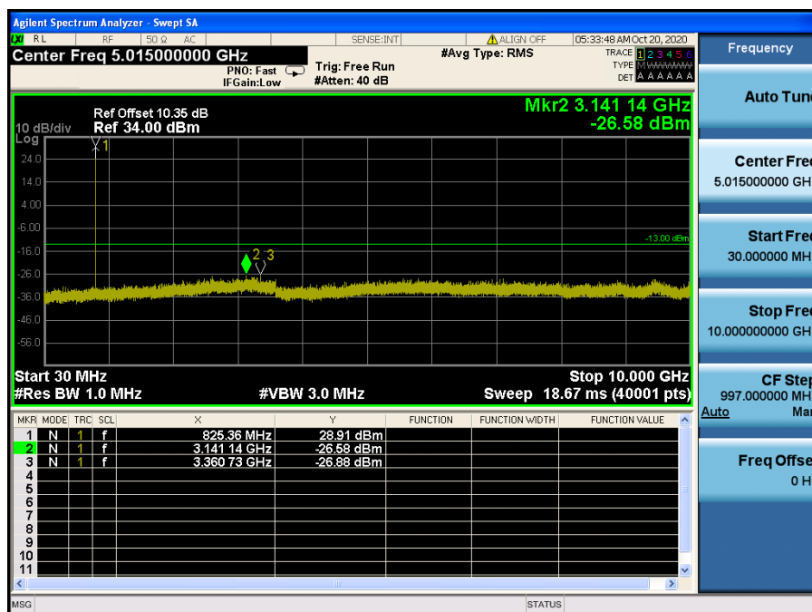
LTE Band 26(5) / 1.4 MHz / QPSK - RB Size/Offset (3/3) – Low Channel
