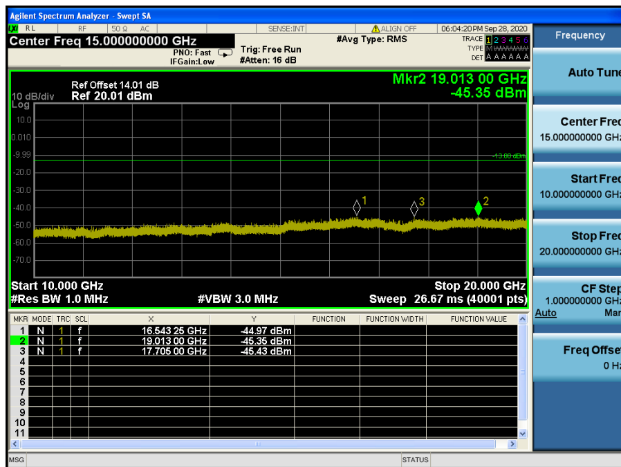
LTE Band 2 / 15 MHz / 16QAM - RB Size/Offset (36/0) – Mid Channel
