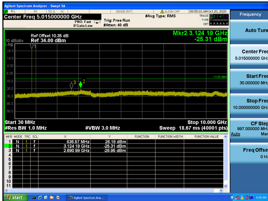
LTE Band 26(5) / 1.4 MHz / 16QAM - RB Size/Offset (6/0) – Mid Channel
