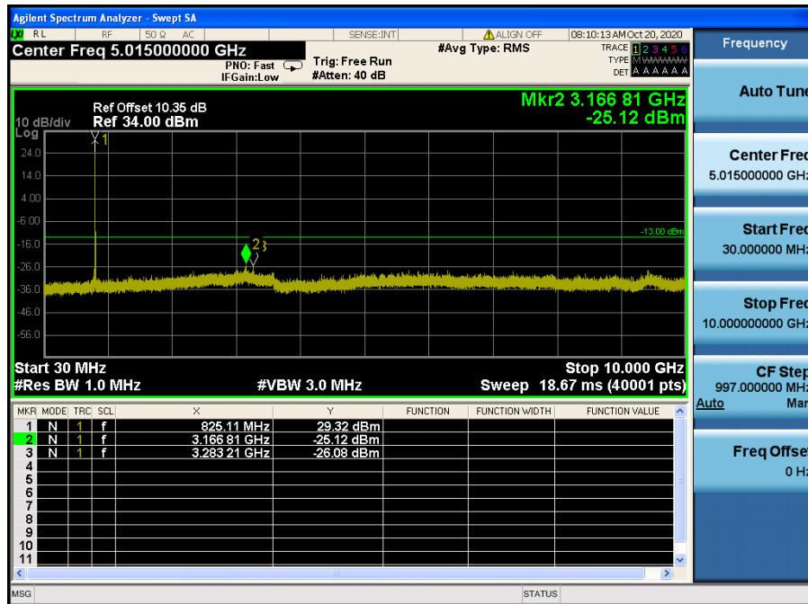
LTE Band 26 / 15 MHz / QPSK- RB Size/Offset (1/0) – Low Channel
