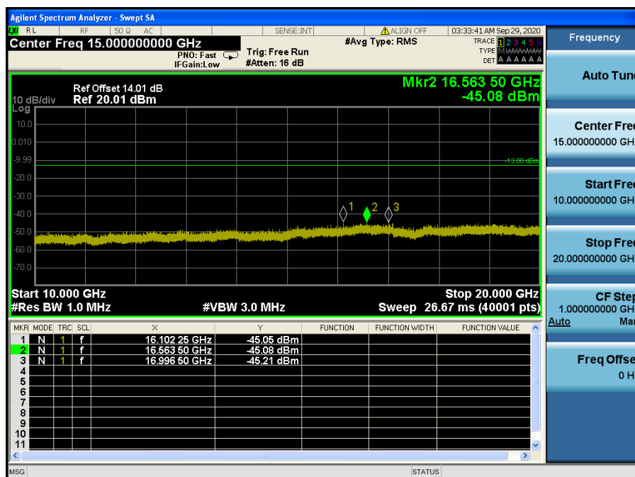
LTE Band 4 / 20 MHz / 16QAM - RB Size/Offset (1/99) –Low Channel
