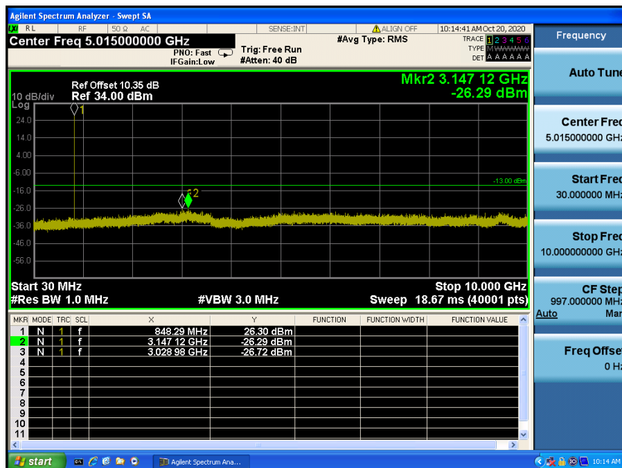
LTE Band 26(5) / 1.4 MHz / 16QAM - RB Size/Offset (6/0) – High Channel
