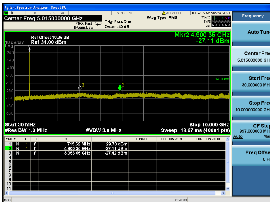
LTE Band 12 / 10 MHz / 16QAM - RB Size/Offset (1/49) – High Channel
