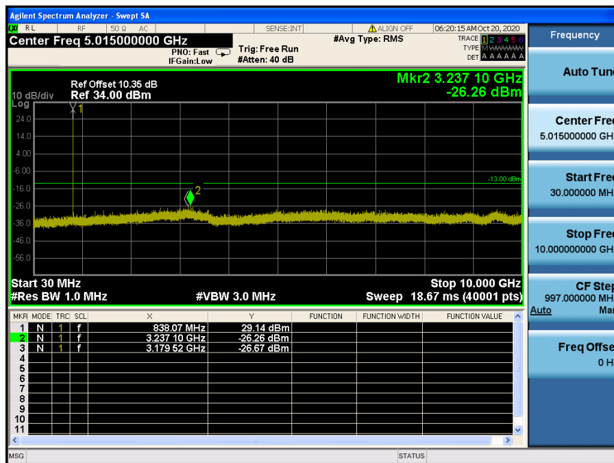
LTE Band 26(5) / 3 MHz / QPSK - RB Size/Offset (1/14) – Mid Channel
