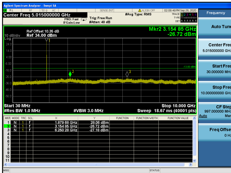
LTE Band 2 / 1.4 MHz / 16QAM - RB Size/Offset (1/0) – Mid Channel
