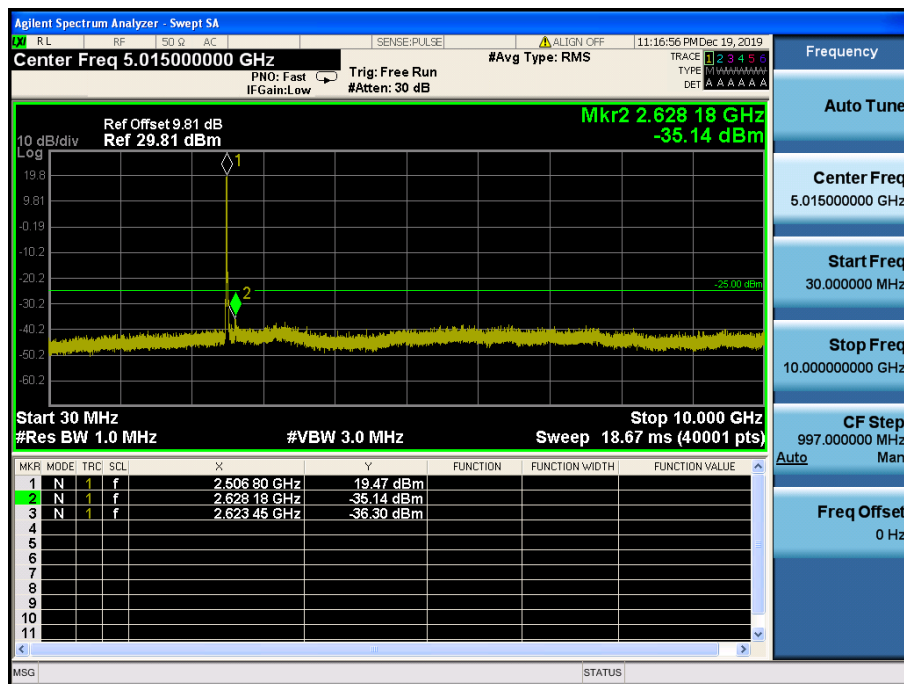
LTE Band 7 / 20MHz / 16QAM - RB Size/Offset (50/0) – Low Channel
