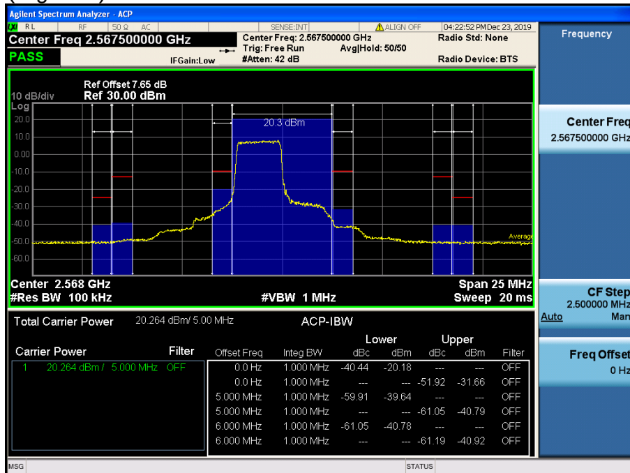
LTE Band 7 / 5MHz / QPSK - RB Size/Offset (12/0)
