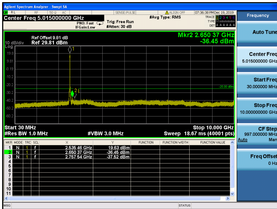
LTE Band 7 / 15MHz / QPSK - RB Size/Offset (75/0) – Mid Channel
