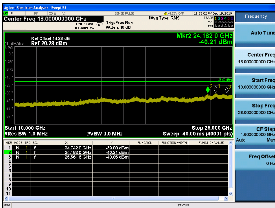
LTE Band 7 / 20MHz / 16QAM - RB Size/Offset (50/25) – Mid Channel
