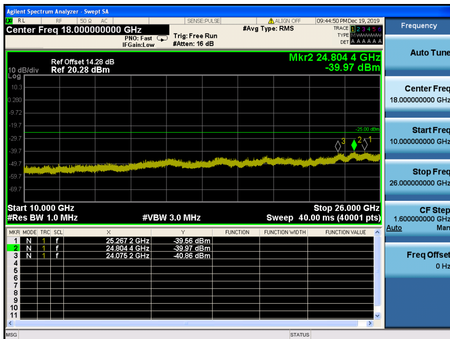
LTE Band 7 / 10MHz / 16QAM - RB Size/Offset (50/0) – Low Channel
