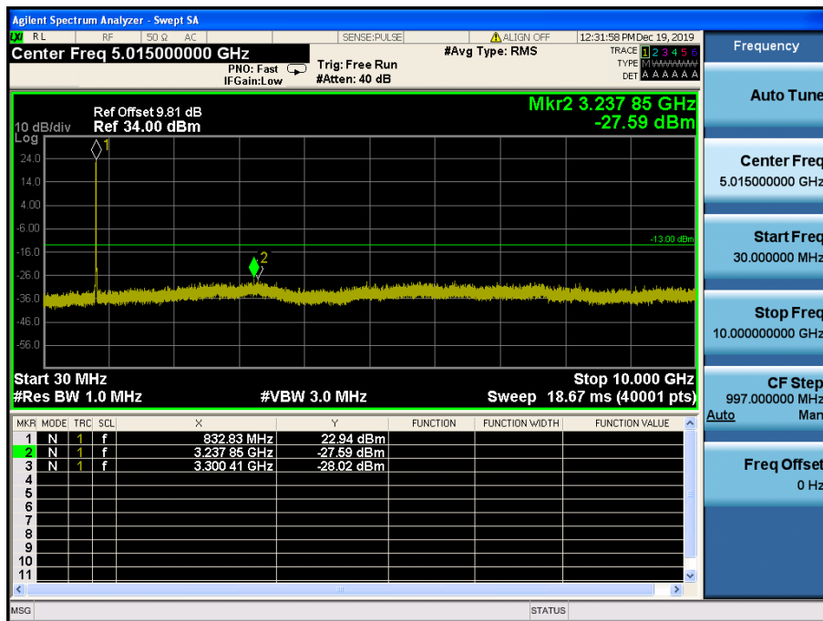
LTE Band 5 / 10MHz / QPSK - RB Size/Offset (25/25) – Low Channel
