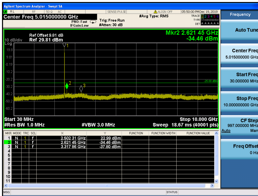
LTE Band 7 / 5MHz / QPSK - RB Size/Offset (12/6) – Low Channel
