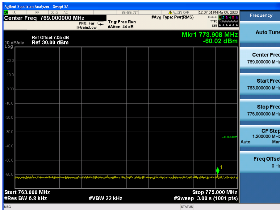
LTE Band 13 / 10MHz / 16QAM - RBSize/Offset (1/25)
