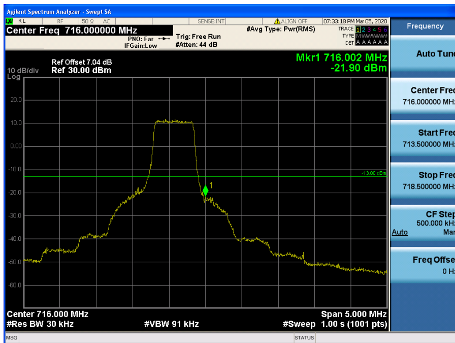
LTE Band 12,17 / 1.4MHz / QPSK - RB Size/Offset (3/3)
