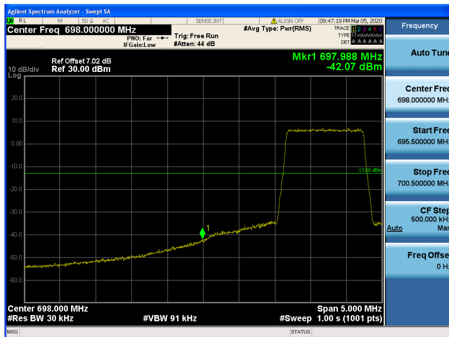
LTE Band 12,17 / 1.4MHz / 16QAM - RB Size/Offset (6/0)
