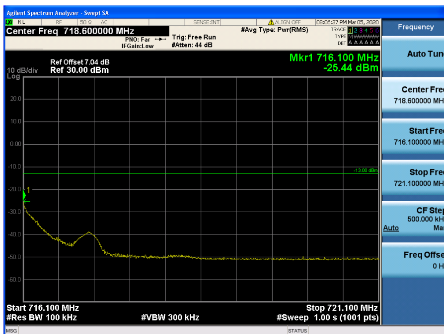
LTE Band 12,17 / 3MHz / QPSK - RB Size/Offset (1/14)
