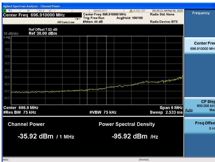
LTE Band 12,17 / 10MHz / 16QAM - RB Size/Offset (25/12)
