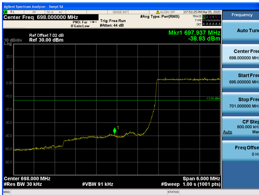
LTE Band 12,17 / 3MHz / QPSK - RB Size/Offset (15/0)
