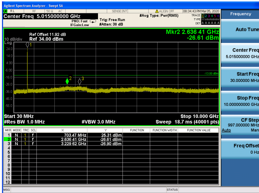
LTE Band 12,17 / 5MHz / QPSK - RB Size/Offset (25/0) – Low Channel
