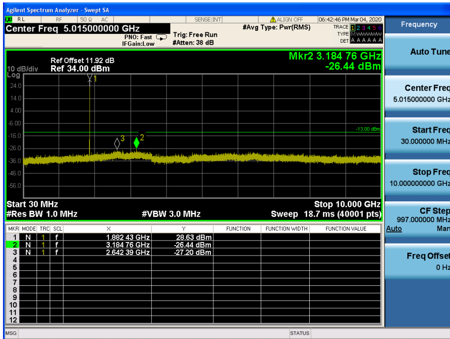
LTE Band 2 / 5MHz / 16QAM - RB Size/Offset (1/24) – Mid Channel
