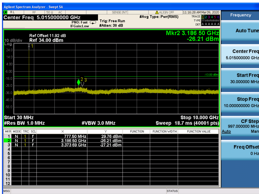
LTE Band 13 / 5MHz / 16QAM - RB Size/Offset (1/0) – Low Channel
