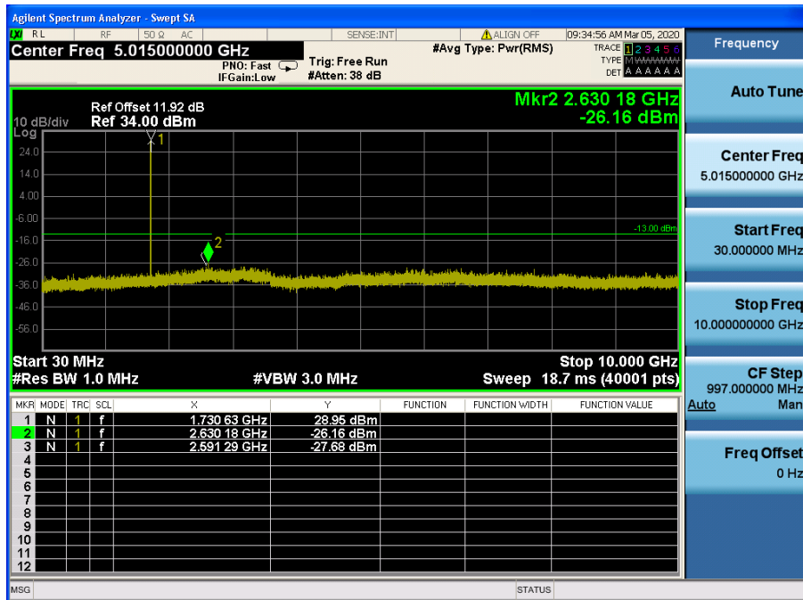
LTE Band 4 / 5MHz / QPSK - RB Size/Offset (1/0) – Mid Channel
