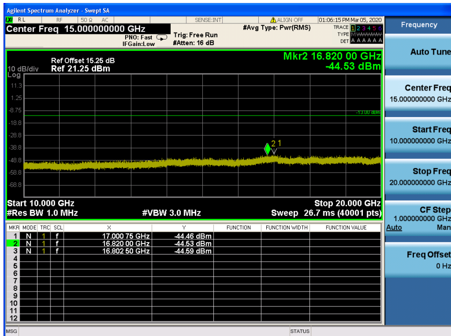
LTE Band 4 / 1.4MHz / 16QAM - RB Size/Offset (3/2) – Mid Channel
