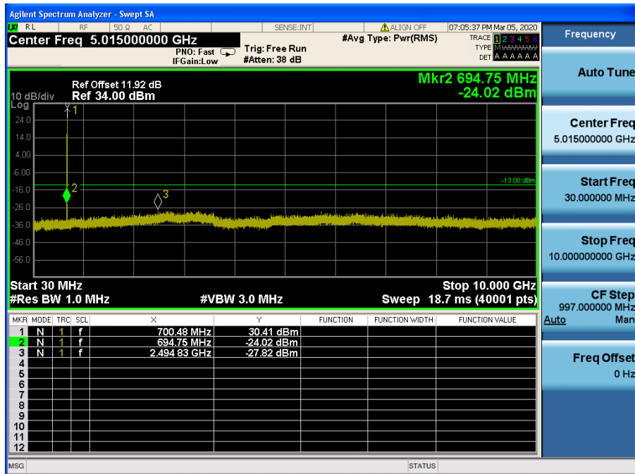
LTE Band 12 / 1.4MHz / QPSK - RB Size/Offset (1/5) – Low Channel
