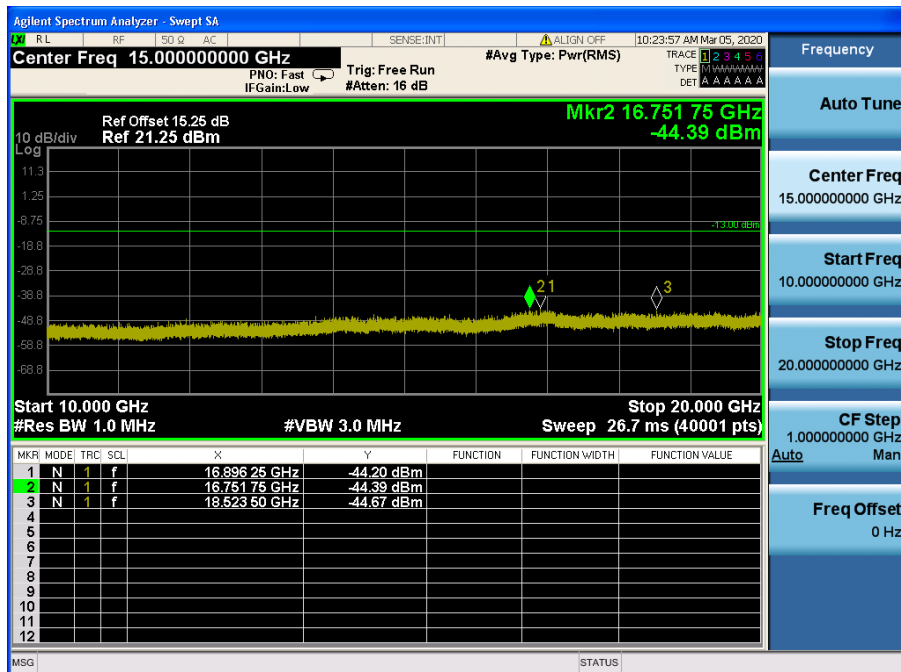
LTE Band 4 / 10MHz / QPSK - RB Size/Offset (1/49) – Mid Channel
