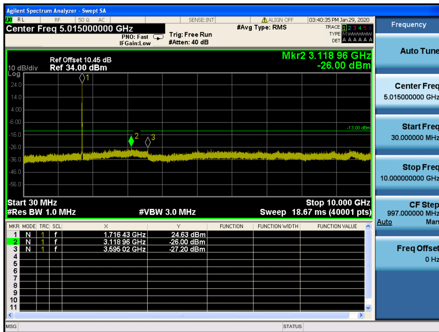
LTE Band 4 / 15MHz / QPSK - RB Size/Offset (36/0)–Low Channel
