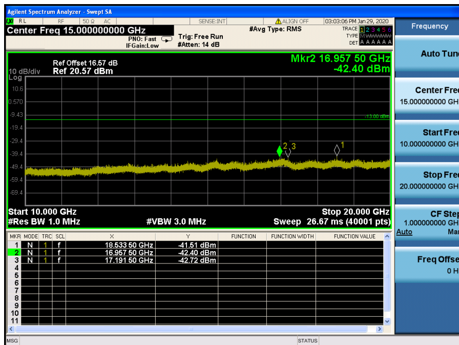
LTE Band 4 / 10MHz / QPSK - RB Size/Offset (25/0) – Mid Channel
