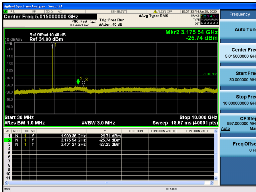
LTE Band 2 / 15MHz / QPSK - RB Size/Offset (1/74) – High Channel
