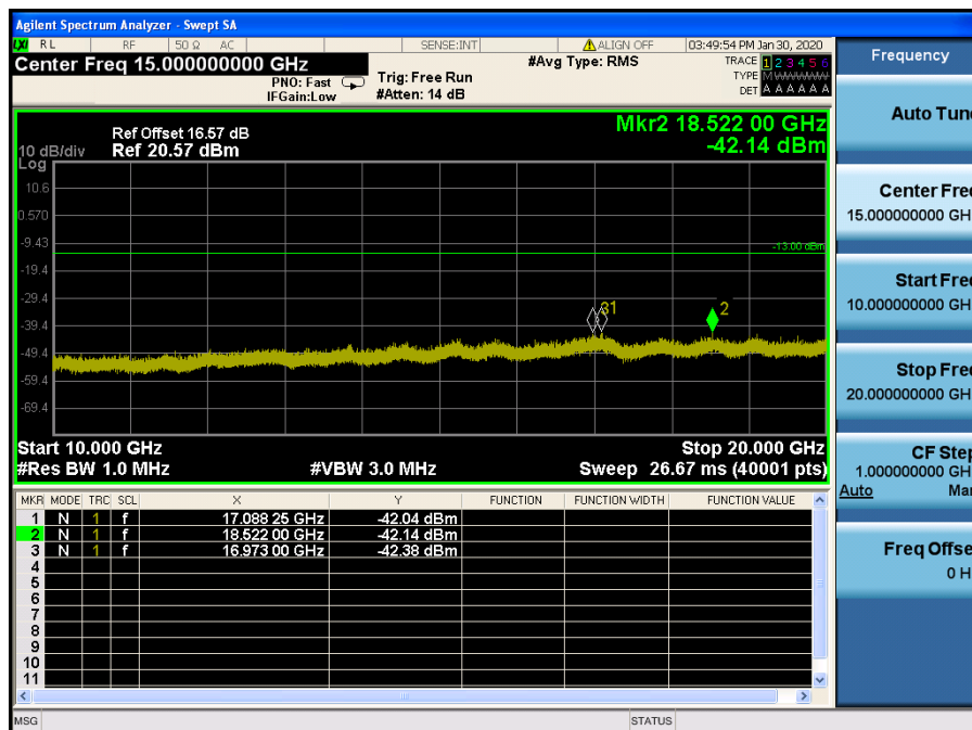
LTE Band 4 / 1.4MHz / 16QAM - RB Size/Offset (1/0) – High Channel
