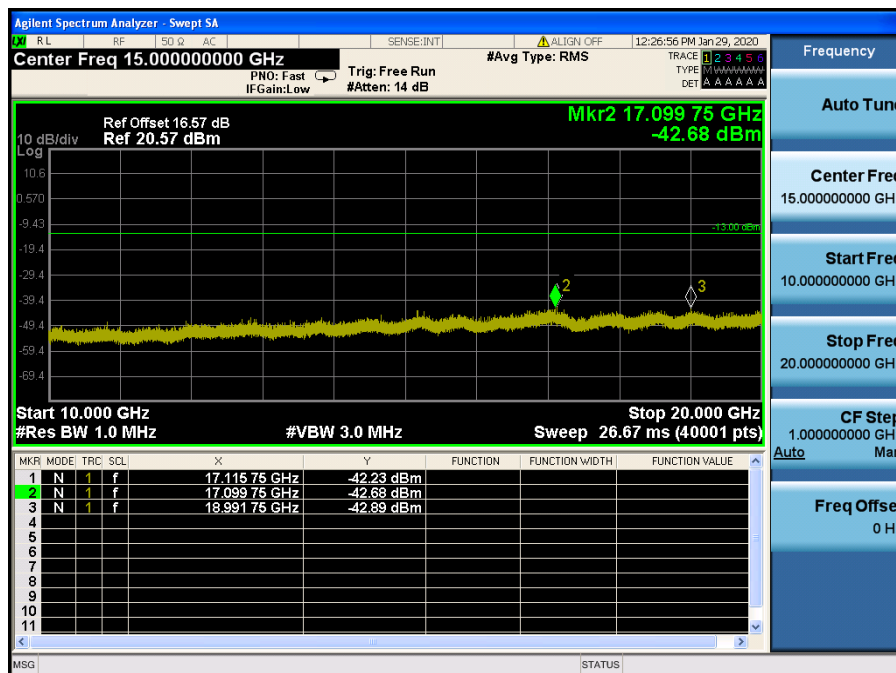
LTE Band 4 / 1.4MHz / QPSK - RB Size/Offset (3/3) – Mid Channel
