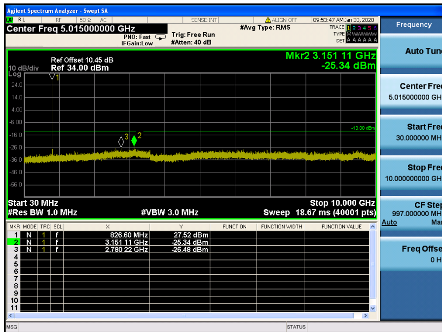
LTE Band 5 / 3MHz / QPSK - RB Size/Offset (8/7) – Low Channel
