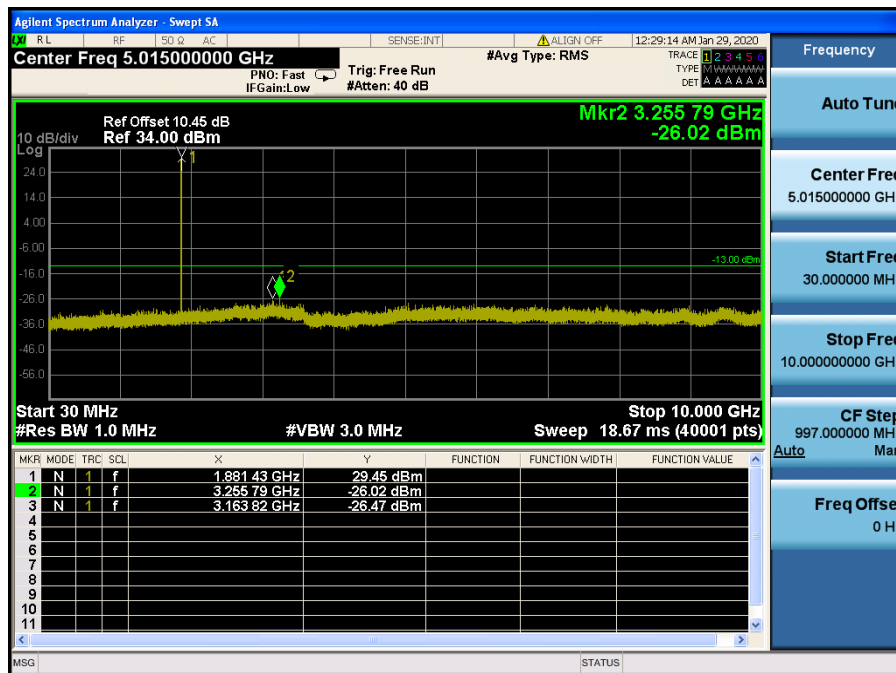
LTE Band 2 / 3MHz / 16QAM - RB Size/Offset (1/14) – Mid Channel
