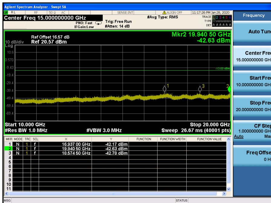
LTE Band 2 / 1.4MHz / 16QAM - RB Size/Offset (1/2) – Low Channel
