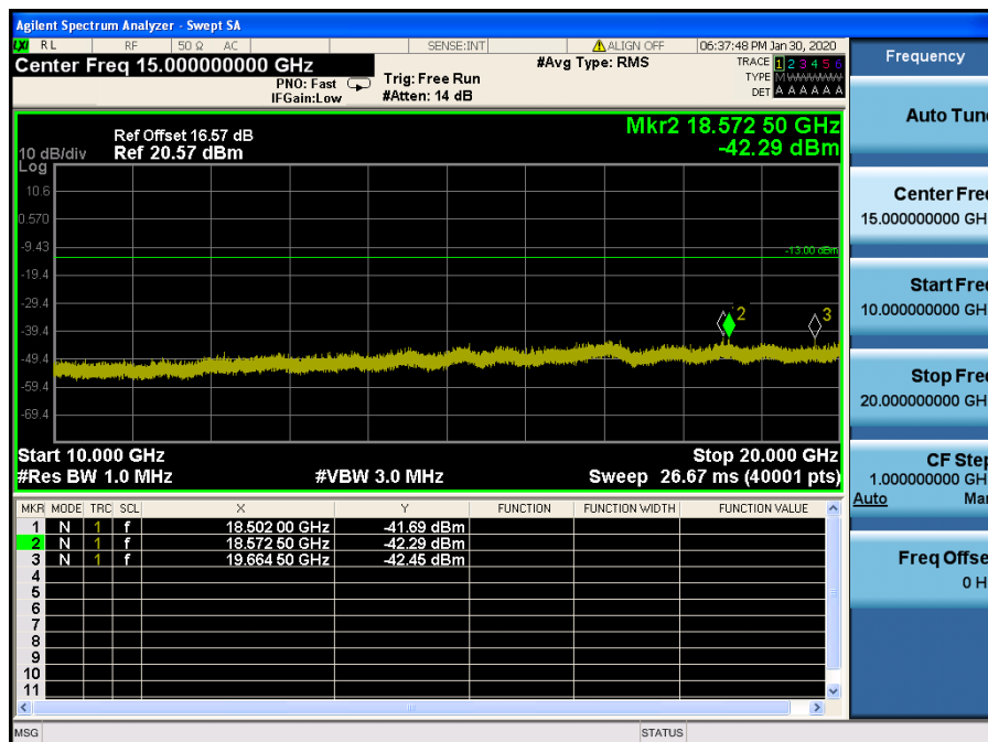
LTE Band 4 / 10MHz / 16QAM - RB Size/Offset (25/12) – High Channel
