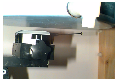
Figure 20. Body SAR Test Setup
