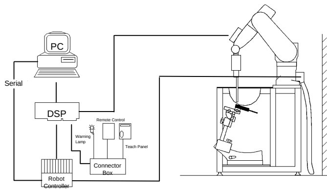
Figure 3. PCTEST SAR Lab II Test Measurement Set-up
