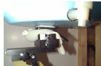
Figure 24. Hand SAR Test Setup
