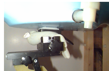
Figure 25. Hand SAR Test Setup
