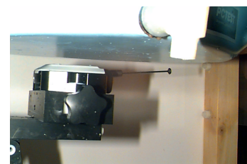
Figure 22. Body SAR Test Setup
