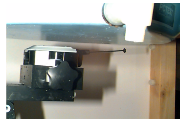
Figure 21. Body SAR Test Setup
