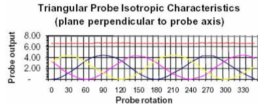
Figure 3.3 Probe Characteristics
