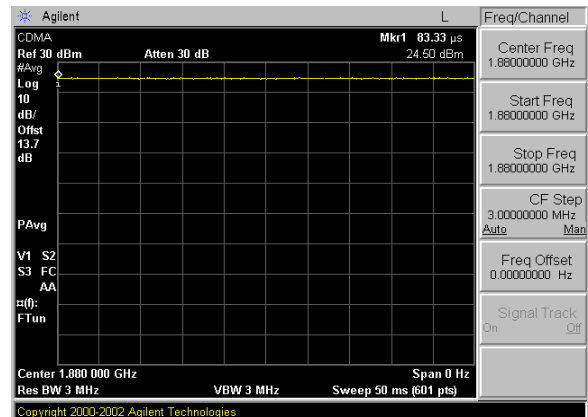
Figure 8-3 Modulation Factors
