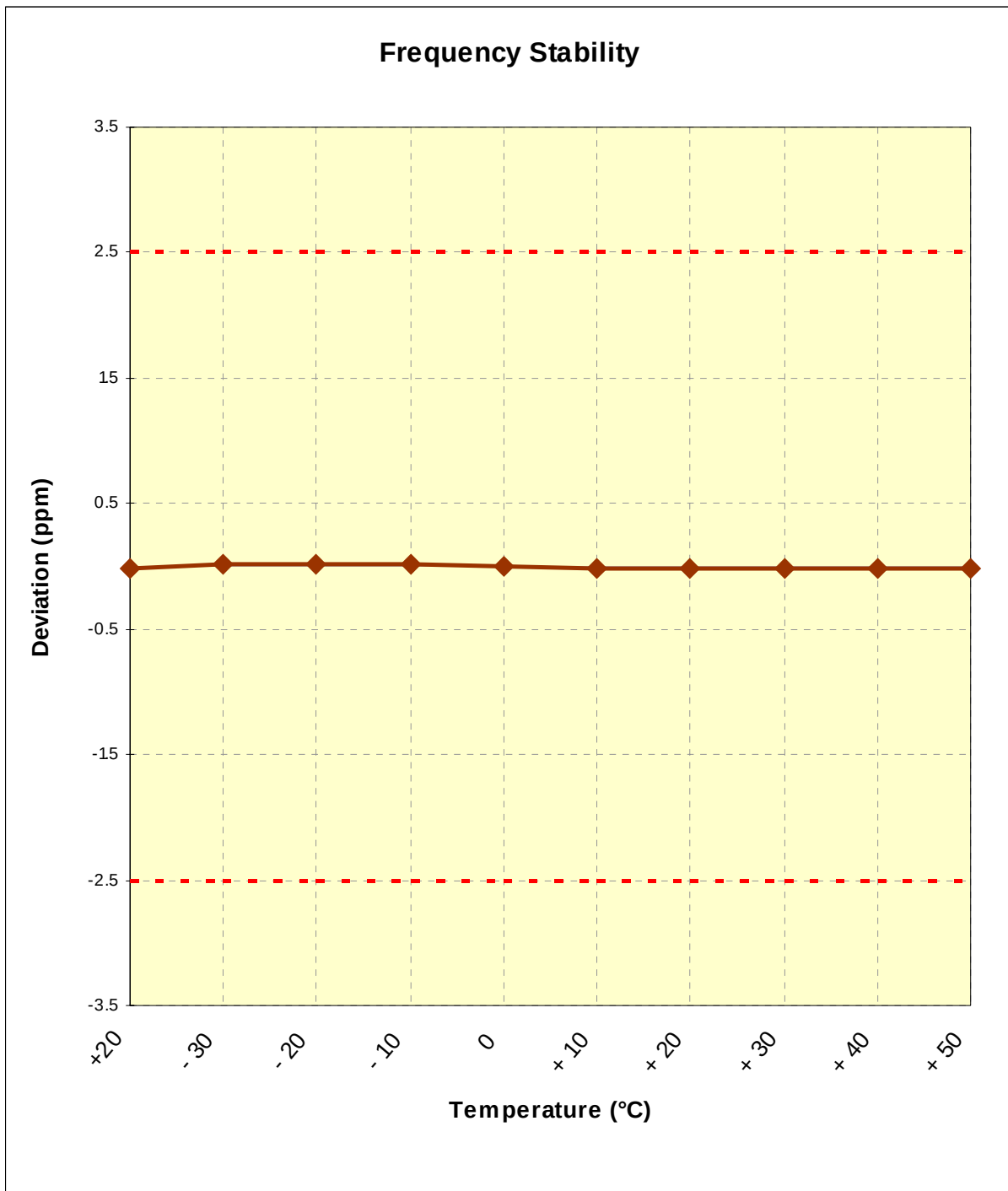
Figure 6-1. Frequency Stability Graph (AWS CDMA Mode – Ch. 450)
