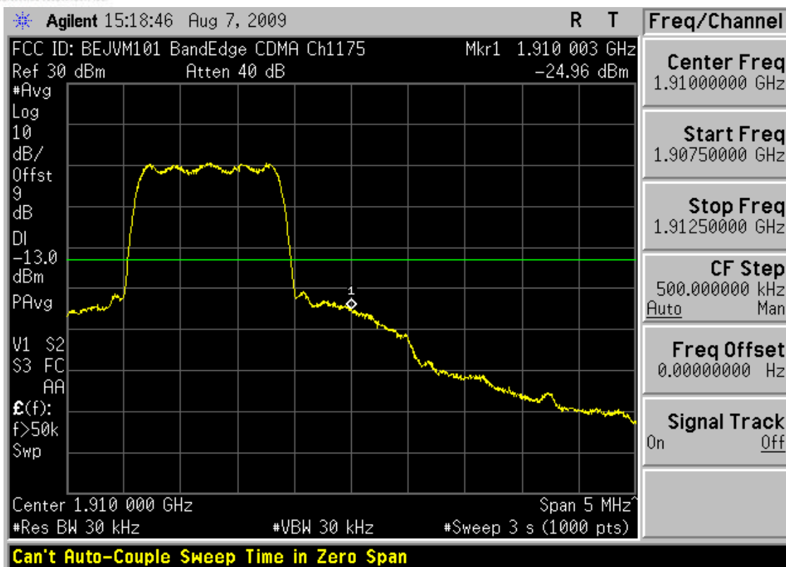
Plot 7-11. Band Edge Plot (PCS CDMA Mode – Ch. 1175)
