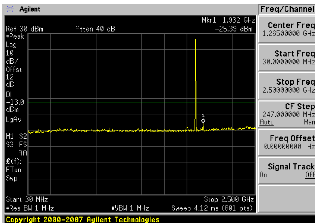
Plot 7-1. Conducted Spurious Plot (PCS CDMA Mode – Ch. 25)
