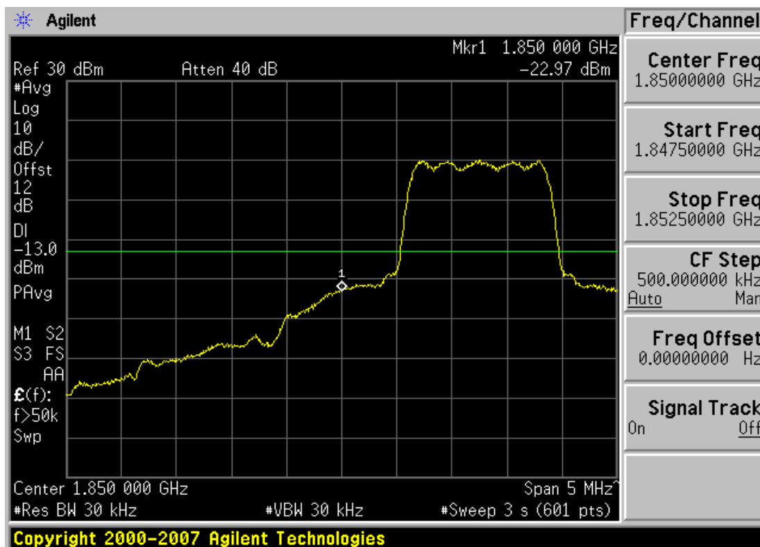
Plot 7-3. Band Edge Plot (PCS CDMA Mode – Ch. 25)
