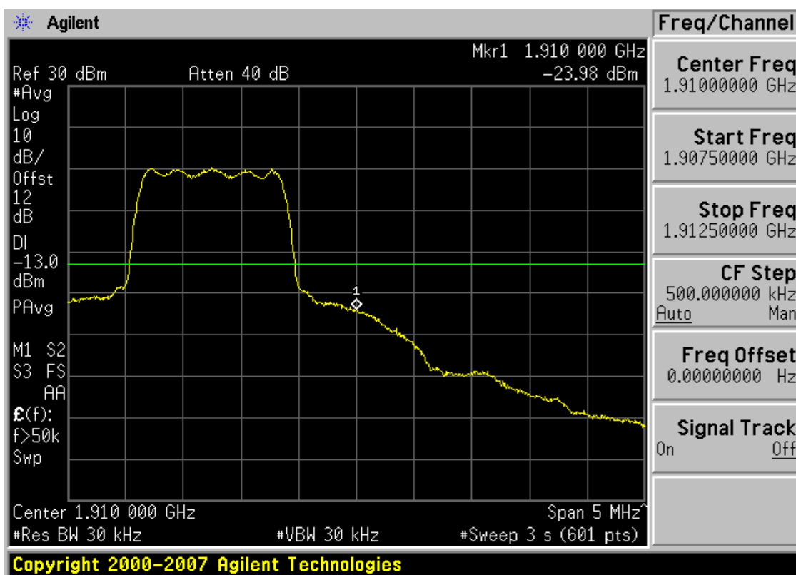
Plot 7-11. Band Edge Plot (PCS CDMA Mode – Ch. 1175)
