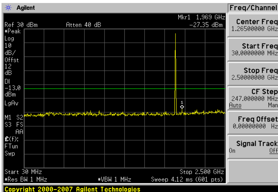
Plot 7-9. Conducted Spurious Plot (PCS CDMA Mode – Ch. 1175)
