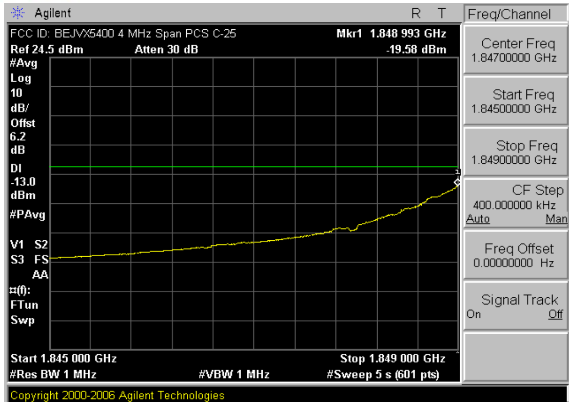
Plot 7-28. 4MHz Span Plot (PCS CDMA Mode - Ch. 25)
