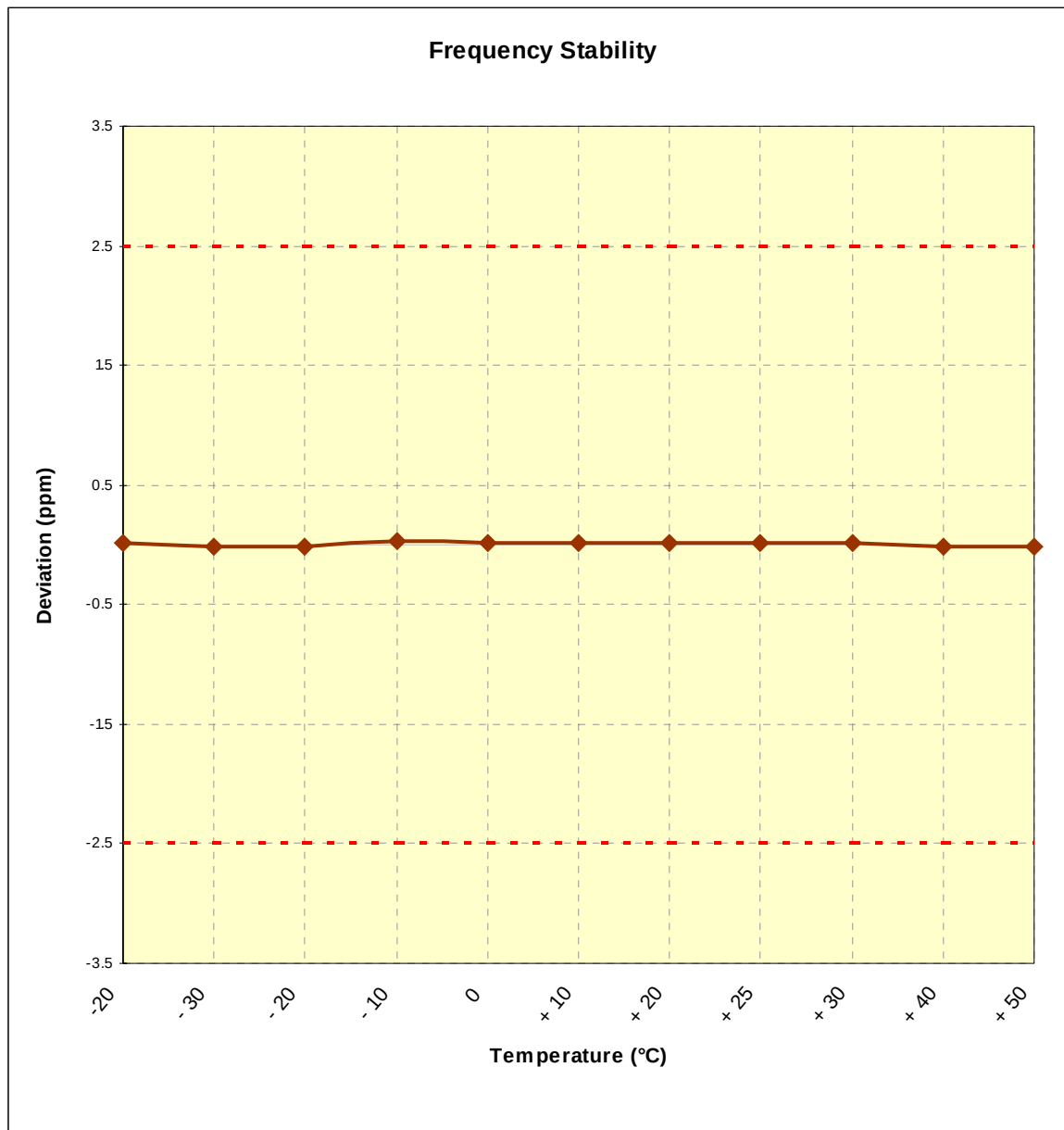
Figure 6-3. Frequency Stability Graph (Cellular CDMA Mode – Ch. 384)
