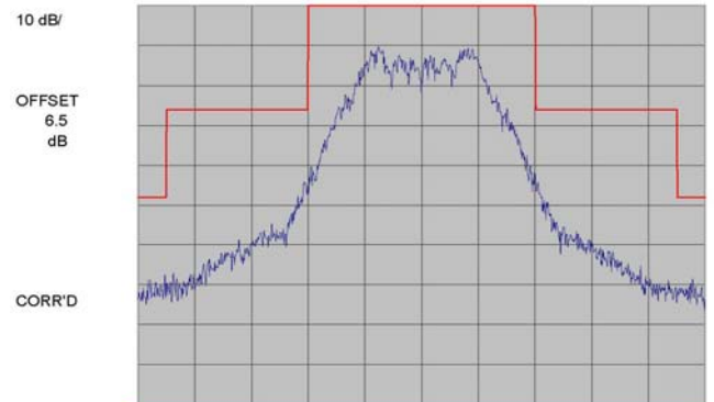
Plot 7-14. SAT + DTMF
