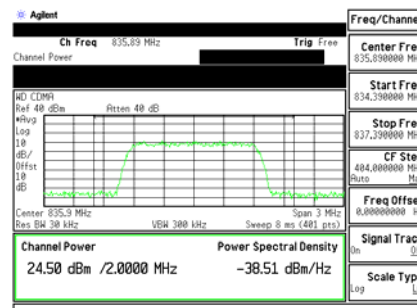
Figure 8-2 Wireless Device Modulated Signal
