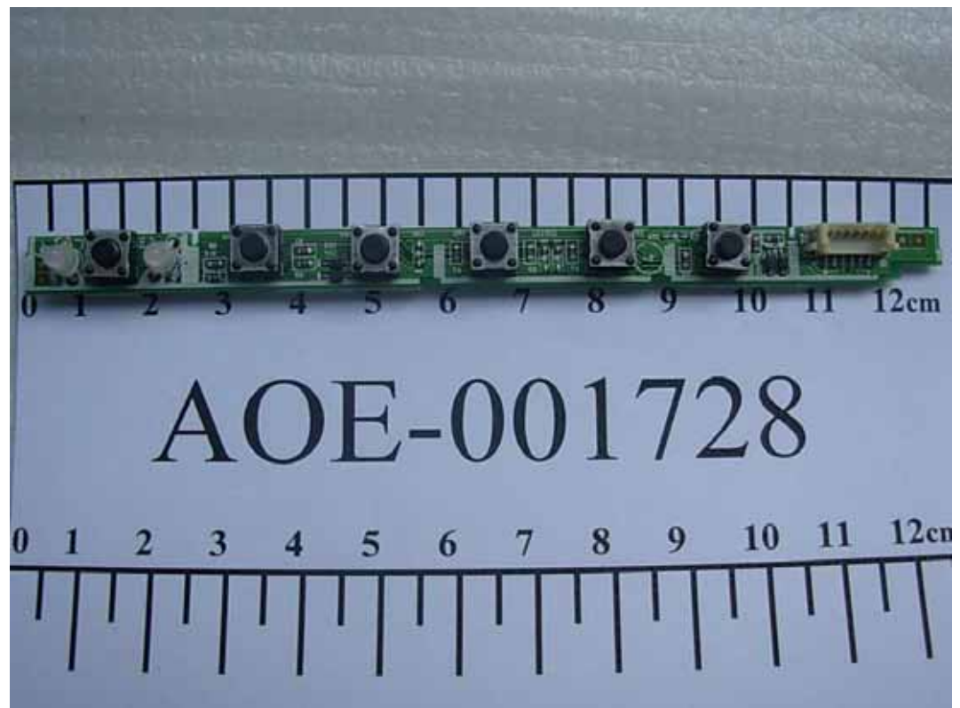
FIGURE 3 LCD MONITOR (M/N: W1642ST) BUTTON BOARD (COMPONENT SIDE)
