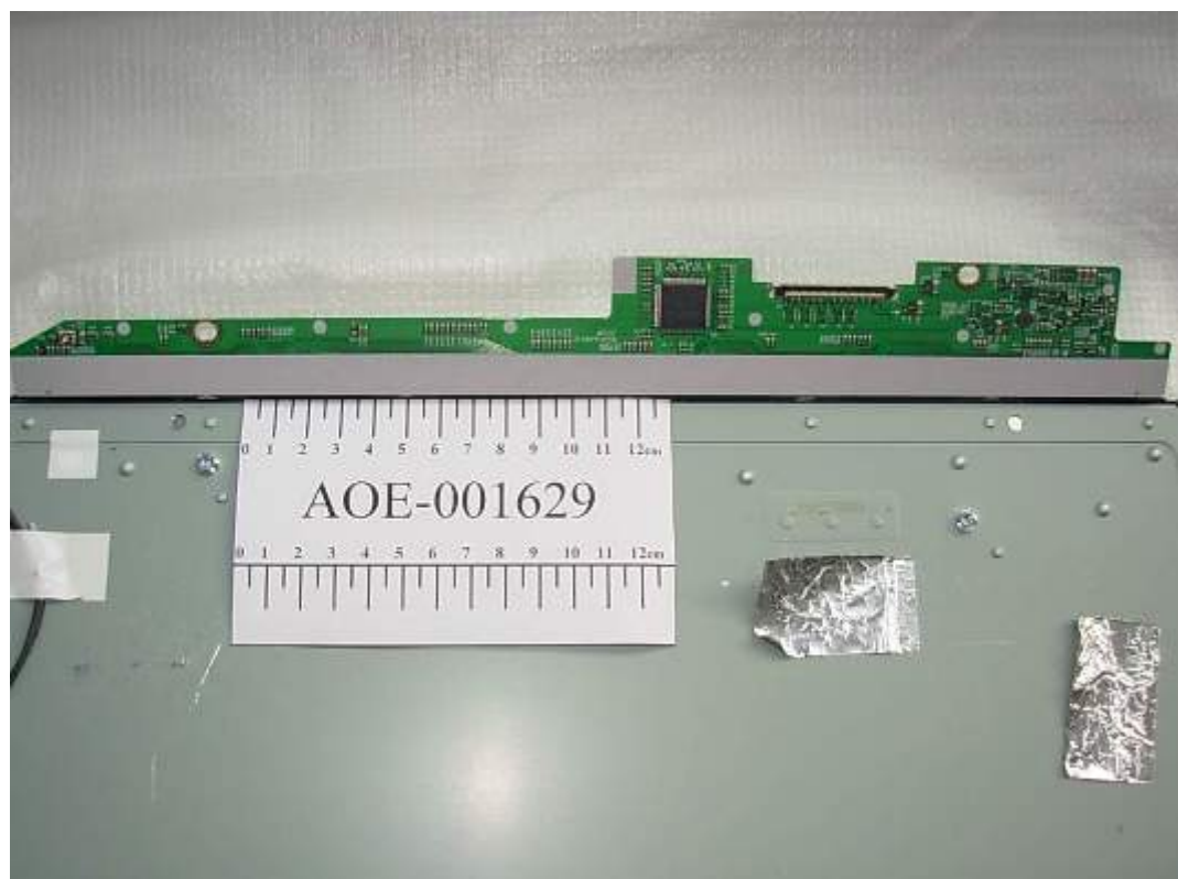
FIGURE 16 LCD MONITOR (M/N: W1752TT) LCD PANEL MAIN BOARD BACK
