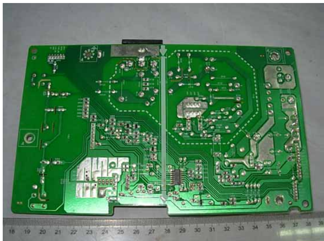
FIGURE 4 LCD MONITOR (M/N: W1946PW) POWER BOARD (COMPONENT SIDE)
