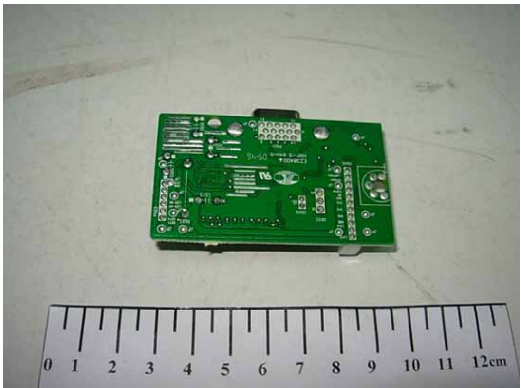
FIGURE 6 LCD MONITOR (M/N: W2040SV) MAIN BOARD (SOLDERED SIDE)
