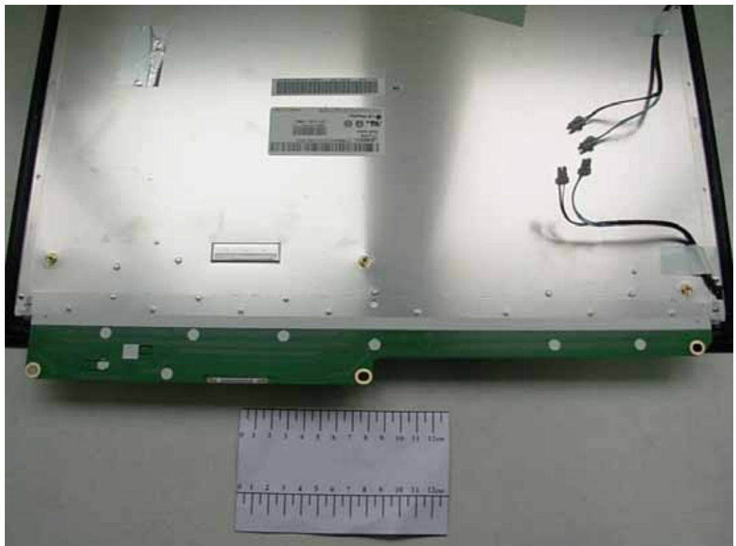
FIGURE 12 LCD MONITOR (M/N: W2040SV) LCD PANEL MAIN BOARD (SOLDERED SIDE)
