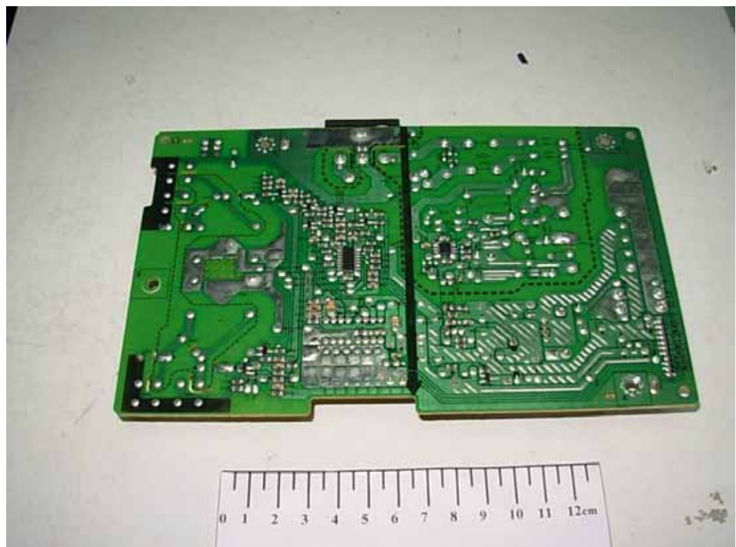
FIGURE 9 LCD MONITOR (M/N: W2040SV) POWER BOARD (SOLDERED SIDE)
