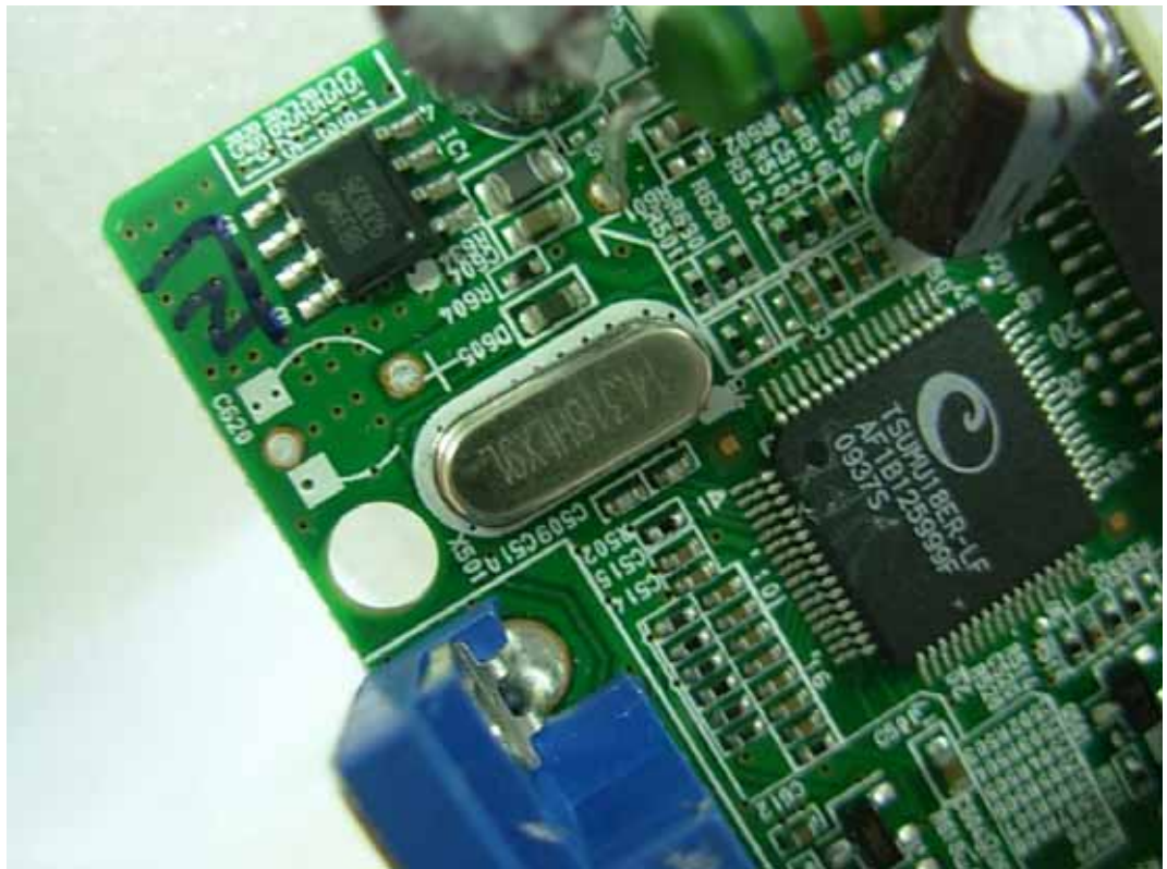
FIGURE 7 LCD MONITOR (M/N: W2040SV) CHIP & CRYSTAL ON MAIN BOARD
