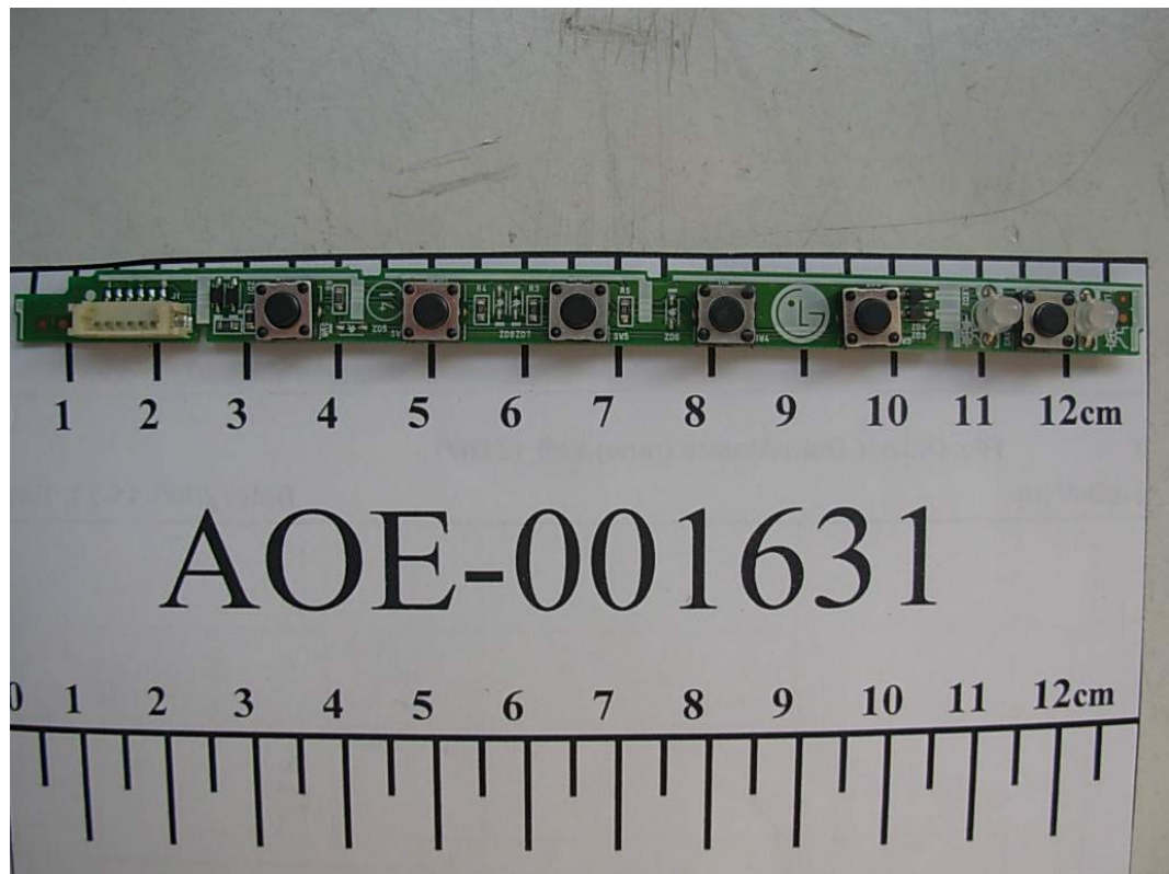
FIGURE 3 LCD MONITOR (M/N: W2042TT) BOTTOM BOARD (COMPONENT SIDE)
