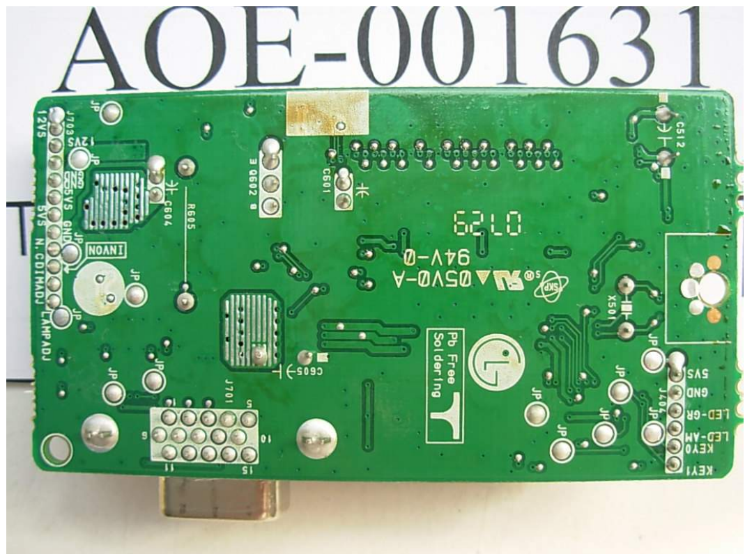
FIGURE 26 LCD MONITOR (M/N: W2042ST) MAIN BOARD (SOLDERED SIDE)
