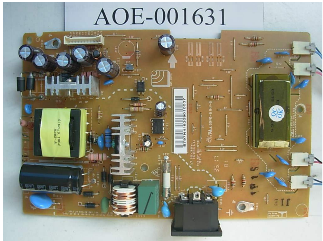
FIGURE 5 LCD MONITOR (M/N: W2042TT) POWER BOARD (COMPONENT SIDE)
