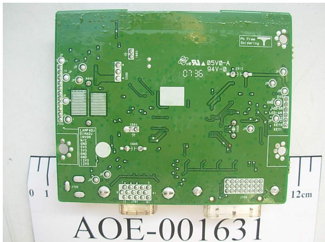
FIGURE 8 LCD MONITOR (M/N: W2042TT) MAIN BOARD (SOLDERED SIDE)
