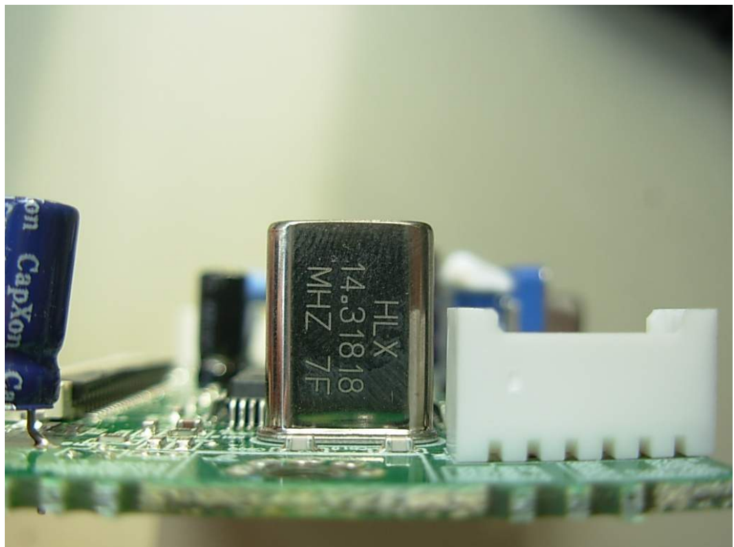
FIGURE 28 LCD MONITOR (M/N: W2042ST) CRYSTAL ON MAIN BOARD
