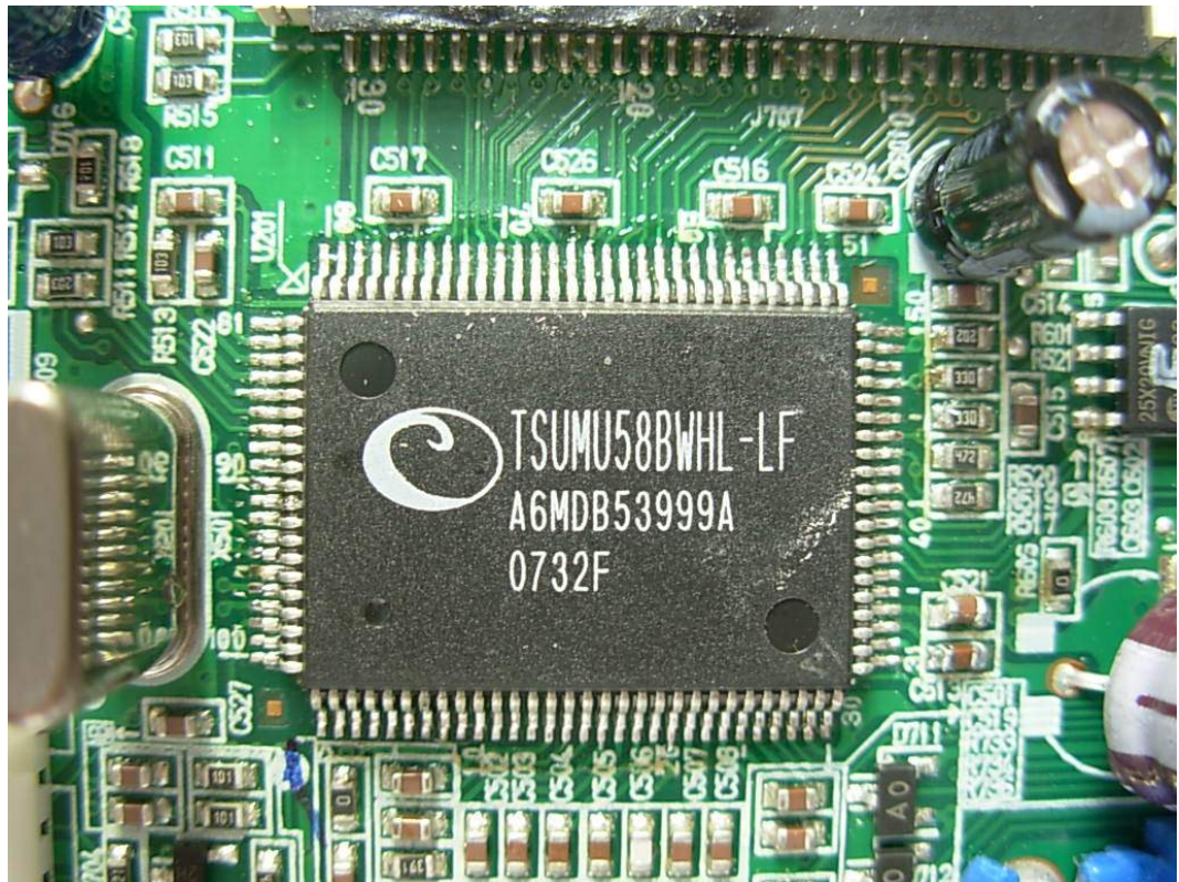
FIGURE 27 LCD MONITOR (M/N: W2042ST) CHIP ON MAIN BOARD
