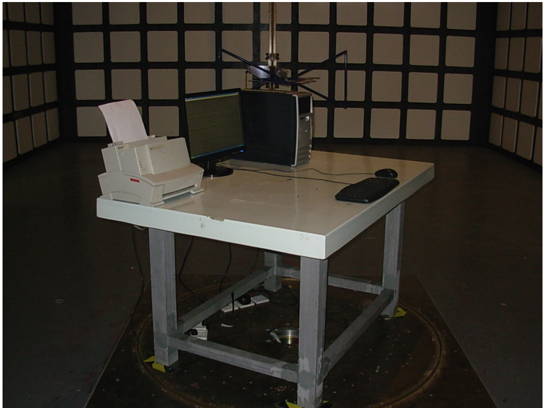
SETUP WITH MAXIMUM DETECTED EMISSION AT HORIZONTAL POLARIZATION (VGA 1680*1050@60Hz, BELOW 1GHz) (M/N: W2042ST)
