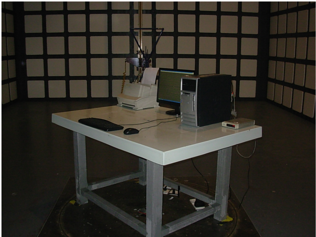
SETUP WITH MAXIMUM DETECTED EMISSION AT VERTICAL POLARIZATION (VGA1680*1050@60Hz, BELOW 1GHz) (M/N: W2042ST)
