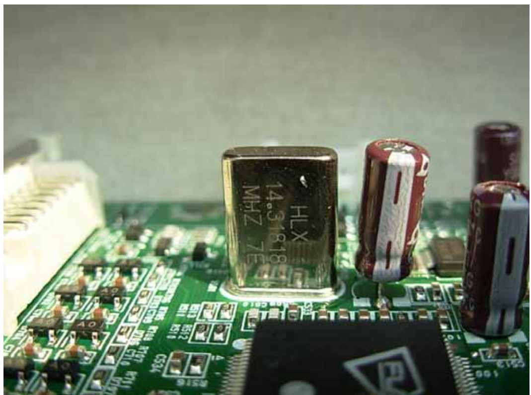
FIGURE 10 LCD MONITOR (M/N: W2052TQT) CRYSTAL ON MAIN BOARD
