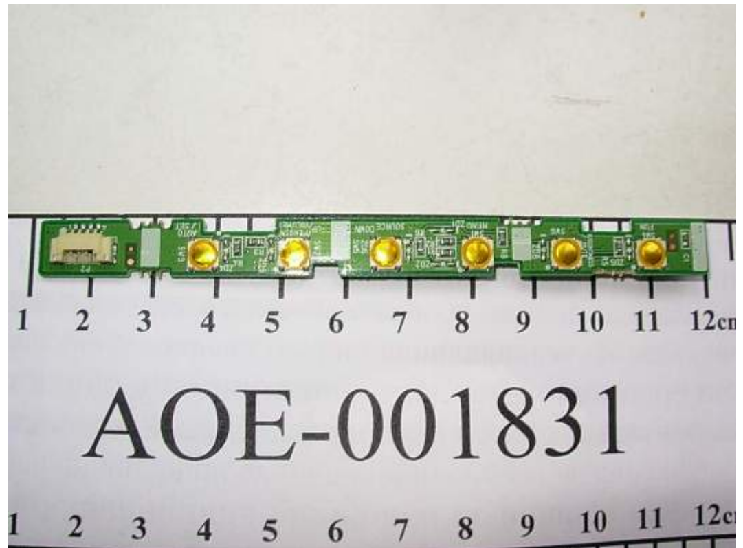
FIGURE 17 LCD MONITOR (M/N: W2052VQT) BUTTON BOARD (COMPONENT SIDE)
