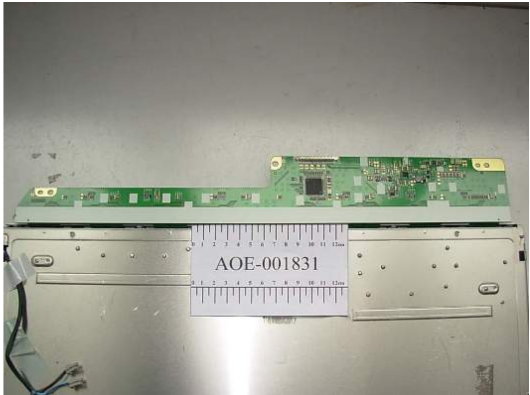
FIGURE 12 LCD MONITOR (M/N: W2052VQT) LCD PANEL MAIN BOARD (COMPONENT SIDE)
