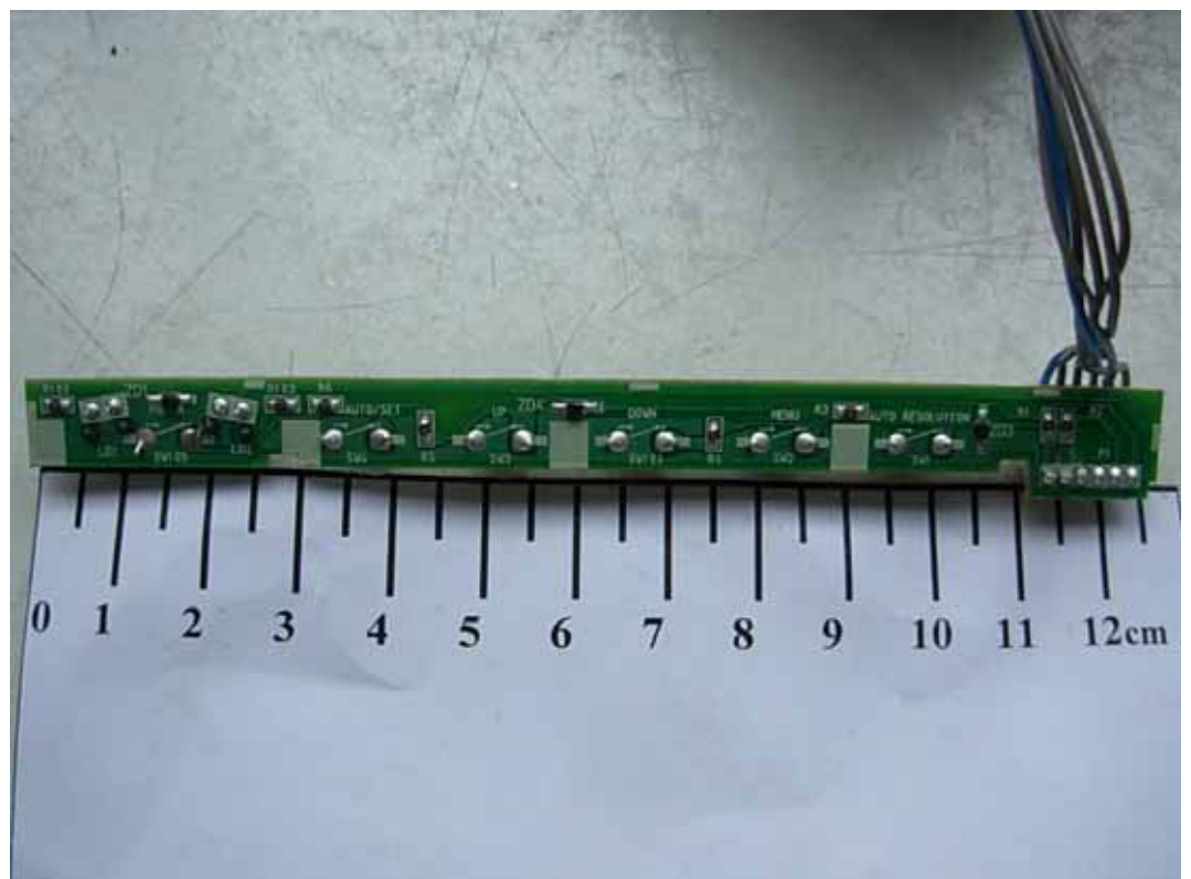
FIGURE 4 LCD MONITOR (M/N: W2240SV) KEY BOARD (SOLDERED SIDE)
