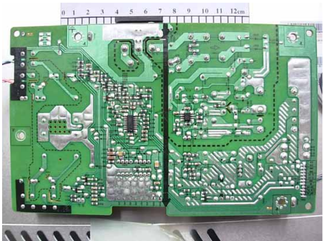
FIGURE 9 LCD MONITOR (M/N: W2240SV) POWER BOARD (SOLDERED SIDE)
