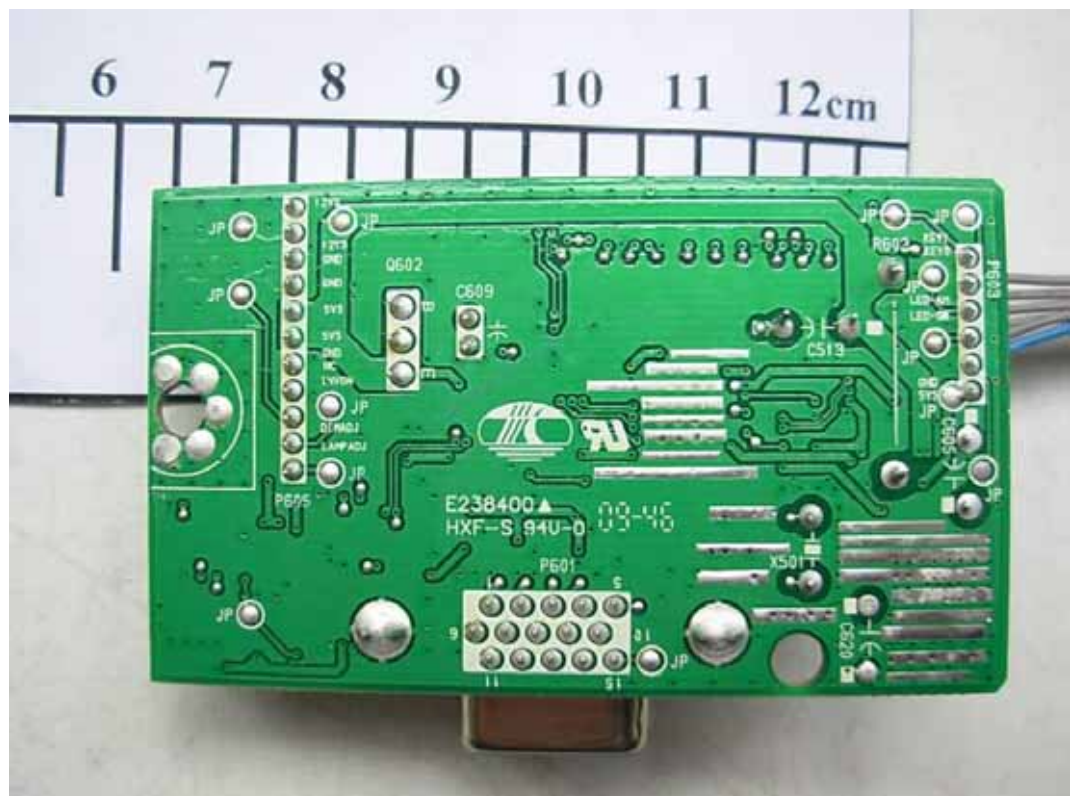
FIGURE 6 LCD MONITOR (M/N: W2240SV) MAIN BOARD (SOLDERED SIDE)
