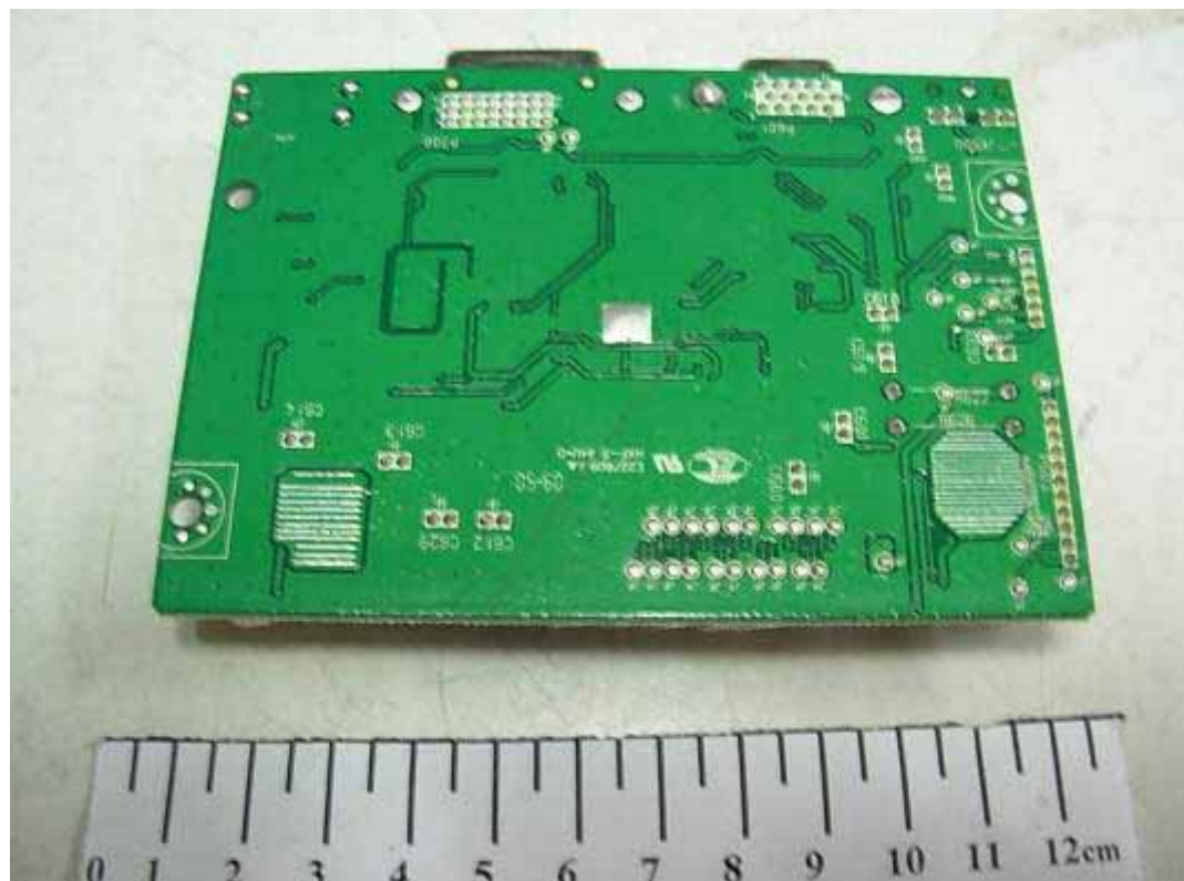
FIGURE 4 LCD MONITOR (M/N: W2240VV) MAIN BOARD (SOLDERED SIDE)
