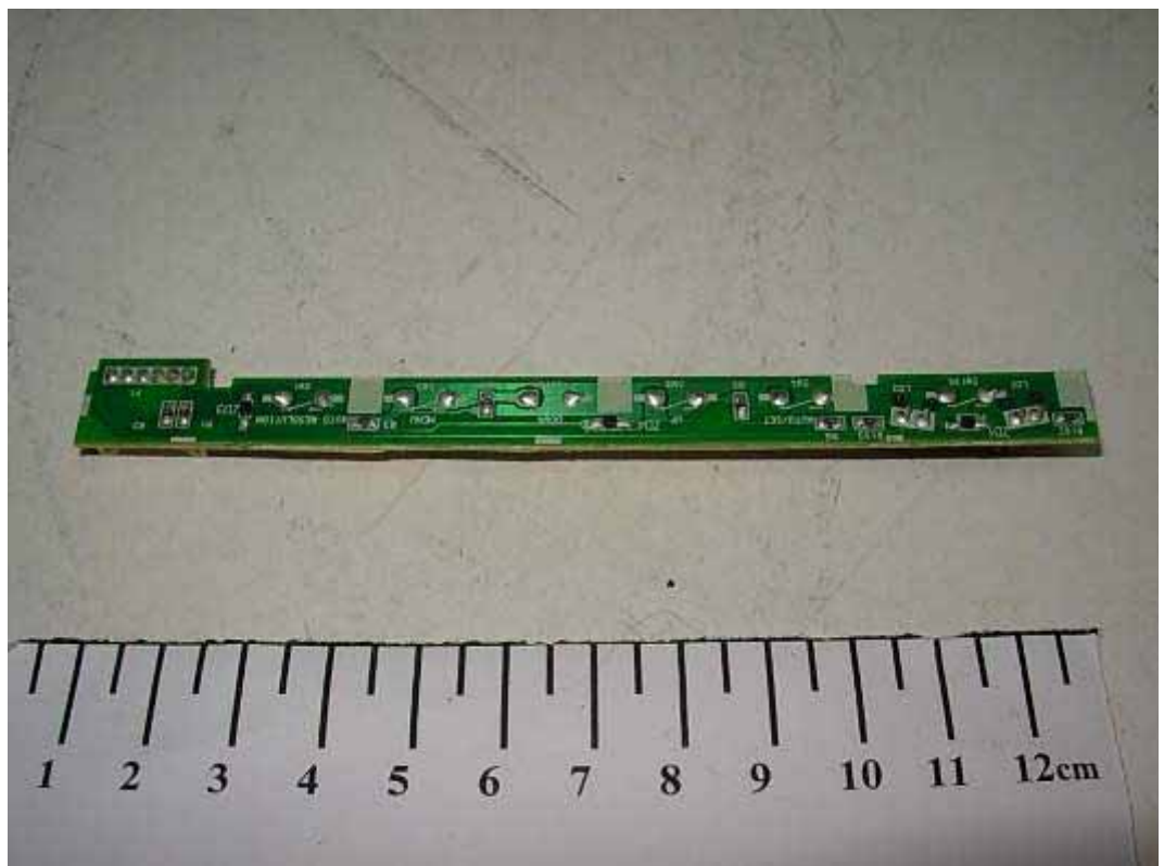
FIGURE 9 LCD MONITOR (M/N: W2240VV) KEY BOARD (SOLDERED SIDE)
