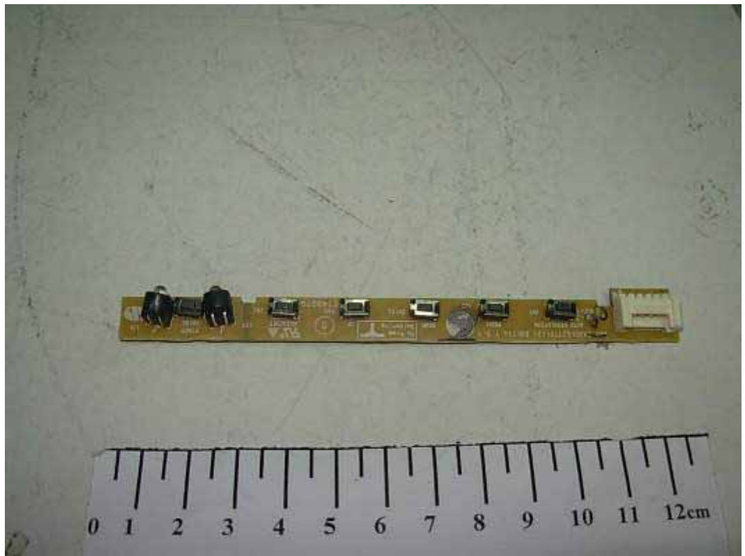
FIGURE 8 LCD MONITOR (M/N: W2240VV) KEY BOARD (COMPONENT SIDE)
