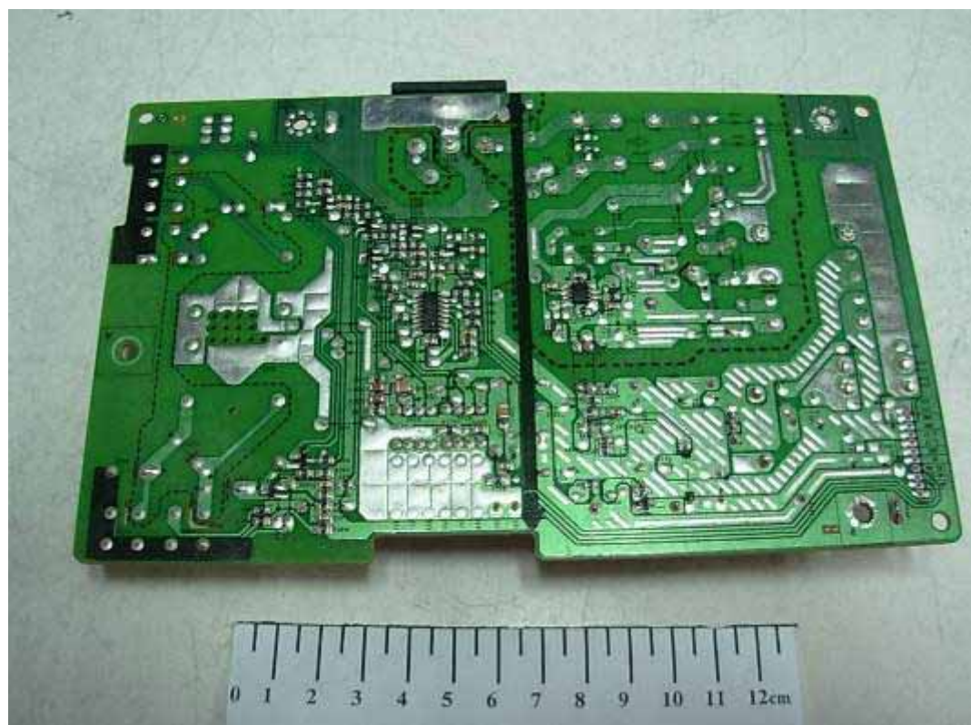
FIGURE 7 LCD MONITOR (M/N: W2240VV) POWER BOARD (SOLDERED SIDE)
