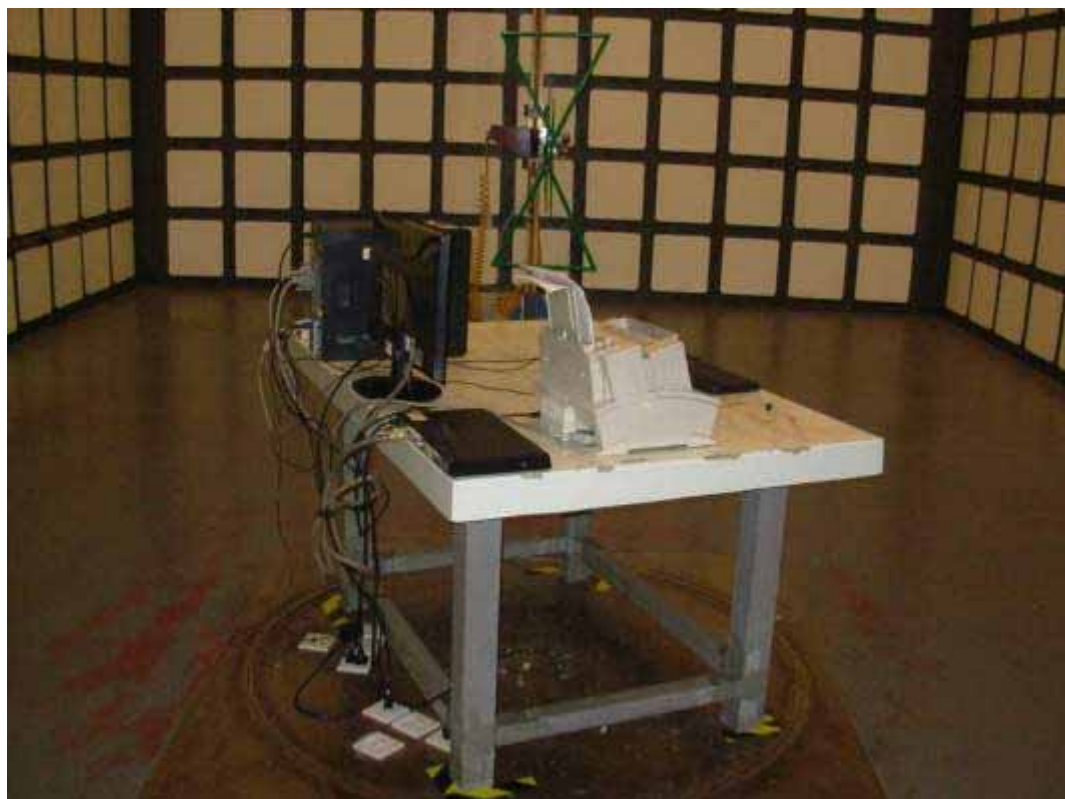
SETUP WITH MAXIMUM DETECTED EMISSION AT VERTICAL POLARIZATION (TEST MODE: HDMI 720P)
