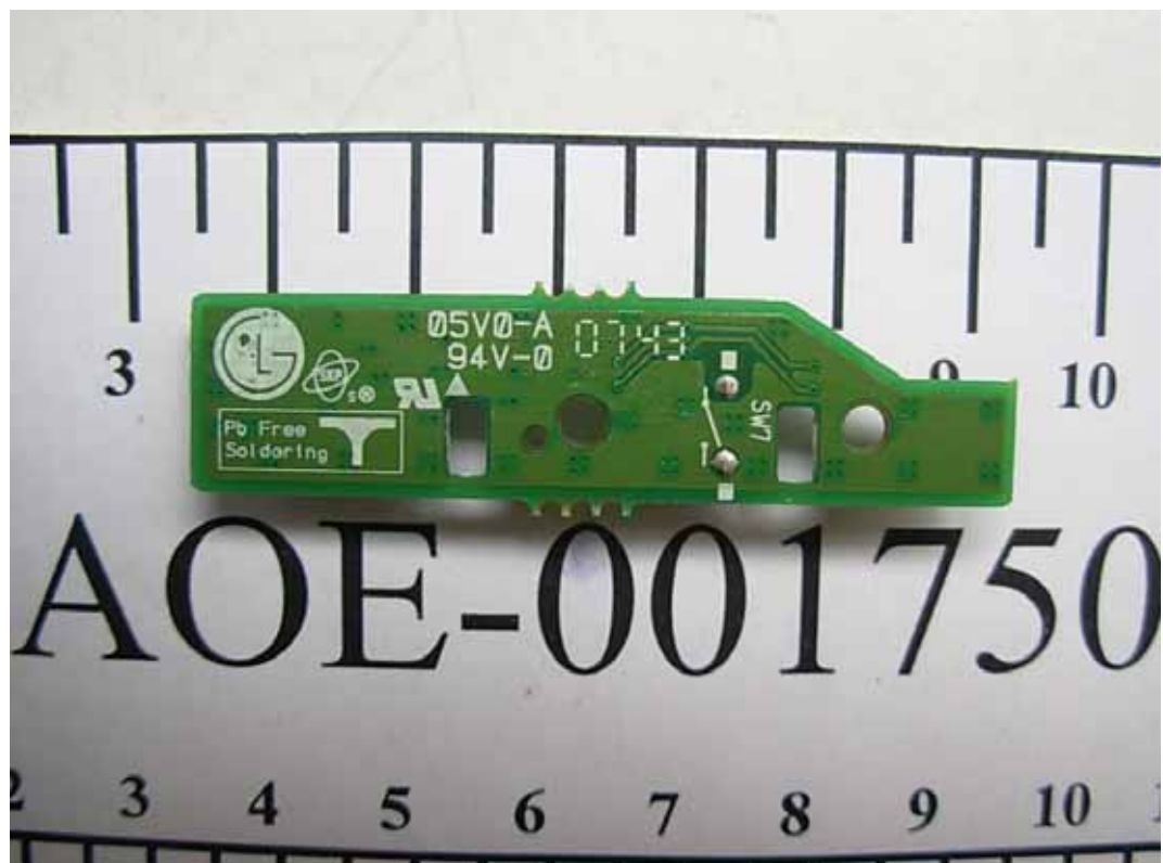
FIGURE 6 LCD MONITOR (M/N: W2252VQT) LED BOARD (SOLDERED SIDE)
